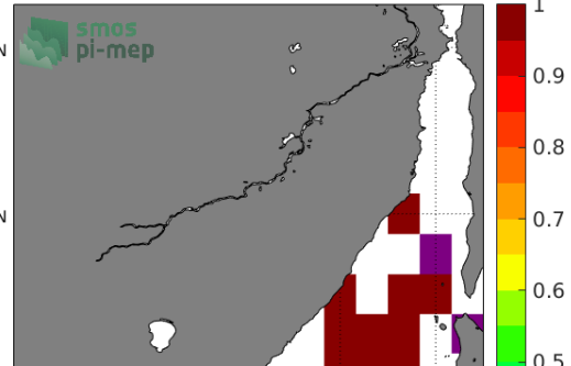
Temporal STD of (Sat - Argo) in 1°x1° boxes over 2013-2020
