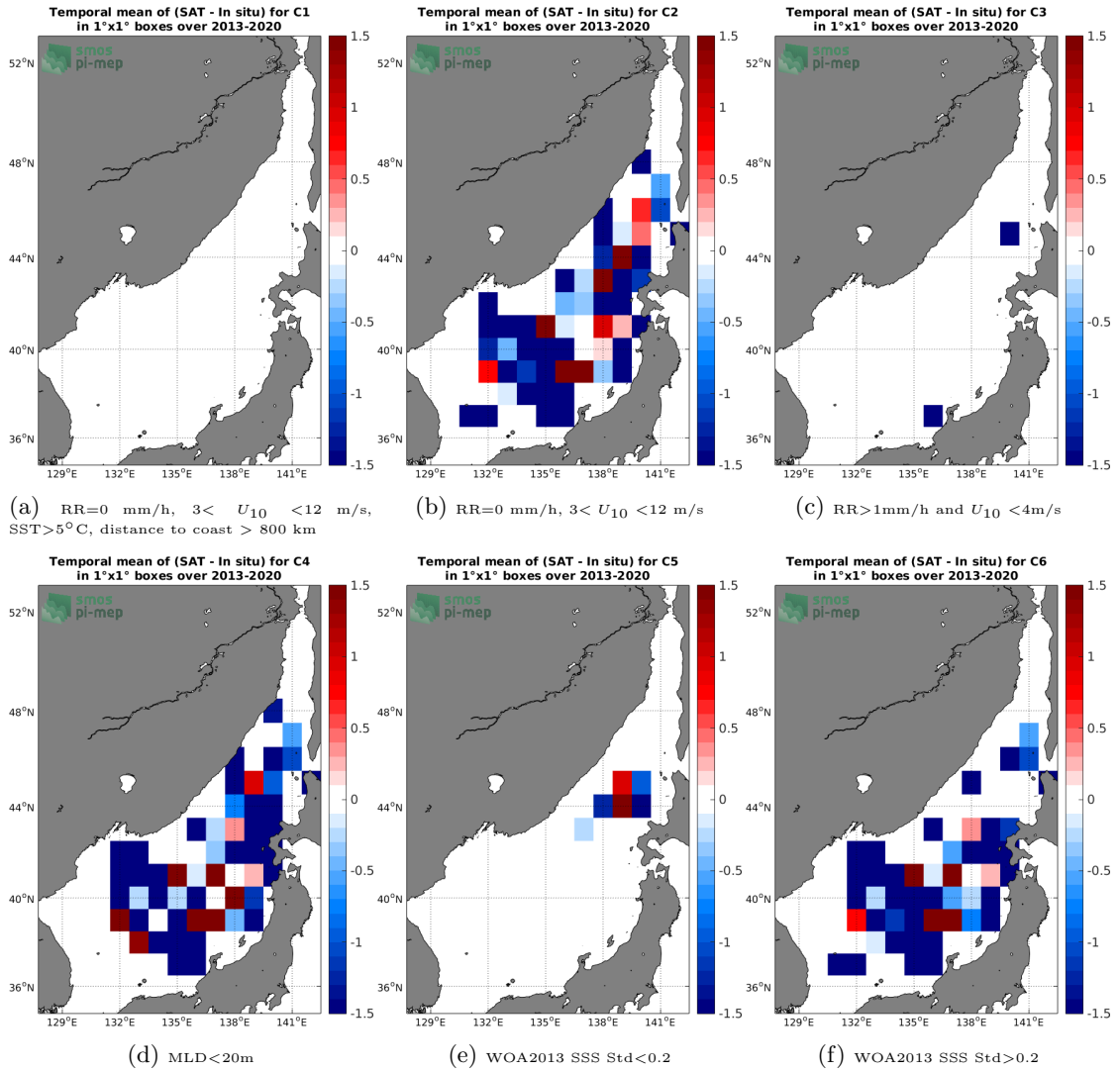
Figure 12: Temporal mean gridded over spatial boxes of size 1^\circ \times 1^\circ of \Delta\text{SSS} (SMOS L2 v662 (ESA) - Argo) for 6 different subdatasets corresponding to: RR=0 mm/h, 3 < U_{10} < 12 m/s, SST > 5^\circ\text{C} , distance to coast > 800 km (a), RR=0 mm/h, 3 < U_{10} < 12 m/s (b), RR > 1\text{mm/h} and U_{10} < 4\text{m/s} (c), MLD < 20\text{m} (d), WOA2013 SSS Std < 0.2 (e), WOA2013 SSS Std > 0.2 (f).
