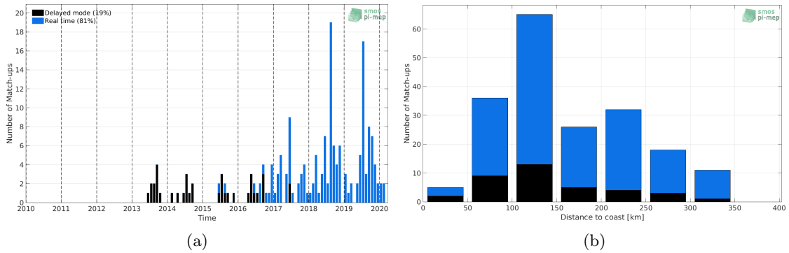
Figure 1: Number of match-ups between Argo and SMOS L2 v662 (ESA) SSS as a function of time (a) and as function of the distance to coast (b) over the Sea of Japan Pi-MEP region and for the full satellite product period.
