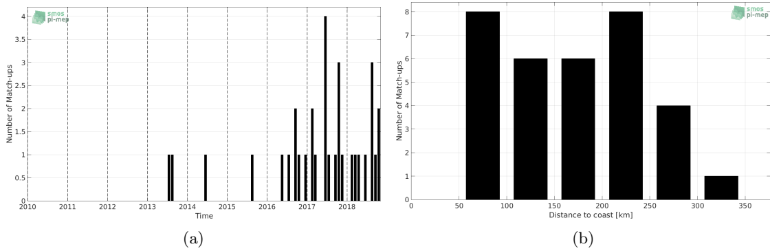
Figure 1: Number of match-ups between Argo and SMOS-L2-DPGS-v662 SSS as a function of time (a) and as function of the distance to coast (b) over the Sea of Japan Pi-MEP region and for the full satellite product period.
