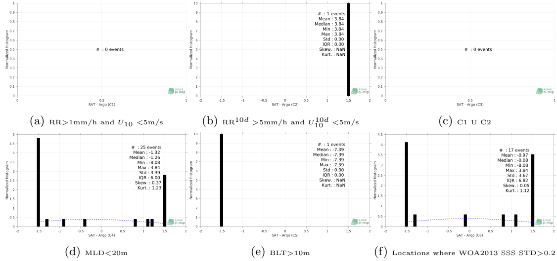
Figure 13: Normalized histogram of \Delta\text{SSS} (SMOS-L2-DPGS-v662 - Argo) for 6 different sub-datasets corresponding to: RR>1mm/h and U_{10} < 5\text{m/s} (a), \text{RR}^{10d} > 5\text{mm/h} and U_{10}^{10d} < 5\text{m/s} (b), C1 U C2 (c), MLD<20m (d), BLT>10m (e), Locations where WOA2013 SSS STD>0.2 (f).
