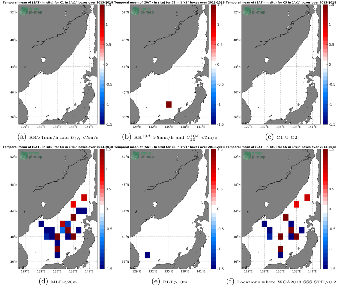
Figure 12: Temporal mean gridded over spatial boxes of size 1^\circ \times 1^\circ of \Delta SSS (SMOS-L2-DPGS-v662 - Argo) for 6 different subdatasets corresponding to: RR > 1\text{mm/h} and U_{10} < 5\text{m/s} (a), RR^{10d} > 5\text{mm/h} and U_{10}^{10d} < 5\text{m/s} (b), C1 U C2 (c), MLD < 20\text{m} (d), BLT > 10\text{m} (e), Locations where WOA2013 SSS STD > 0.2 (f).
