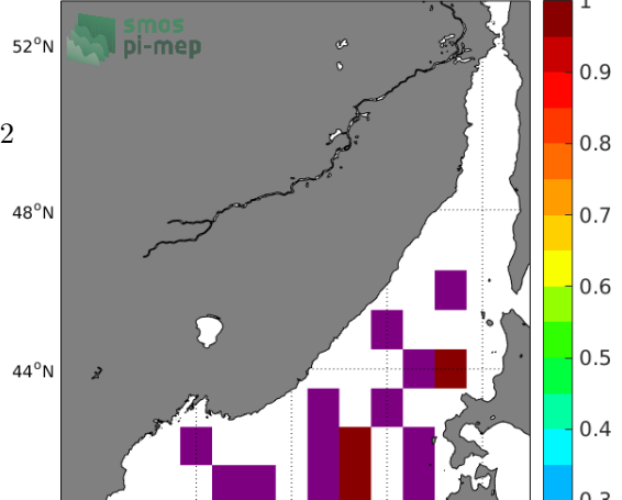
Temporal STD of (Sat-Argo) in 1°x1° boxes over 2013-2018
