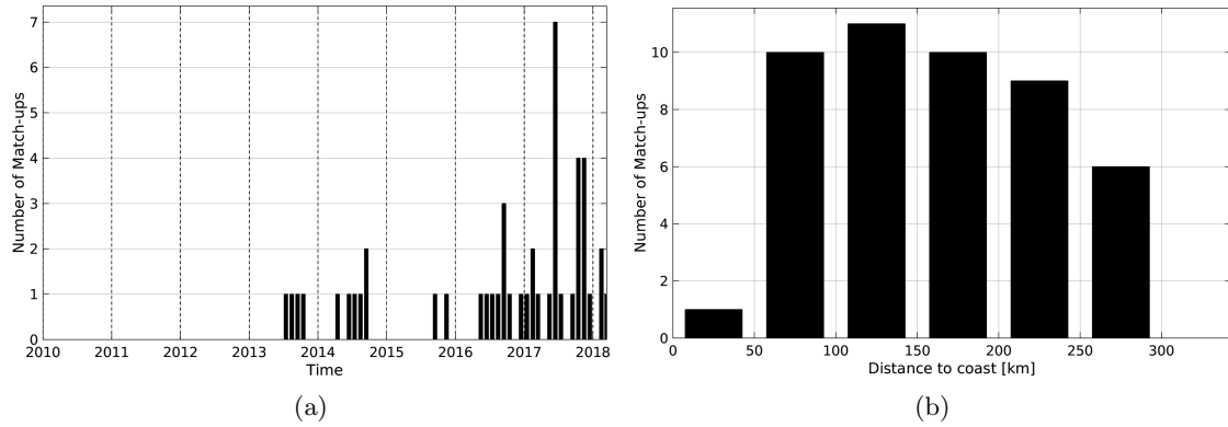
Figure 1: Number of match-ups between Argo and SMOS-L2-DPGS-v662 SSS as a function of time (a) and as function of the distance to coast (b) over the Sea of Japan Pi-MEP region and for the full satellite product period.
