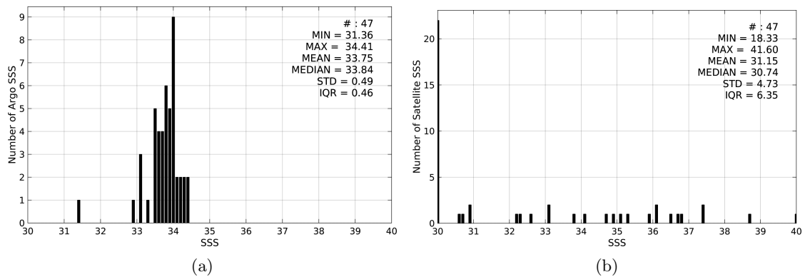
Figure 2: Histograms of SSS from Argo (a) and SMOS-L2-DPGS-v662 (b) considering all match-up pairs per bins of 0.1 over the Sea of Japan Pi-MEP region and for the full satellite product period.
