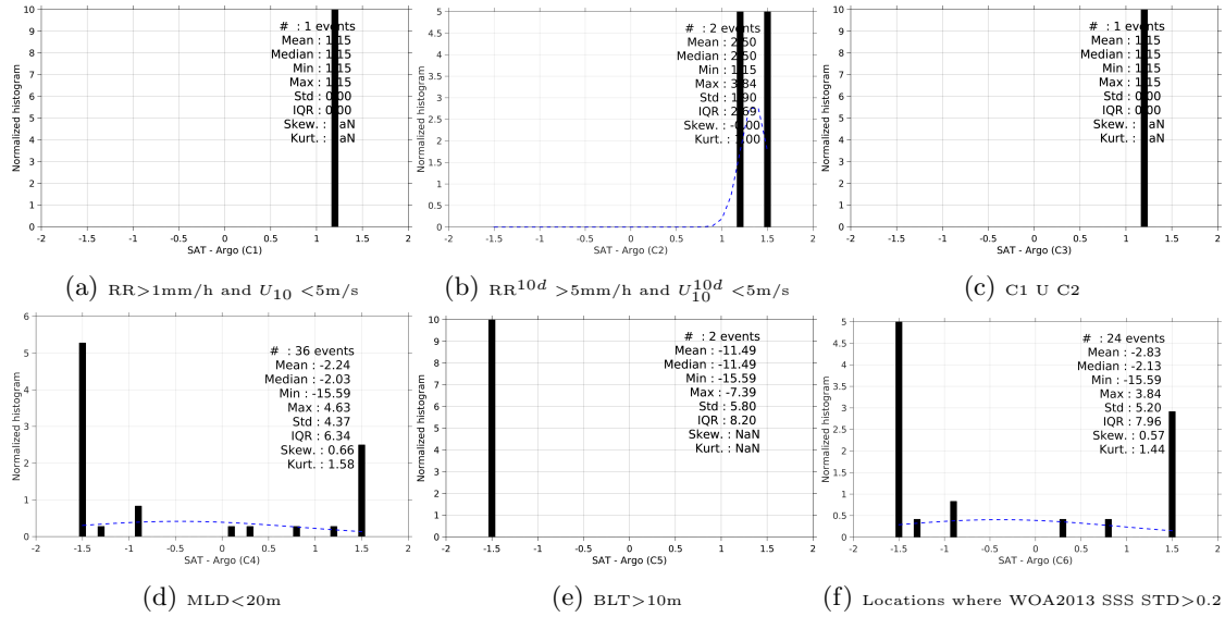
Figure 13: Normalized histogram of \Delta SSS (SMOS-L2-DPGS-v662 - Argo) for 6 different sub-datasets corresponding to: RR>1mm/h and U_{10} < 5 m/s (a), RR 10d >5mm/h and U_{10}^{10d} < 5 m/s (b), C1 U C2 (c),MLD<20m (d),BLT>10m (e),Locations where WOA2013 SSS STD>0.2 (f).
