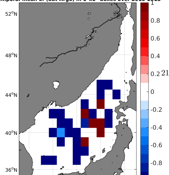
Temporal mean of (Sat-Argo) in 1°x1° boxes over 2013-2018 Temporal STD of (Sat-Argo) in 1°x1° boxes over 2013-2018
