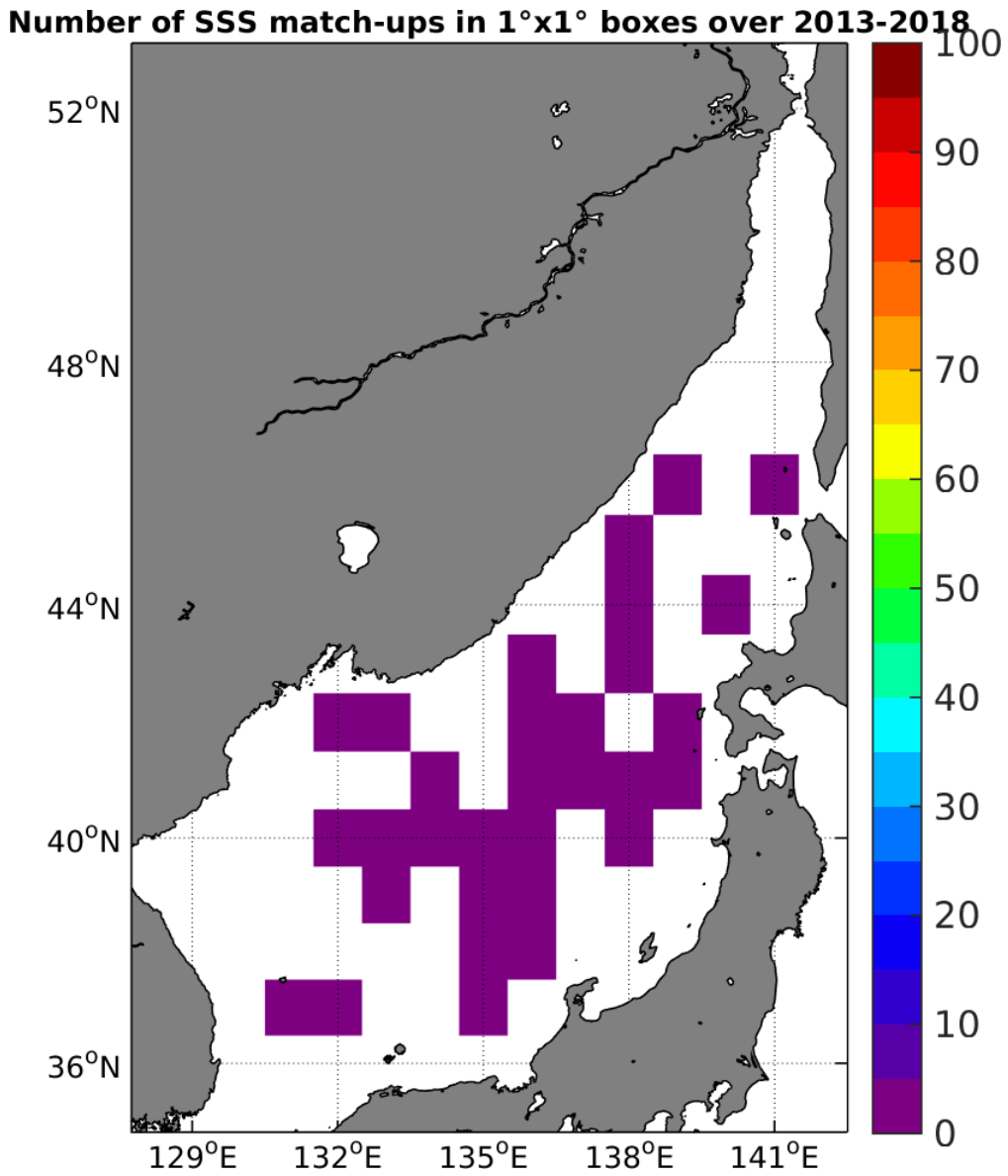
Figure 4: Number of SSS match-ups between Argo SSS and the SMOS-L2-DPGS-v662 SSS product for the Sea of Japan Pi-MEP region over 1°x1° boxes and for the full satellite product period.
