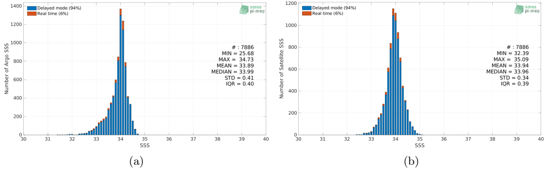
Figure 2: Histograms of SSS from Argo (a) and SMAP SSS L4 OI v1 - 7 Days (IPRC) (b) considering all match-up pairs per bins of 0.1 over the Sea of Japan Pi-MEP region and for the full satellite product period.
