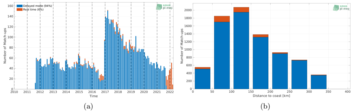
Figure 1: Number of match-ups between Argo and SMAP SSS L4 OI v1 - 7 Days (IPRC) SSS as a function of time (a) and as function of the distance to coast (b) over the Sea of Japan Pi-MEP region and for the full satellite product period.
