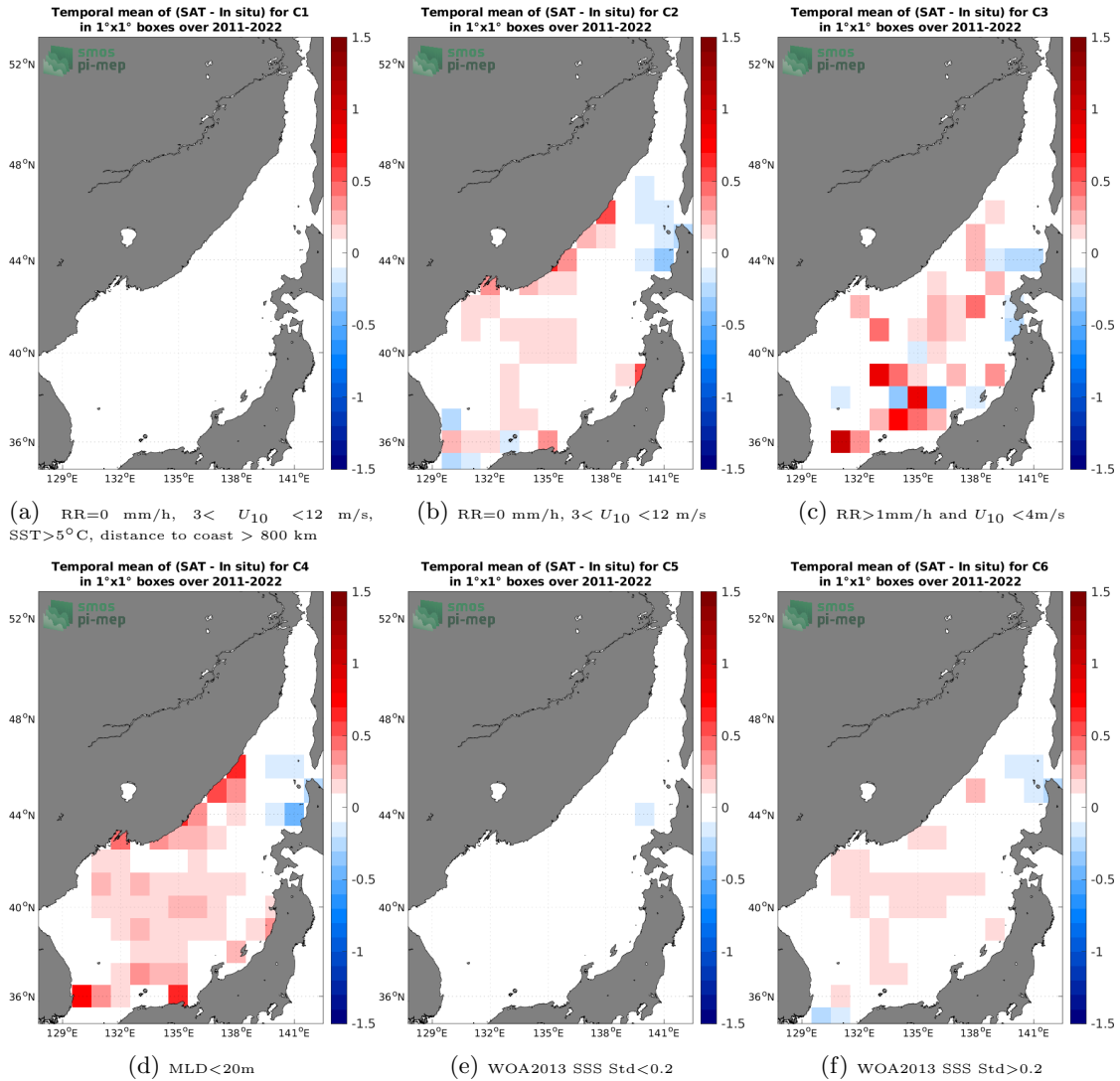
Figure 12: Temporal mean gridded over spatial boxes of size 1^\circ \times 1^\circ of \Delta SSS (SMAP SSS L4 OI v1 - 7 Days (IPRC) - Argo) for 6 different subdatasets corresponding to:RR=0 mm/h, 3 < U_{10} < 12 m/s, SST>5°C, distance to coast > 800 km (a), RR=0 mm/h, 3 < U_{10} < 12 m/s (b), RR>1mm/h and U_{10} < 4 m/s (c),MLD<20m (d),WOA2013 SSS Std<0.2 (e),WOA2013 SSS Std>0.2 (f).
