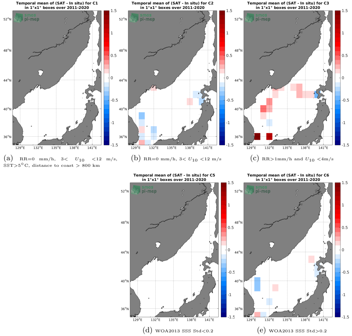
Figure 12: Temporal mean gridded over spatial boxes of size 1^\circ \times 1^\circ of \Delta SSS (SMAP SSS L4 OI v1 - Monthly (IPRC) - TSG (LEGOS-DM)) for 5 different subdatasets corresponding to:RR=0 mm/h, 3 < U_{10} < 12 m/s, SST>5°C, distance to coast > 800 km (a), RR=0 mm/h, 3 < U_{10} < 12 m/s (b), RR>1mm/h and U_{10} < 4 m/s (c), WOA2013 SSS Std<0.2 (d), WOA2013 SSS Std>0.2 (e).
