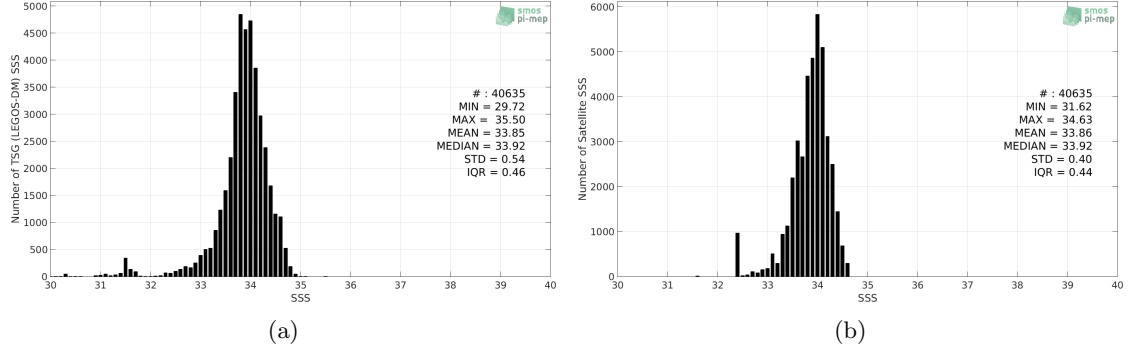
Figure 2: Histograms of SSS from TSG (LEGOS-DM) (a) and SMAP SSS L4 OI v1 - Monthly (IPRC) (b) considering all match-up pairs per bins of 0.1 over the Sea of Japan Pi-MEP region and for the full satellite product period.
