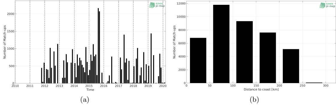
Figure 1: Number of match-ups between TSG (LEGOS-DM) and SMAP SSS L4 OI v1 - Monthly (IPRC) SSS as a function of time (a) and as function of the distance to coast (b) over the Sea of Japan Pi-MEP region and for the full satellite product period.
