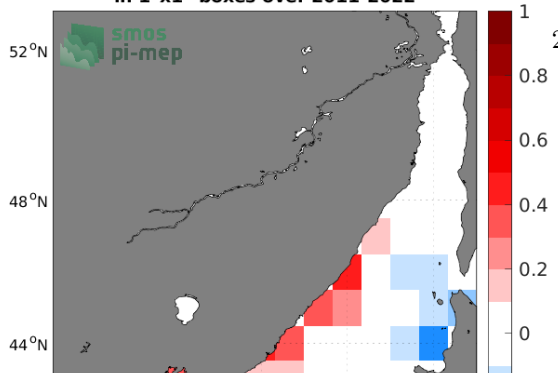
Temporal mean of (Sat - Argo) in 1°x1° boxes over 2011-2022
