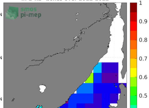
Temporal STD of (Sat - Argo) in 1°x1° boxes over 2011-2022
