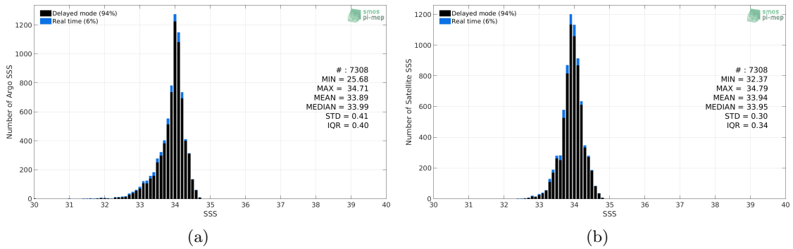
Figure 2: Histograms of SSS from Argo (a) and SMAP SSS L4 OI v1 - Monthly (IPRC) (b) considering all match-up pairs per bins of 0.1 over the Sea of Japan Pi-MEP region and for the full satellite product period.
