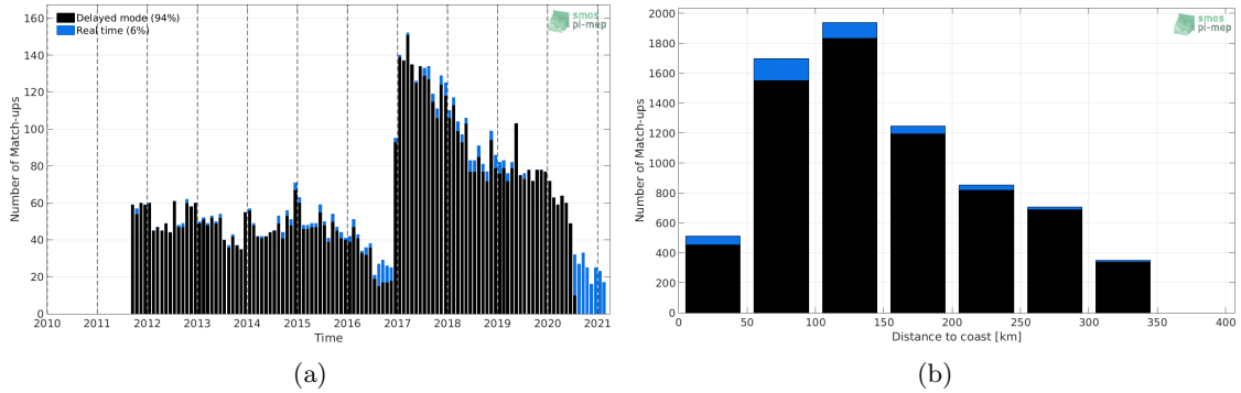
Figure 1: Number of match-ups between Argo and SMAP SSS L4 OI v1 - Monthly (IPRC) SSS as a function of time (a) and as function of the distance to coast (b) over the Sea of Japan Pi-MEP region and for the full satellite product period.
