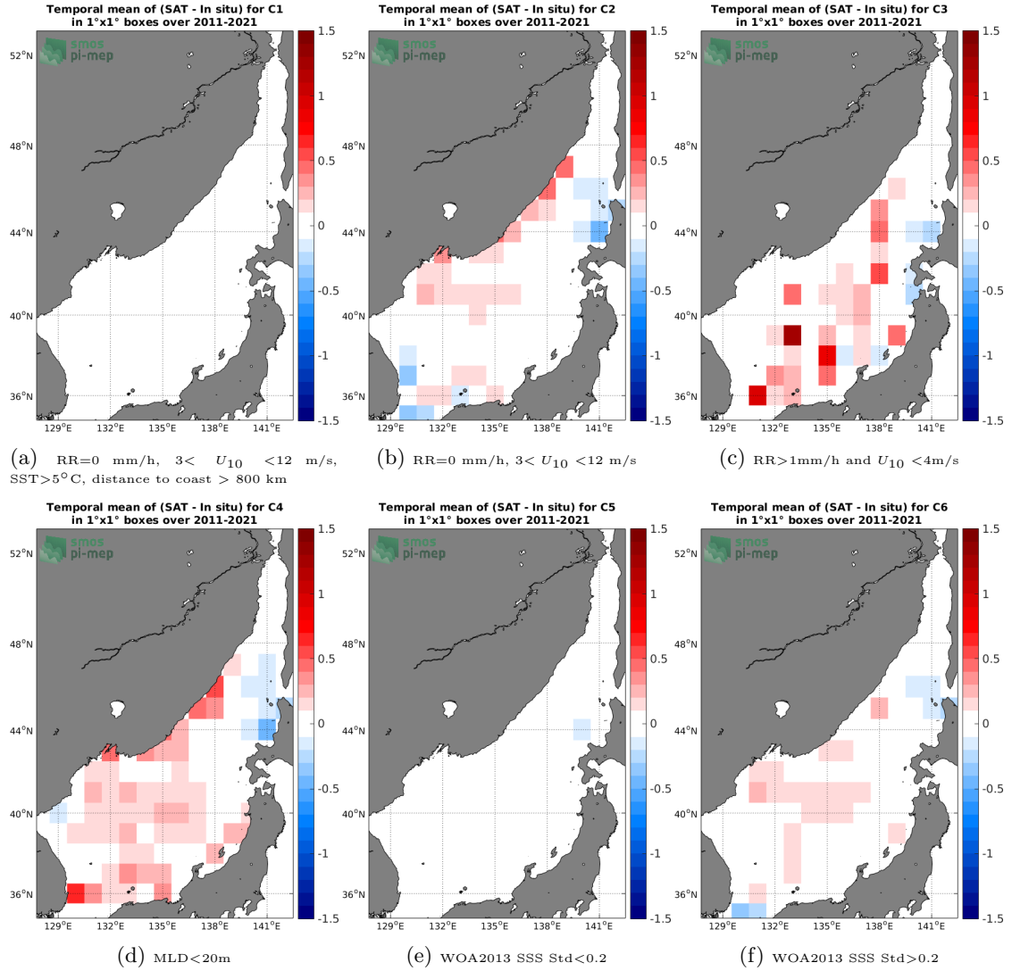
Figure 12: Temporal mean gridded over spatial boxes of size 1^\circ \times 1^\circ of \Delta SSS (SMAP SSS L4 OI v1 - Monthly (IPRC) - Argo) for 6 different subdatasets corresponding to: RR=0 mm/h, 3 < U_{10} < 12 m/s, SST > 5^\circ\text{C} , distance to coast > 800 km (a), RR=0 mm/h, 3 < U_{10} < 12 m/s (b), RR > 1 mm/h and U_{10} < 4 m/s (c), MLD < 20 m (d), WOA2013 SSS Std < 0.2 (e), WOA2013 SSS Std > 0.2 (f).
