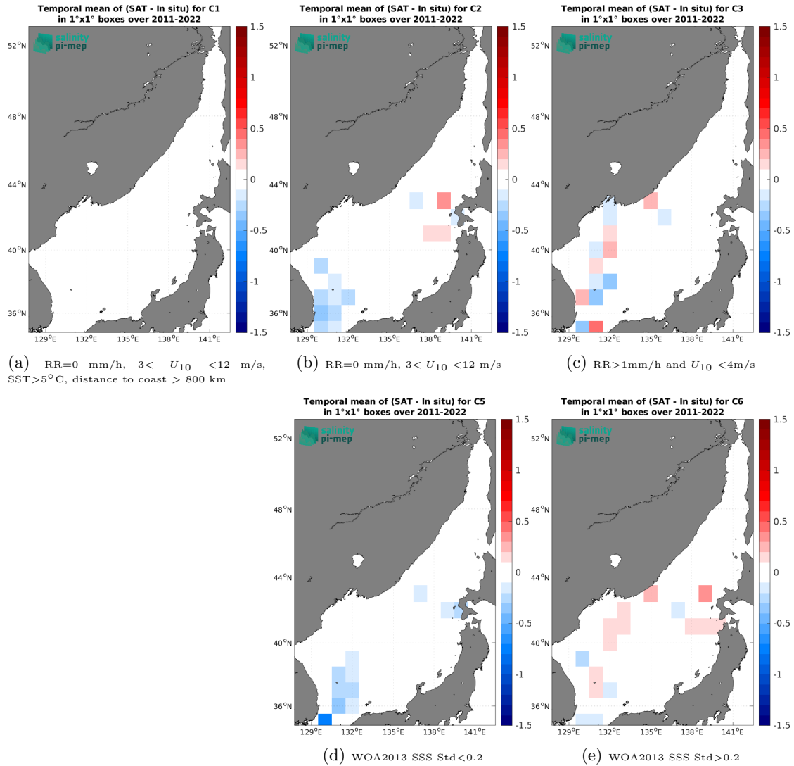
Figure 14: Temporal mean gridded over spatial boxes of size 1^\circ \times 1^\circ of \Delta SSS (SMAP SSS L4 OI v3 - Monthly (ESR) - TSG (LEGOS-DM)) for 5 different subdatasets corresponding to: RR=0 mm/h, 3 < U_{10} < 12 m/s, SST>5°C, distance to coast > 800 km (a), RR=0 mm/h, 3 < U_{10} < 12 m/s (b), RR>1mm/h and U_{10} < 4 m/s (c), WOA2013 SSS Std<0.2 (d), WOA2013 SSS Std>0.2 (e).
