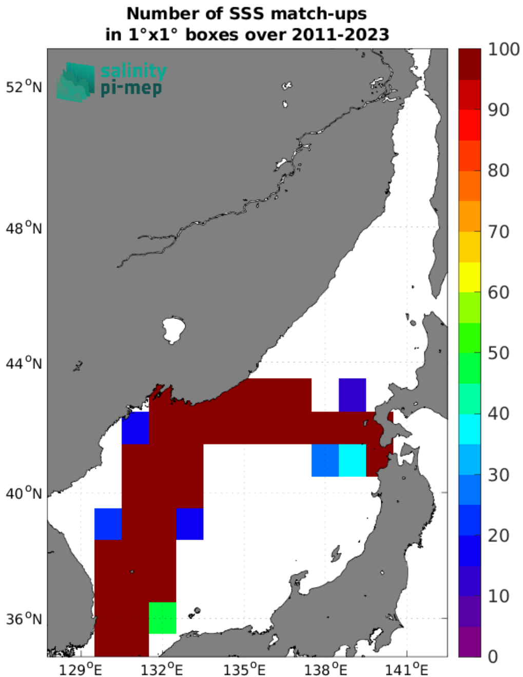
Figure 5: Number of SSS match-ups between TSG (LEGOS-DM) SSS and the SMAP SSS L4 OI v3 - Daily (ESR) SSS product for the Sea of Japan Pi-MEP region over 1°x1° boxes and for the full satellite product period.
