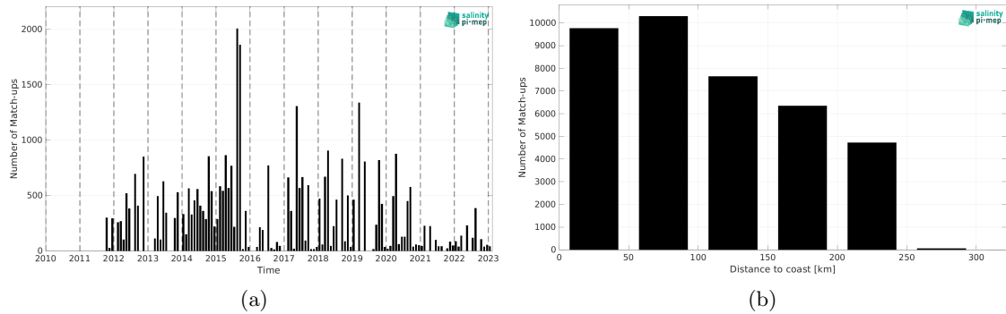
Figure 2: Number of match-ups between TSG (LEGOS-DM) and SMAP SSS L4 OI v3 - Daily (ESR) SSS as a function of time (a) and as function of the distance to coast (b) over the Sea of Japan Pi-MEP region and for the full satellite product period.
