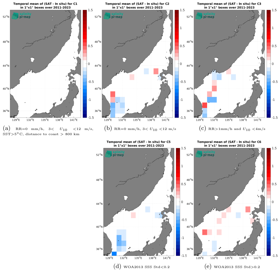
Figure 14: Temporal mean gridded over spatial boxes of size 1^\circ \times 1^\circ of \Delta SSS (SMAP SSS L4 OI v3 - Daily (ESR) - TSG (LEGOS-DM)) for 5 different subdatasets corresponding to:RR=0 mm/h, 3 < U_{10} < 12 m/s, SST>5°C, distance to coast > 800 km (a), RR=0 mm/h, 3 < U_{10} < 12 m/s (b), RR>1mm/h and U_{10} < 4 m/s (c), WOA2013 SSS Std<0.2 (d), WOA2013 SSS Std>0.2 (e).
