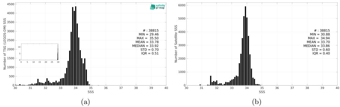
Figure 3: Histograms of SSS from TSG (LEGOS-DM) (a) and SMAP SSS L4 OI v3 - Daily (ESR) (b) considering all match-up pairs per bins of 0.1 over the Sea of Japan Pi-MEP region and for the full satellite product period.
