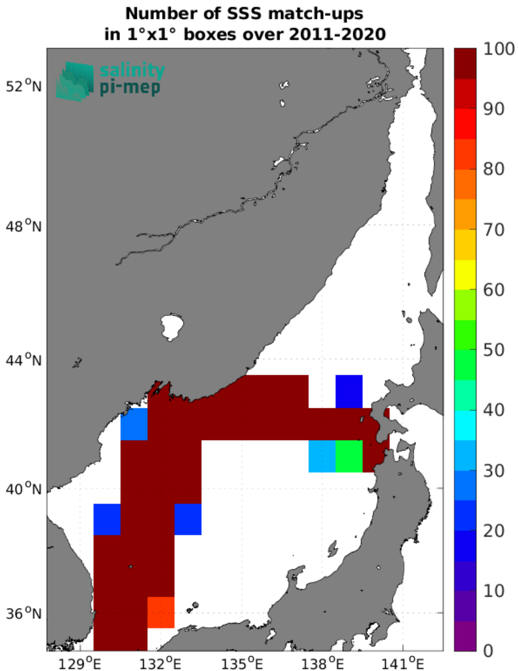
Figure 4: Number of SSS match-ups between TSG (LEGOS-DM) SSS and the SMAP SSS L4 OI v2 - 7 Days (ESR) SSS product for the Sea of Japan Pi-MEP region over 1°x1° boxes and for the full satellite product period.
