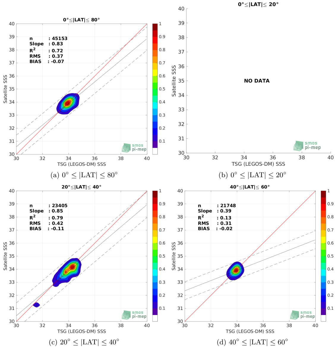
Figure 9: Contour maps of the concentration of SMAP SSS L4 OI v2 - 7 Days (ESR) SSS (y-axis) versus TSG (LEGOS-DM) SSS (x-axis) at match-up pairs for different latitude bands. For each plot, the red line shows x=y . The black thin and dashed lines indicate a linear fit through the data cloud and the \pm 95\% confidence levels, respectively. The number match-up pairs n , the slope and R^2 coefficient of the linear fit, the root mean square (RMS) and the mean bias between satellite and in situ data are indicated for each latitude band in each plots.
