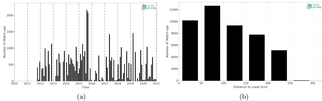
Figure 1: Number of match-ups between TSG (LEGOS-DM) and SMAP SSS L4 OI v2 - 7 Days (ESR) SSS as a function of time (a) and as function of the distance to coast (b) over the Sea of Japan Pi-MEP region and for the full satellite product period.
