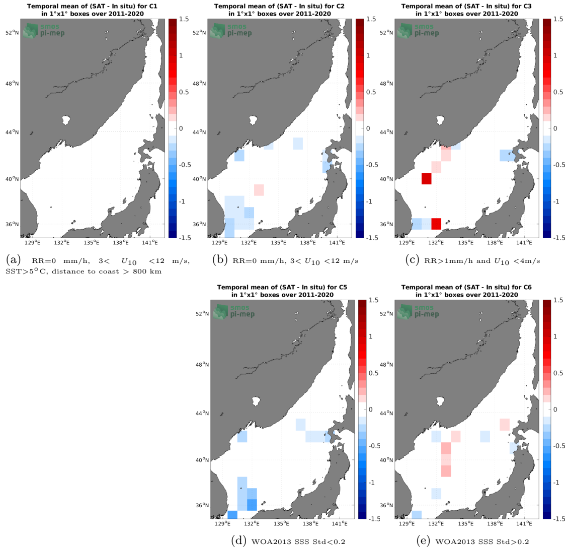
Figure 12: Temporal mean gridded over spatial boxes of size 1^\circ \times 1^\circ of \Delta\text{SSS} (SMAP SSS L4 OI v2 - 7 Days (ESR) - TSG (LEGOS-DM)) for 5 different subdatasets corresponding to: RR=0 mm/h, 3 < U_{10} < 12 m/s, SST > 5^\circ\text{C} , distance to coast > 800 km (a), RR=0 mm/h, 3 < U_{10} < 12 m/s (b), RR > 1\text{mm/h} and U_{10} < 4\text{m/s} (c), WOA2013 SSS Std < 0.2 (d), WOA2013 SSS Std > 0.2 (e).
