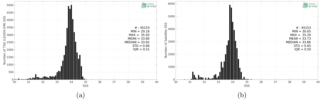
Figure 2: Histograms of SSS from TSG (LEGOS-DM) (a) and SMAP SSS L4 OI v2 - 7 Days (ESR) (b) considering all match-up pairs per bins of 0.1 over the Sea of Japan Pi-MEP region and for the full satellite product period.
