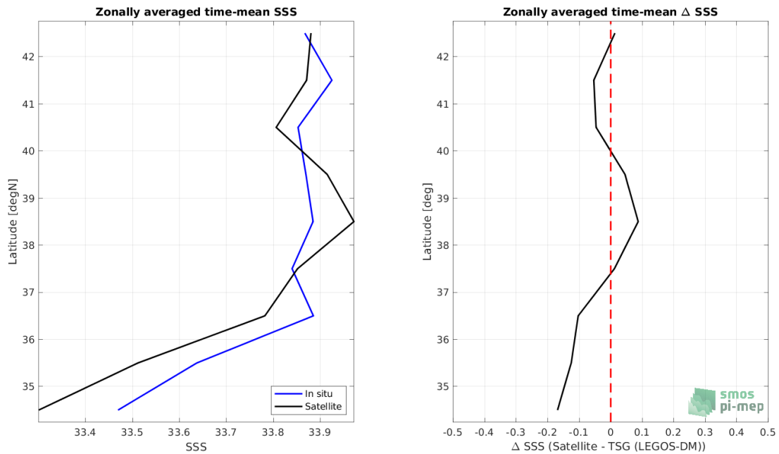
Figure 8: Left panel: Zonal mean SSS from SMAP SSS L4 OI v2 - 7 Days (ESR) satellite product (black) and from TSG (LEGOS-DM) (blue). Right panel: Zonal mean of \Delta SSS (Satellite - TSG (LEGOS-DM)) for all the collected Pi-MEP match-up pairs estimated over the full satellite product period.
