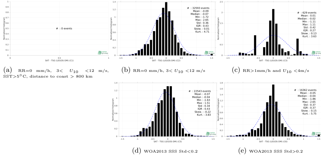
Figure 13: Normalized histogram of \Delta SSS (SMAP SSS L4 OI v2 - 7 Days (ESR) - TSG (LEGOS-DM)) for 5 different subdatasets corresponding to: RR=0 mm/h, 3 < U_{10} < 12 m/s, SST > 5°C, distance to coast > 800 km (a), RR=0 mm/h, 3 < U_{10} < 12 m/s (b), RR > 1mm/h and U_{10} < 4 m/s (c), WOA2013 SSS Std < 0.2 (d), WOA2013 SSS Std > 0.2 (e).
