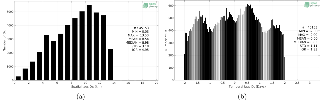
Figure 5: Histograms of the spatial (a) and temporal (b) lags between the location/time of the TSG (LEGOS-DM) measurement and the date of the corresponding SMAP SSS L4 OI v2 - 7 Days (ESR) SSS pixel.
