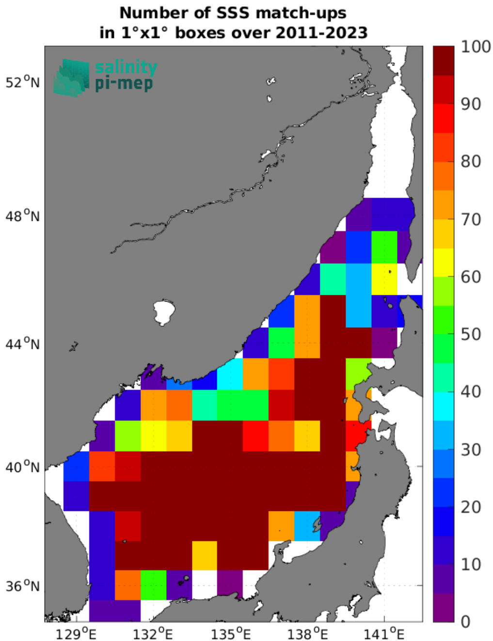
Figure 4: Number of SSS match-ups between Argo SSS and the SMAP SSS L4 OI v2 - 7 Days (ESR) SSS product for the Sea of Japan Pi-MEP region over 1°x1° boxes and for the full satellite product period.
