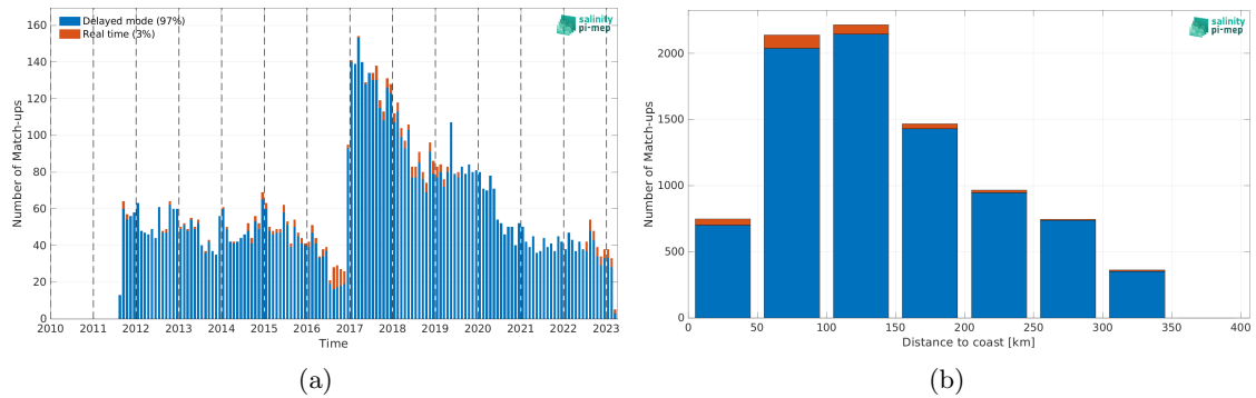
Figure 1: Number of match-ups between Argo and SMAP SSS L4 OI v2 - 7 Days (ESR) SSS as a function of time (a) and as function of the distance to coast (b) over the Sea of Japan Pi-MEP region and for the full satellite product period.
