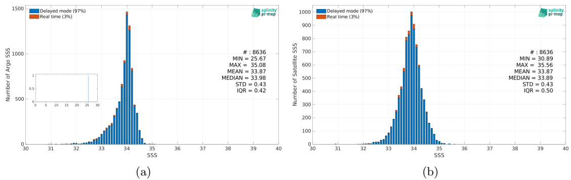
Figure 2: Histograms of SSS from Argo (a) and SMAP SSS L4 OI v2 - 7 Days (ESR) (b) considering all match-up pairs per bins of 0.1 over the Sea of Japan Pi-MEP region and for the full satellite product period.
