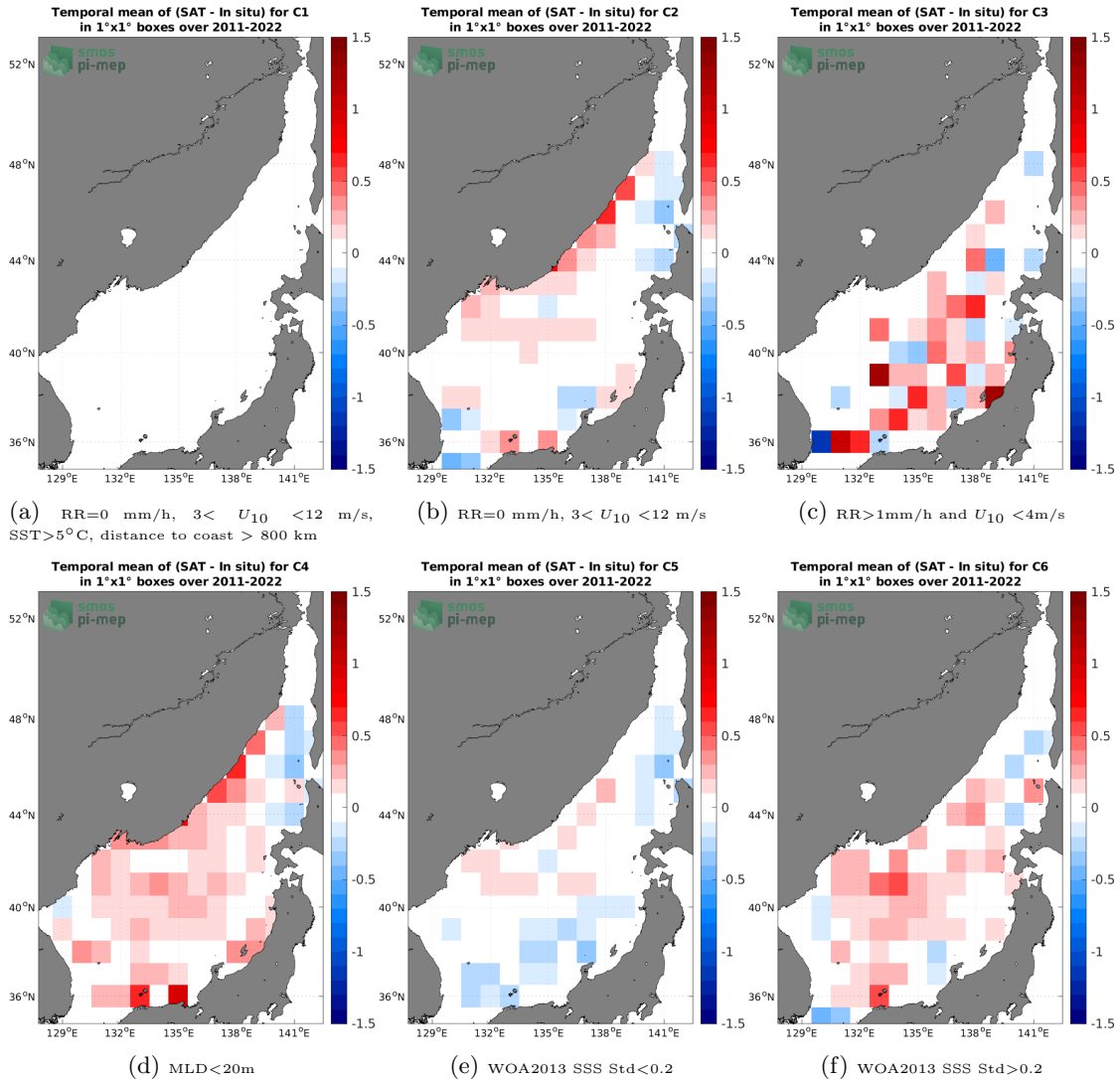
Figure 12: Temporal mean gridded over spatial boxes of size 1^\circ \times 1^\circ of \Delta SSS (SMAP SSS L4 OI v2 - 7 Days (ESR) - Argo) for 6 different subdatasets corresponding to: RR=0 mm/h, 3 < U_{10} < 12 m/s, SST > 5^\circ\text{C} , distance to coast > 800 km (a), RR=0 mm/h, 3 < U_{10} < 12 m/s (b), RR > 1 mm/h and U_{10} < 4 m/s (c), MLD < 20 m (d), WOA2013 SSS Std < 0.2 (e), WOA2013 SSS Std > 0.2 (f).
