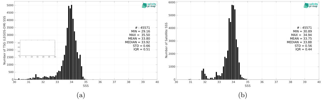
Figure 2: Histograms of SSS from TSG (LEGOS-DM) (a) and SMAP SSS L4 OI v2 - Monthly (IPRC) (b) considering all match-up pairs per bins of 0.1 over the Sea of Japan Pi-MEP region and for the full satellite product period.
