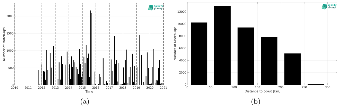
Figure 1: Number of match-ups between TSG (LEGOS-DM) and SMAP SSS L4 OI v2 - Monthly (IPRC) SSS as a function of time (a) and as function of the distance to coast (b) over the Sea of Japan Pi-MEP region and for the full satellite product period.
