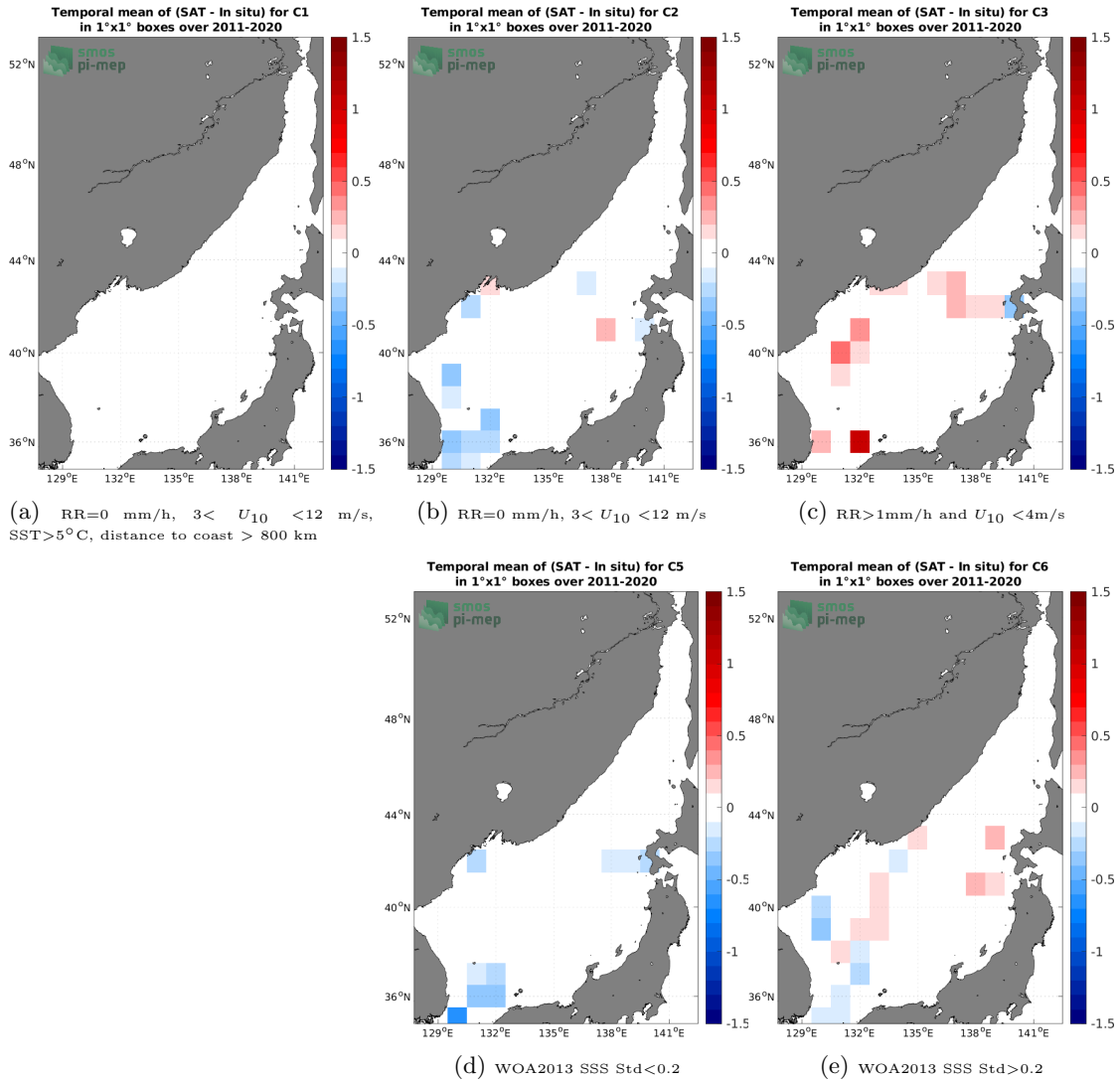
Figure 12: Temporal mean gridded over spatial boxes of size 1^\circ \times 1^\circ of \Delta\text{SSS} (SMAP SSS L4 OI v2 - Monthly (IPRC) - TSG (LEGOS-DM)) for 5 different subdatasets corresponding to: RR=0 mm/h, 3 < U_{10} < 12 m/s, SST > 5^\circ\text{C} , distance to coast > 800 km (a), RR=0 mm/h, 3 < U_{10} < 12 m/s (b), RR > 1\text{mm/h} and U_{10} < 4\text{m/s} (c), WOA2013 SSS Std < 0.2 (d), WOA2013 SSS Std > 0.2 (e).
