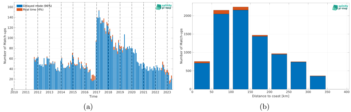
Figure 1: Number of match-ups between Argo and SMAP SSS L4 OI v2 - Monthly (IPRC) SSS as a function of time (a) and as function of the distance to coast (b) over the Sea of Japan Pi-MEP region and for the full satellite product period.
