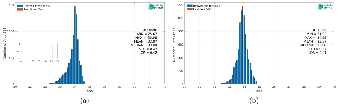
Figure 2: Histograms of SSS from Argo (a) and SMAP SSS L4 OI v2 - Monthly (IPRC) (b) considering all match-up pairs per bins of 0.1 over the Sea of Japan Pi-MEP region and for the full satellite product period.
