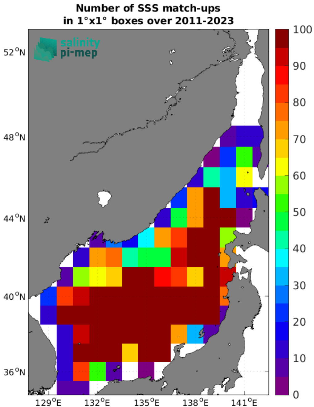
Figure 4: Number of SSS match-ups between Argo SSS and the SMAP SSS L4 OI v2 - Monthly (IPRC) SSS product for the Sea of Japan Pi-MEP region over 1°x1° boxes and for the full satellite product period.
