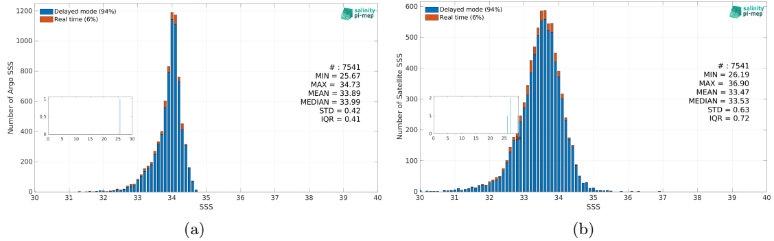
Figure 3: Histograms of SSS from Argo (a) and SMAP SSS L3 v5.3 - 8-Day running (RSS) (b) considering all match-up pairs per bins of 0.1 over the Sea of Japan Pi-MEP region and for the full satellite product period.
