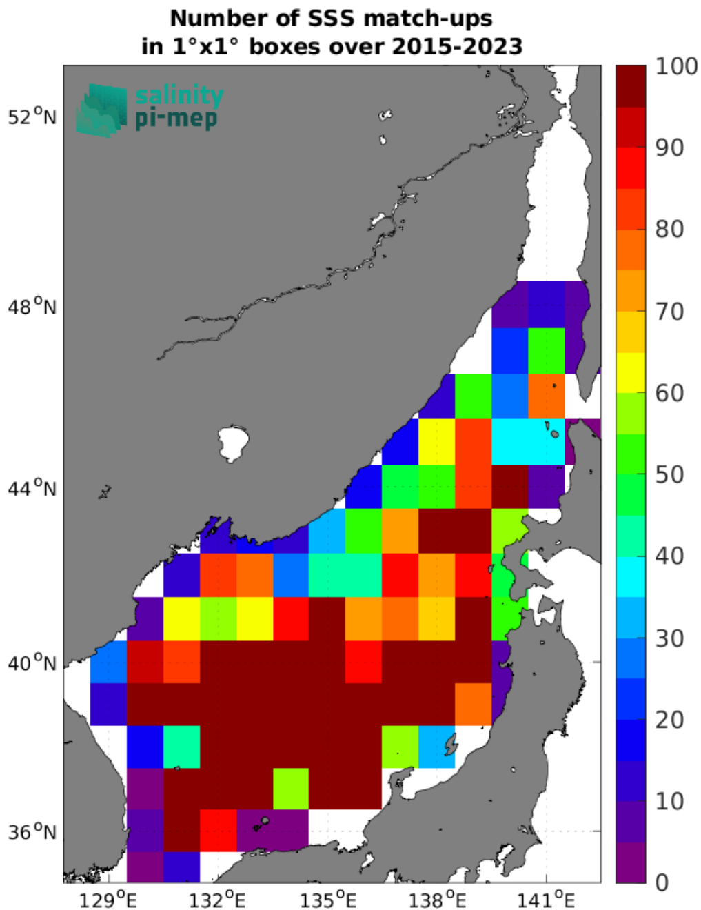
Figure 5: Number of SSS match-ups between Argo SSS and the SMAP SSS L3 v5.3 - 8-Day running (RSS) SSS product for the Sea of Japan Pi-MEP region over 1°x1° boxes and for the full satellite product period.
