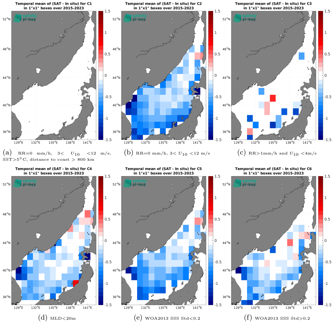
Figure 14: Temporal mean gridded over spatial boxes of size 1^\circ \times 1^\circ of \Delta\text{SSS} (SMAP SSS L3 v5.3 - 8-Day running (RSS) - Argo) for 6 different subdatasets corresponding to: RR=0 mm/h, 3 < U_{10} < 12 m/s, SST > 5^\circ\text{C} , distance to coast > 800 km (a), RR=0 mm/h, 3 < U_{10} < 12 m/s (b), RR > 1 mm/h and U_{10} < 4 m/s (c), MLD < 20 m (d), WOA2013 SSS Std < 0.2 (e), WOA2013 SSS Std > 0.2 (f).
