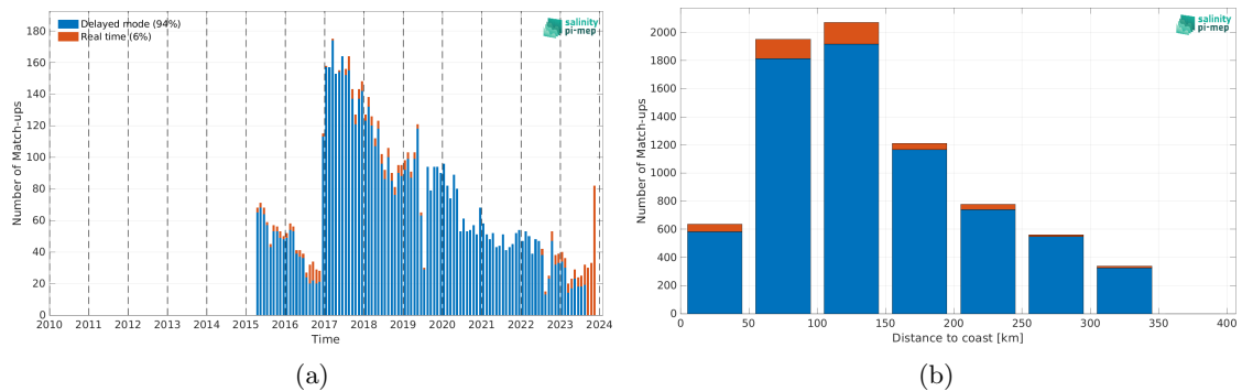
Figure 2: Number of match-ups between Argo and SMAP SSS L3 v5.3 - 8-Day running (RSS) SSS as a function of time (a) and as function of the distance to coast (b) over the Sea of Japan Pi-MEP region and for the full satellite product period.
