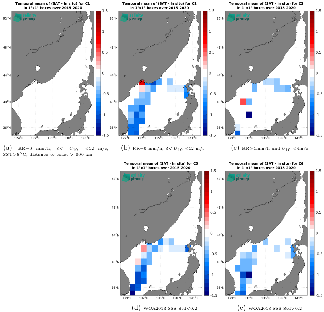
Figure 12: Temporal mean gridded over spatial boxes of size 1^\circ \times 1^\circ of \Delta\text{SSS} (SMAP SSS L3 v5 - 8-Day running (RSS) - TSG (LEGOS-DM)) for 5 different subdatasets corresponding to: RR=0 mm/h, 3 < U_{10} < 12 m/s, SST > 5^\circ\text{C} , distance to coast > 800 km (a), RR=0 mm/h, 3 < U_{10} < 12 m/s (b), RR > 1 mm/h and U_{10} < 4 m/s (c), WOA2013 SSS Std < 0.2 (d), WOA2013 SSS Std > 0.2 (e).
