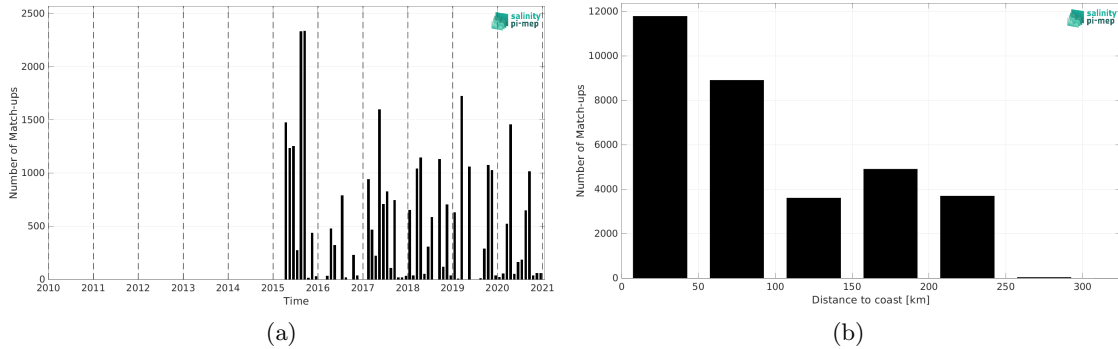
Figure 1: Number of match-ups between TSG (LEGOS-DM) and SMAP SSS L3 v5 - 8-Day running (RSS) SSS as a function of time (a) and as function of the distance to coast (b) over the Sea of Japan Pi-MEP region and for the full satellite product period.
