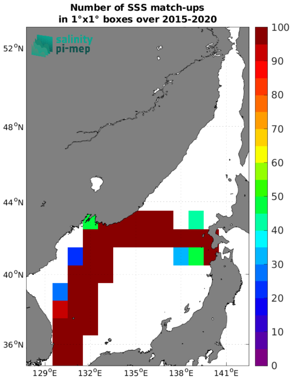
Figure 4: Number of SSS match-ups between TSG (LEGOS-DM) SSS and the SMAP SSS L3 v5 - 8-Day running (RSS) SSS product for the Sea of Japan Pi-MEP region over 1°x1° boxes and for the full satellite product period.
