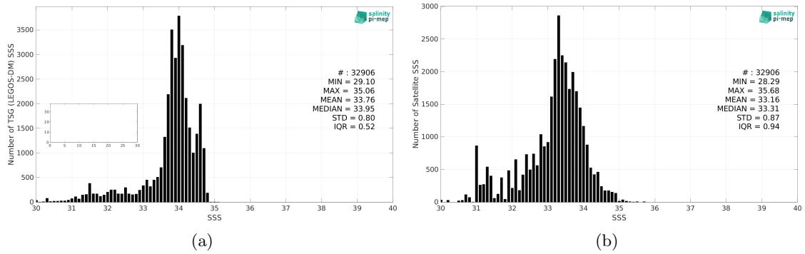
Figure 2: Histograms of SSS from TSG (LEGOS-DM) (a) and SMAP SSS L3 v5 - 8-Day running (RSS) (b) considering all match-up pairs per bins of 0.1 over the Sea of Japan Pi-MEP region and for the full satellite product period.
