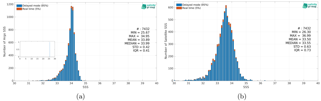
Figure 2: Histograms of SSS from Argo (a) and SMAP SSS L3 v5 - 8-Day running (RSS) (b) considering all match-up pairs per bins of 0.1 over the Sea of Japan Pi-MEP region and for the full satellite product period.
