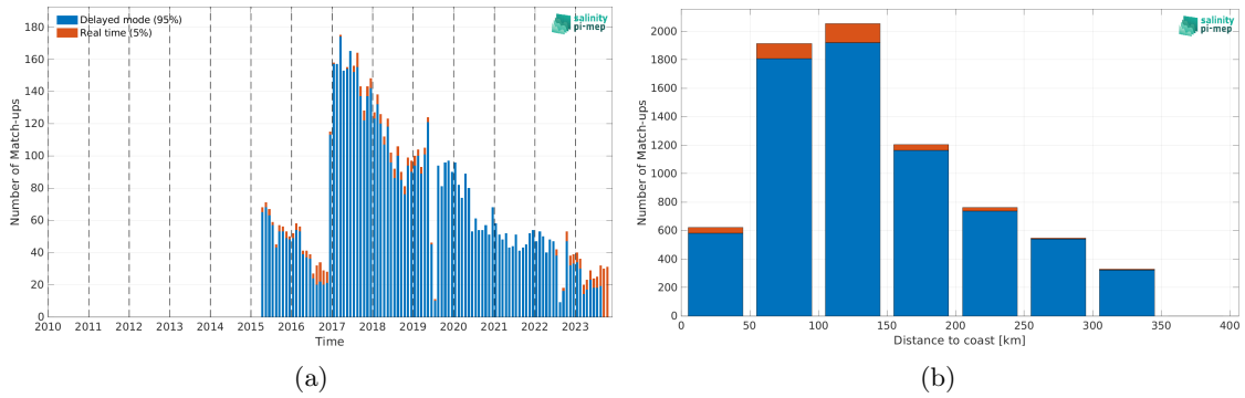
Figure 1: Number of match-ups between Argo and SMAP SSS L3 v5 - 8-Day running (RSS) SSS as a function of time (a) and as function of the distance to coast (b) over the Sea of Japan Pi-MEP region and for the full satellite product period.
