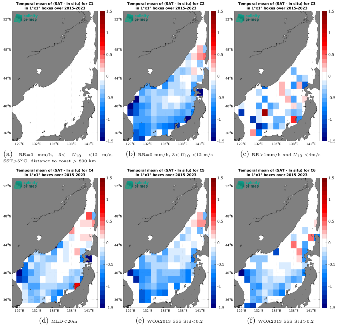
Figure 12: Temporal mean gridded over spatial boxes of size 1^\circ \times 1^\circ of \Delta SSS (SMAP SSS L3 v5 - 8-Day running (RSS) - Argo) for 6 different subdatasets corresponding to:RR=0 mm/h, 3 < U_{10} < 12 m/s, SST>5°C, distance to coast > 800 km (a), RR=0 mm/h, 3 < U_{10} < 12 m/s (b), RR>1mm/h and U_{10} < 4 m/s (c),MLD<20m (d),WOA2013 SSS Std<0.2 (e),WOA2013 SSS Std>0.2 (f).
