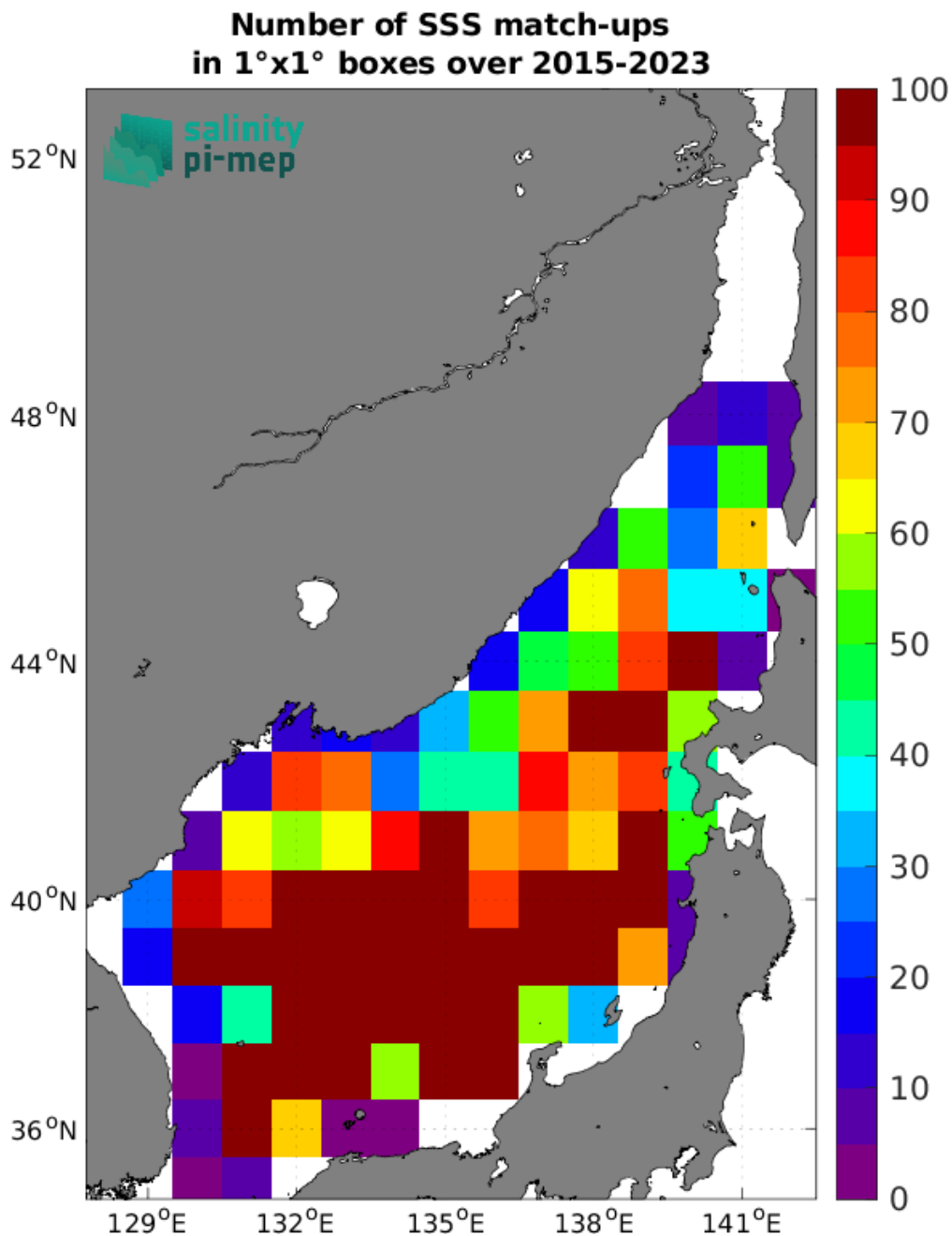
Figure 4: Number of SSS match-ups between Argo SSS and the SMAP SSS L3 v5 - 8-Day running (RSS) SSS product for the Sea of Japan Pi-MEP region over 1°x1° boxes and for the full satellite product period.
