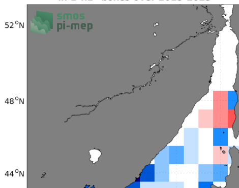
Temporal mean of (Sat - Argo) in 1°x1° boxes over 2015-2023
