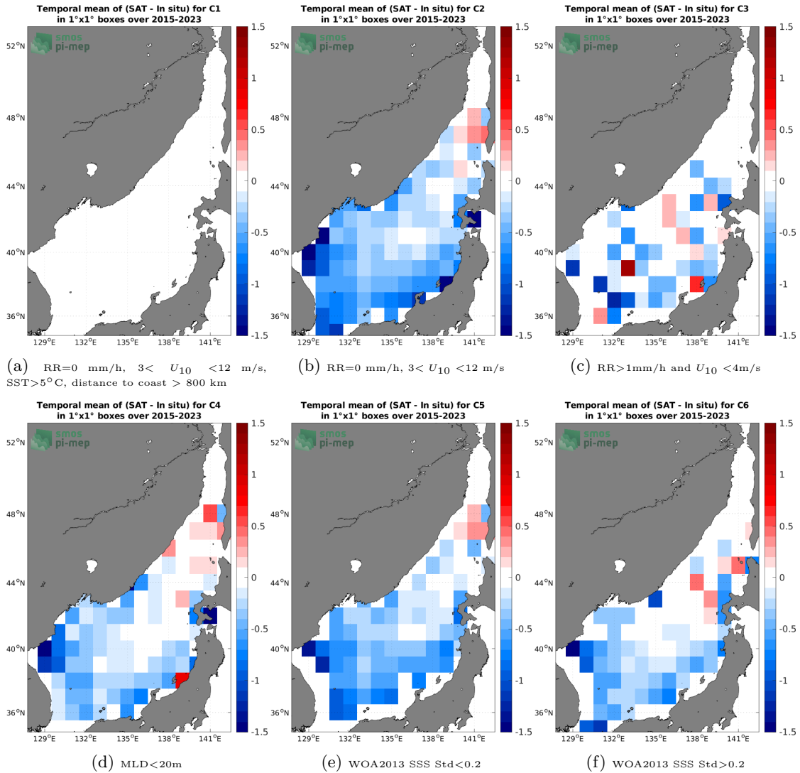
Figure 12: Temporal mean gridded over spatial boxes of size 1^\circ \times 1^\circ of \Delta SSS (SMAP SSS L3 v5 - 8-Day running (RSS) - Argo) for 6 different subdatasets corresponding to: RR=0 mm/h, 3 < U_{10} < 12 m/s, SST > 5^\circ C , distance to coast > 800 km (a), RR=0 mm/h, 3 < U_{10} < 12 m/s (b), RR > 1 mm/h and U_{10} < 4 m/s (c), MLD < 20 m (d), WOA2013 SSS Std < 0.2 (e), WOA2013 SSS Std > 0.2 (f).
