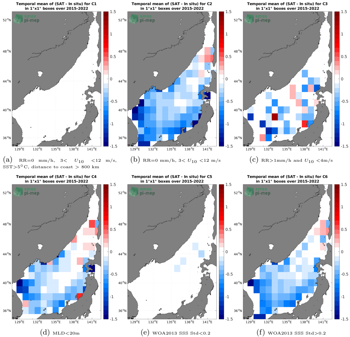
Figure 12: Temporal mean gridded over spatial boxes of size 1^\circ \times 1^\circ of \Delta\text{SSS} (SMAP SSS L3 v5 - 8-Day running (RSS) - Argo) for 6 different subdatasets corresponding to:RR=0 mm/h, 3 < U_{10} < 12 m/s, SST> 5^\circ\text{C} , distance to coast > 800 km (a), RR=0 mm/h, 3 < U_{10} < 12 m/s (b), RR>1mm/h and U_{10} < 4 m/s (c),MLD<20m (d),WOA2013 SSS Std<0.2 (e),WOA2013 SSS Std>0.2 (f).
