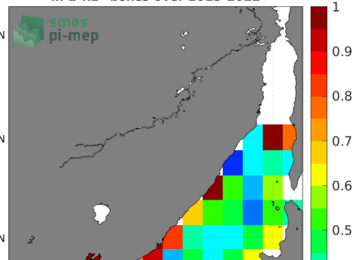
Temporal STD of (Sat - Argo) in 1°x1° boxes over 2015-2022
