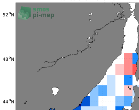
Temporal mean of (Sat - Argo) in 1°x1° boxes over 2015-2022
