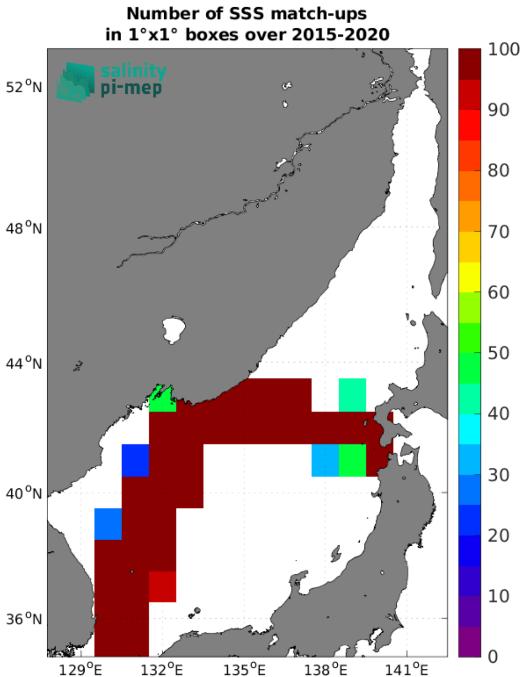
Figure 4: Number of SSS match-ups between TSG (LEGOS-DM) SSS and the SMAP SSS L3 v5 - Monthly (RSS) SSS product for the Sea of Japan Pi-MEP region over 1°x1° boxes and for the full satellite product period.
