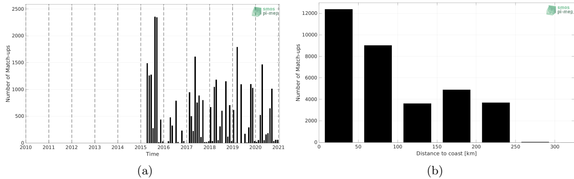
Figure 1: Number of match-ups between TSG (LEGOS-DM) and SMAP SSS L3 v5 - Monthly (RSS) SSS as a function of time (a) and as function of the distance to coast (b) over the Sea of Japan Pi-MEP region and for the full satellite product period.
