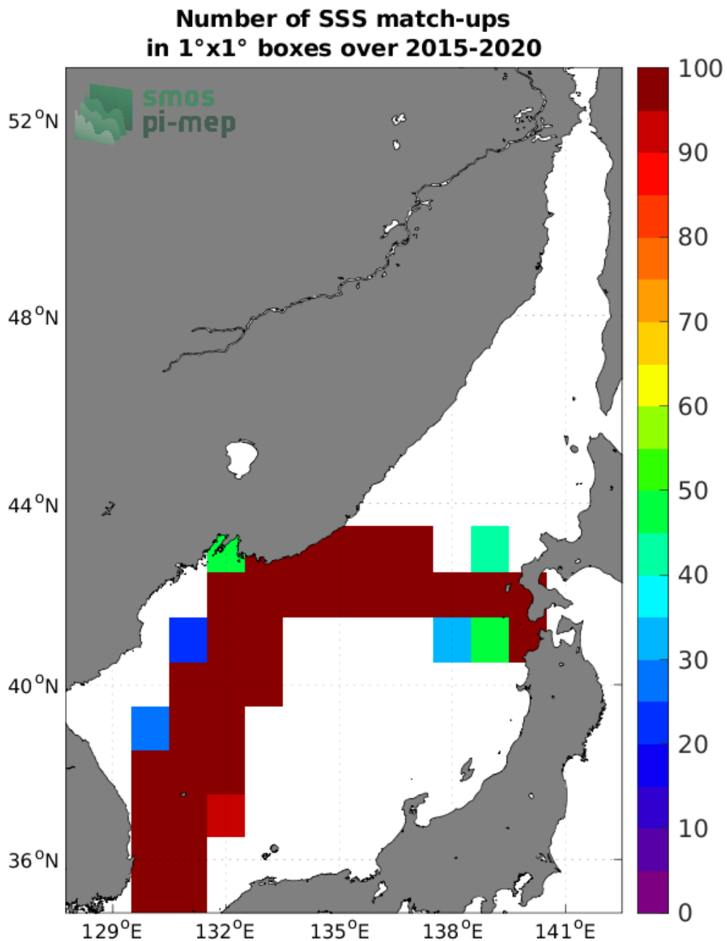
Figure 4: Number of SSS match-ups between TSG (LEGOS-DM) SSS and the SMAP SSS L3 v5 - Monthly (RSS) SSS product for the Sea of Japan Pi-MEP region over 1°×1° boxes and for the full satellite product period.
