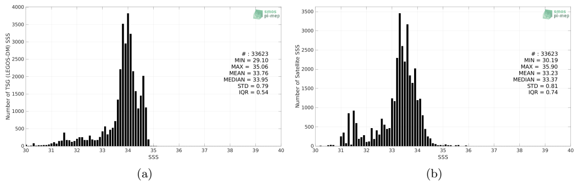
Figure 2: Histograms of SSS from TSG (LEGOS-DM) (a) and SMAP SSS L3 v5 - Monthly (RSS) (b) considering all match-up pairs per bins of 0.1 over the Sea of Japan Pi-MEP region and for the full satellite product period.
