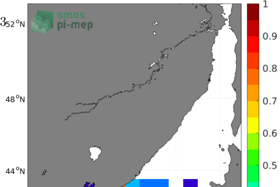
Temporal STD of (Sat - TSG (LEGOS-DM)) in 1°x1° boxes over 2015-2020
