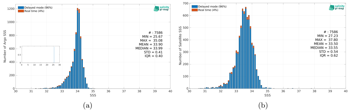
Figure 2: Histograms of SSS from Argos (a) and SMAP SSS L3 v5 - Monthly (RSS) (b) considering all match-up pairs per bins of 0.1 over the Sea of Japan Pi-MEP region and for the full satellite product period.
