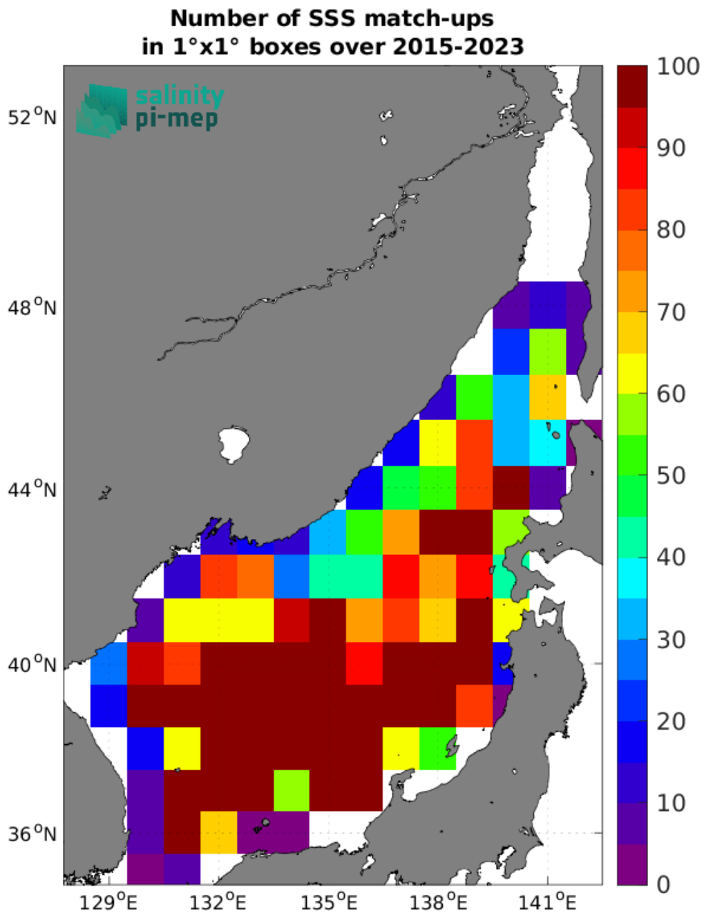
Figure 4: Number of SSS match-ups between Argo SSS and the SMAP SSS L3 v5 - Monthly (RSS) SSS product for the Sea of Japan Pi-MEP region over 1°x1° boxes and for the full satellite product period.
