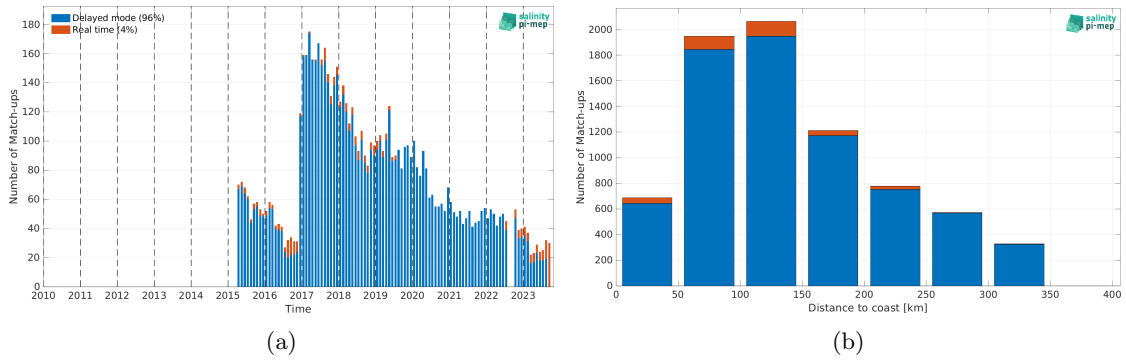
Figure 1: Number of match-ups between Argo and SMAP SSS L3 v5 - Monthly (RSS) SSS as a function of time (a) and as function of the distance to coast (b) over the Sea of Japan Pi-MEP region and for the full satellite product period.
