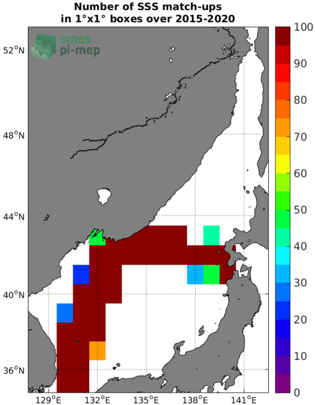
Figure 4: Number of SSS match-ups between TSG (LEGOS-DM) SSS and the SMAP SSS L3 v4 - 8-Day running (RSS) SSS product for the Sea of Japan Pi-MEP region over 1°x1° boxes and for the full satellite product period.
