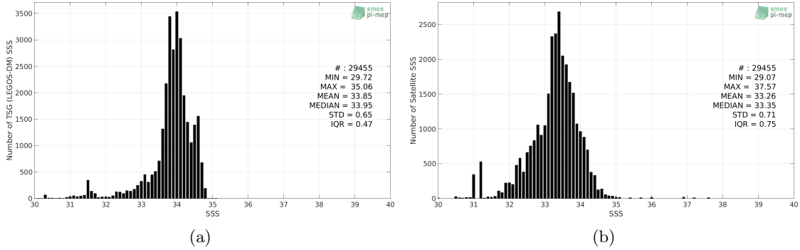
Figure 2: Histograms of SSS from TSG (LEGOS-DM) (a) and SMAP SSS L3 v4 - 8-Day running (RSS) (b) considering all match-up pairs per bins of 0.1 over the Sea of Japan Pi-MEP region and for the full satellite product period.
