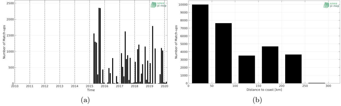
Figure 1: Number of match-ups between TSG (LEGOS-DM) and SMAP SSS L3 v4 - 8-Day running (RSS) SSS as a function of time (a) and as function of the distance to coast (b) over the Sea of Japan Pi-MEP region and for the full satellite product period.
