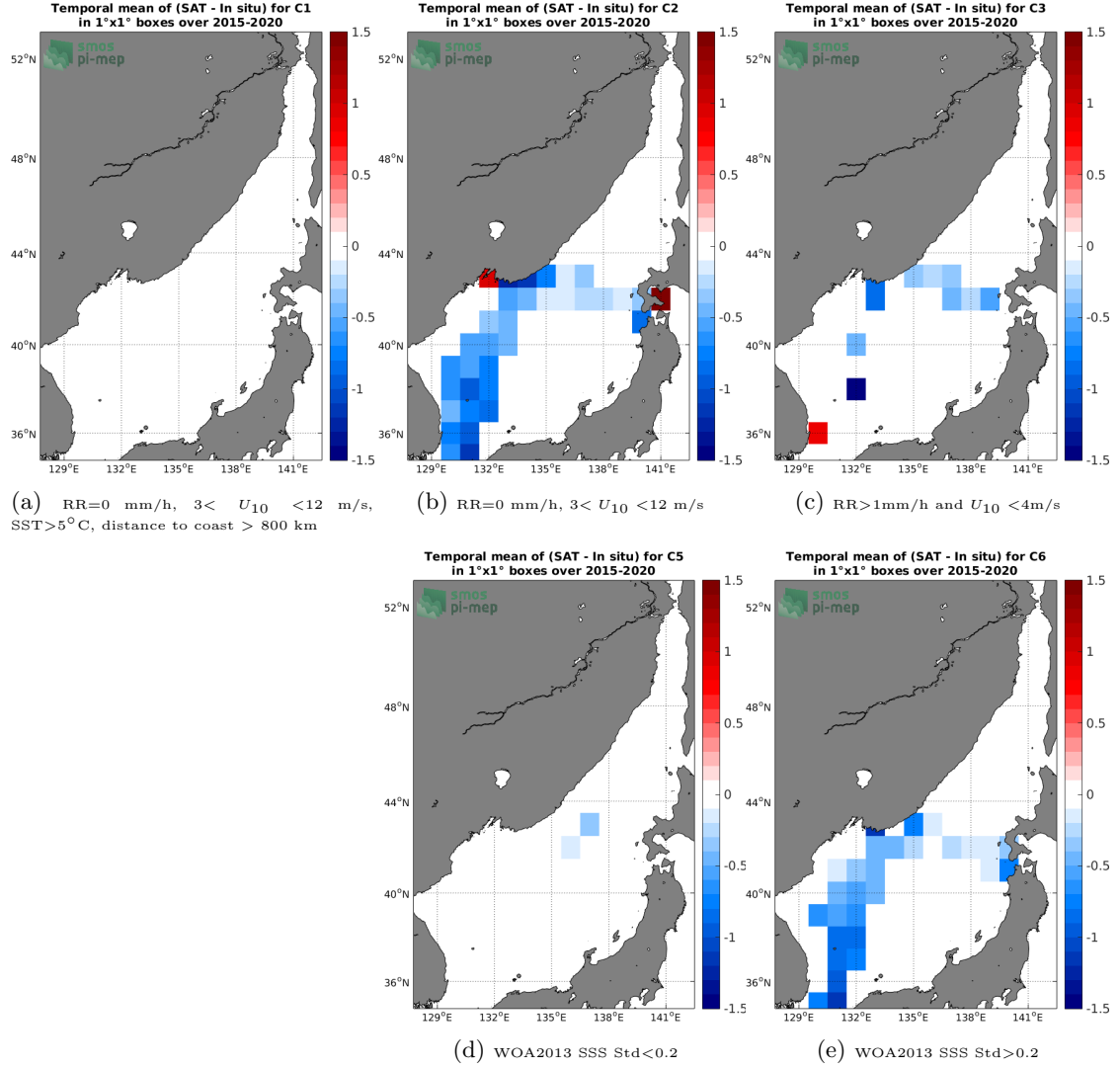
Figure 12: Temporal mean gridded over spatial boxes of size 1^\circ \times 1^\circ of \Delta SSS (SMAP SSS L3 v4 - 8-Day running (RSS) - TSG (LEGOS-DM)) for 5 different subdatasets corresponding to: RR=0 mm/h, 3 < U_{10} < 12 m/s, SST > 5°C, distance to coast > 800 km (a), RR=0 mm/h, 3 < U_{10} < 12 m/s (b), RR > 1 mm/h and U_{10} < 4 m/s (c), WOA2013 SSS Std < 0.2 (d), WOA2013 SSS Std > 0.2 (e).
