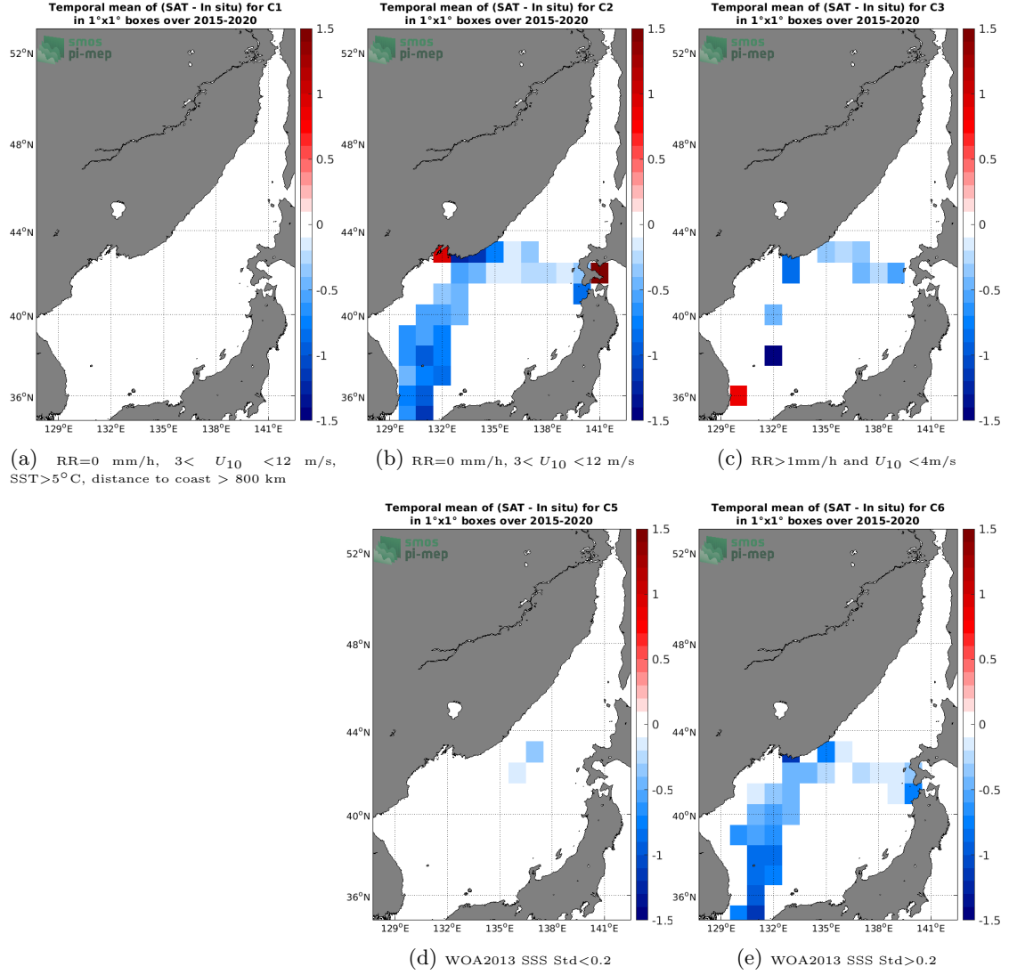
Figure 12: Temporal mean gridded over spatial boxes of size 1°x1° of \Delta\text{SSS} (SMAP SSS L3 v4 - 8-Day running (RSS) - TSG (LEGOS-DM)) for 5 different subdatasets corresponding to: RR=0 mm/h, 3 < U_{10} < 12 m/s, SST > 5^\circ\text{C} , distance to coast > 800 km (a), RR=0 mm/h, 3 < U_{10} < 12 m/s (b), RR > 1 mm/h and U_{10} < 4 m/s (c), WOA2013 SSS Std < 0.2 (d), WOA2013 SSS Std > 0.2 (e).
