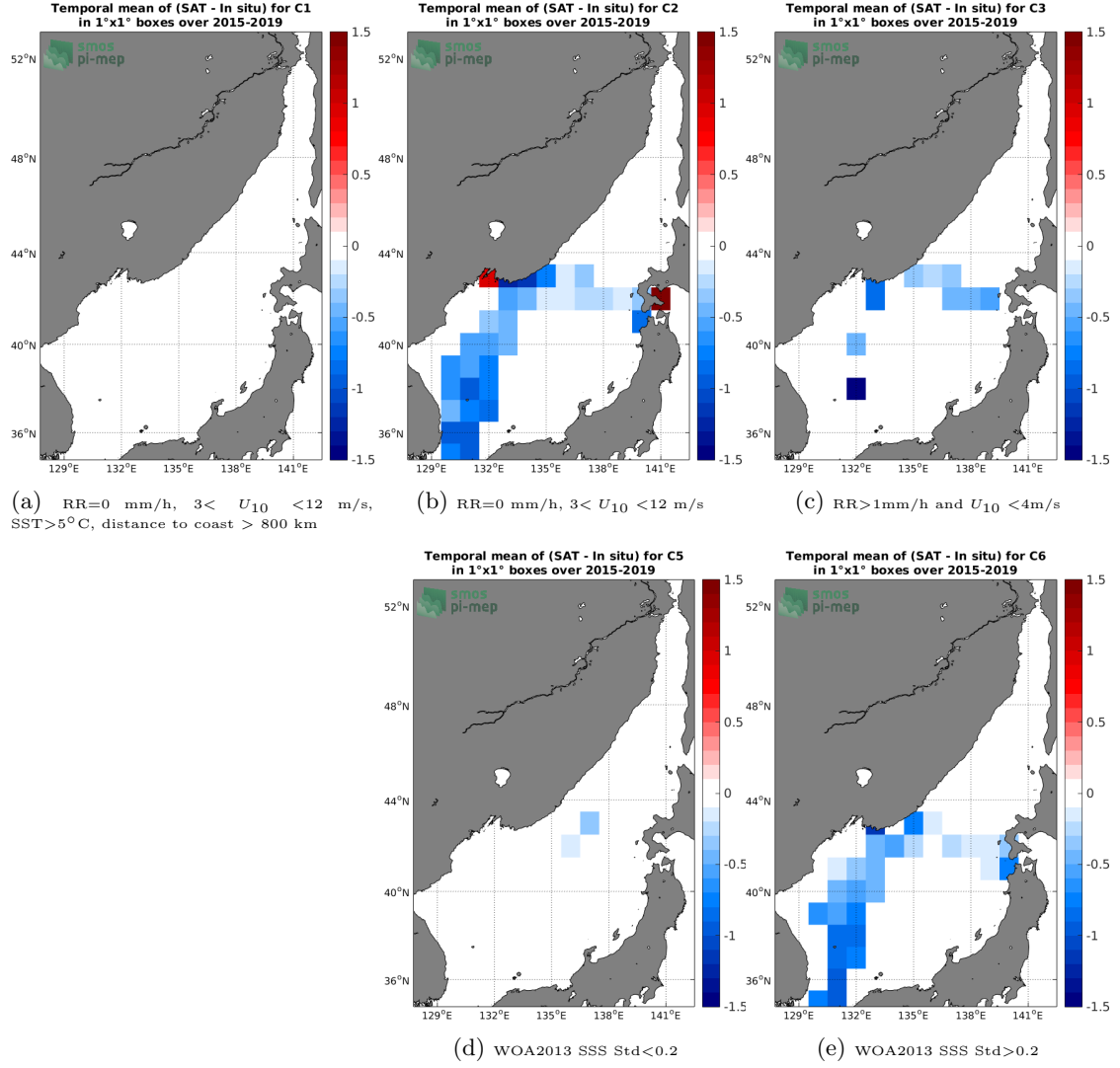
Figure 12: Temporal mean gridded over spatial boxes of size 1°x1° of \Delta\text{SSS} (SMAP-L3-RSS-V4-8DAY-RUNNING - TSG-LEGOS-DM) for 5 different subdatasets corresponding to: RR=0 mm/h, 3 < U_{10} < 12 m/s, SST > 5^\circ\text{C} , distance to coast > 800 km (a), RR=0 mm/h, 3 < U_{10} < 12 m/s (b), RR > 1 mm/h and U_{10} < 4 m/s (c), WOA2013 SSS Std < 0.2 (d), WOA2013 SSS Std > 0.2 (e).
