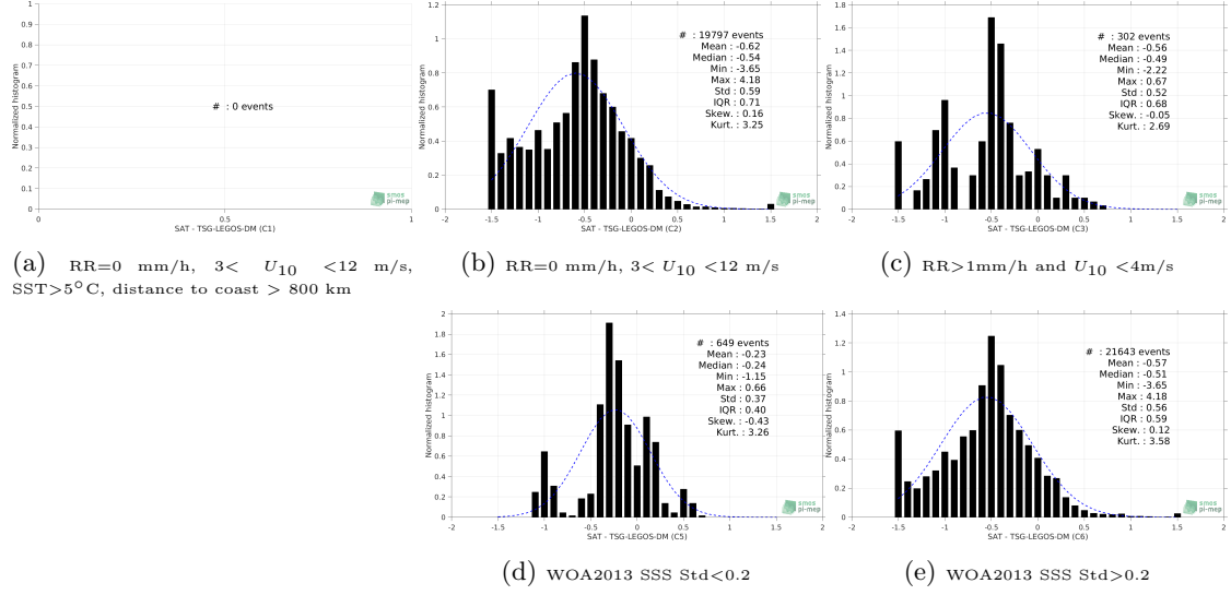
Figure 13: Normalized histogram of \Delta SSS (SMAP-L3-RSS-V4-8DAY-RUNNING - TSG-LEGOS-DM) for 5 different subdatasets corresponding to: RR=0 mm/h, 3 < U_{10} < 12 m/s, SST > 5^\circ C , distance to coast > 800 km (a), RR=0 mm/h, 3 < U_{10} < 12 m/s (b), RR > 1 mm/h and U_{10} < 4 m/s (c), WOA2013 SSS Std < 0.2 (d), WOA2013 SSS Std > 0.2 (e).
