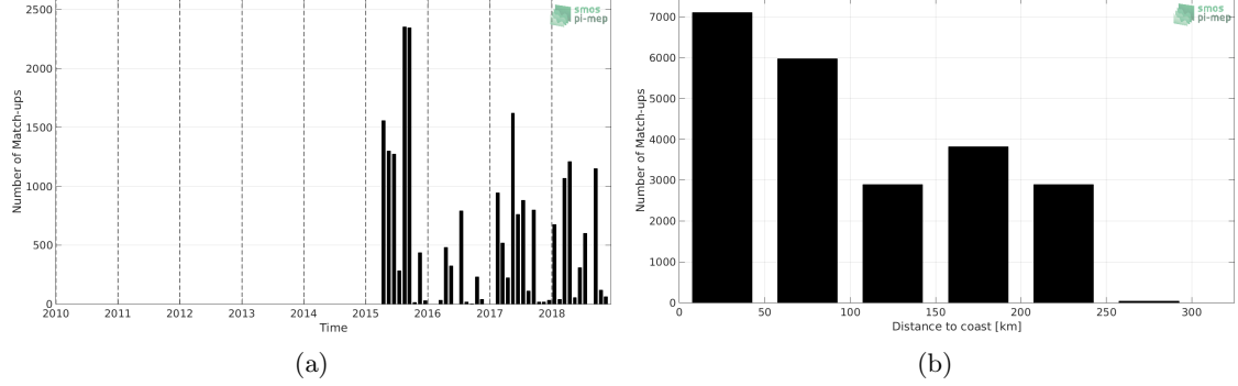
Figure 1: Number of match-ups between TSG-LEGOS-DM and SMAP-L3-RSS-V4-8DAY-RUNNING SSS as a function of time (a) and as function of the distance to coast (b) over the Sea of Japan Pi-MEP region and for the full satellite product period.
