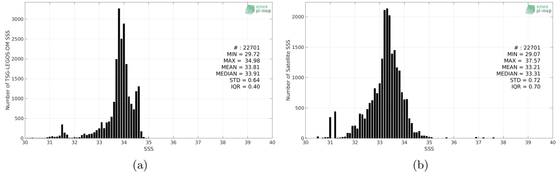
Figure 2: Histograms of SSS from TSG-LEGOS-DM (a) and SMAP-L3-RSS-V4-8DAY-RUNNING (b) considering all match-up pairs per bins of 0.1 over the Sea of Japan Pi-MEP region and for the full satellite product period.
