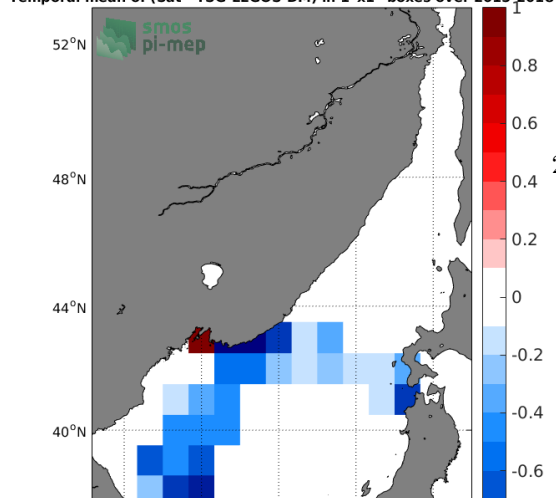
Temporal mean of (Sat - TSG-LEGOS-DM) in 1°x1° boxes over 2015-2018
