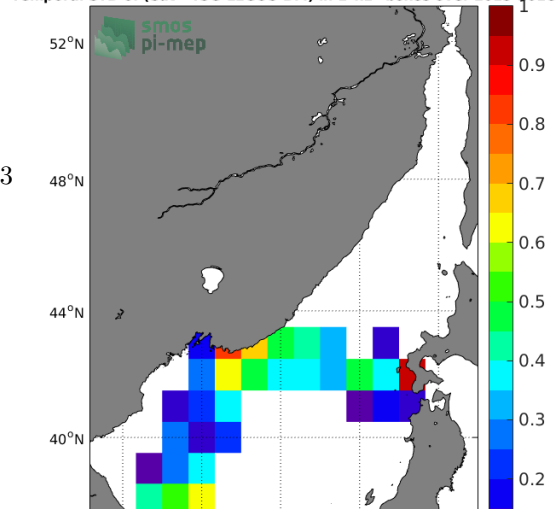
Temporal STD of (Sat - TSG-LEGOS-DM) in 1°x1° boxes over 2015-2018
