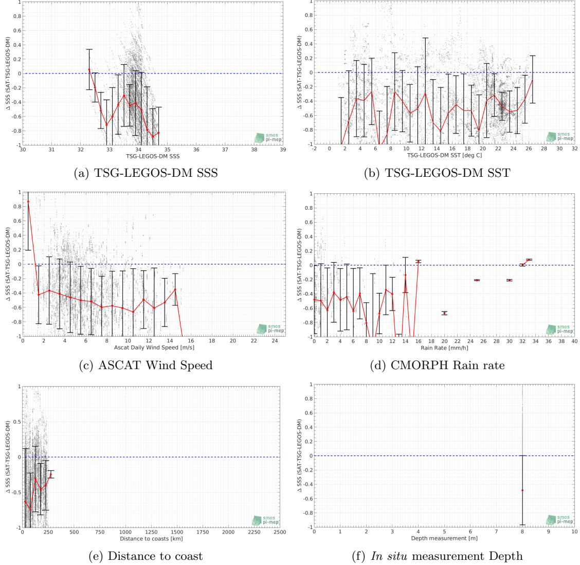
Figure 11: \Delta SSS (Satellite - TSG-LEGOS-DM) sorted as function of TSG-LEGOS-DM SSS values a), TSG-LEGOS-DM SST b), ASCAT Wind speed c), CMORPH rain rate d), distance to coast (e) and in situ measurement depth (f). In all plots the median and Std of \Delta SSS for each bin is indicated by the red curves and black vertical thick bars ( \pm 1 Std)
