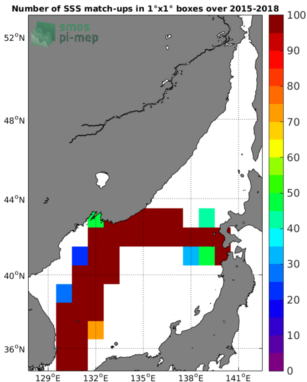
Figure 4: Number of SSS match-ups between TSG-LEGOS-DM SSS and the SMAP-L3-RSS-V4-8DAY-RUNNING SSS product for the Sea of Japan Pi-MEP region over 1°x1° boxes and for the full satellite product period.
