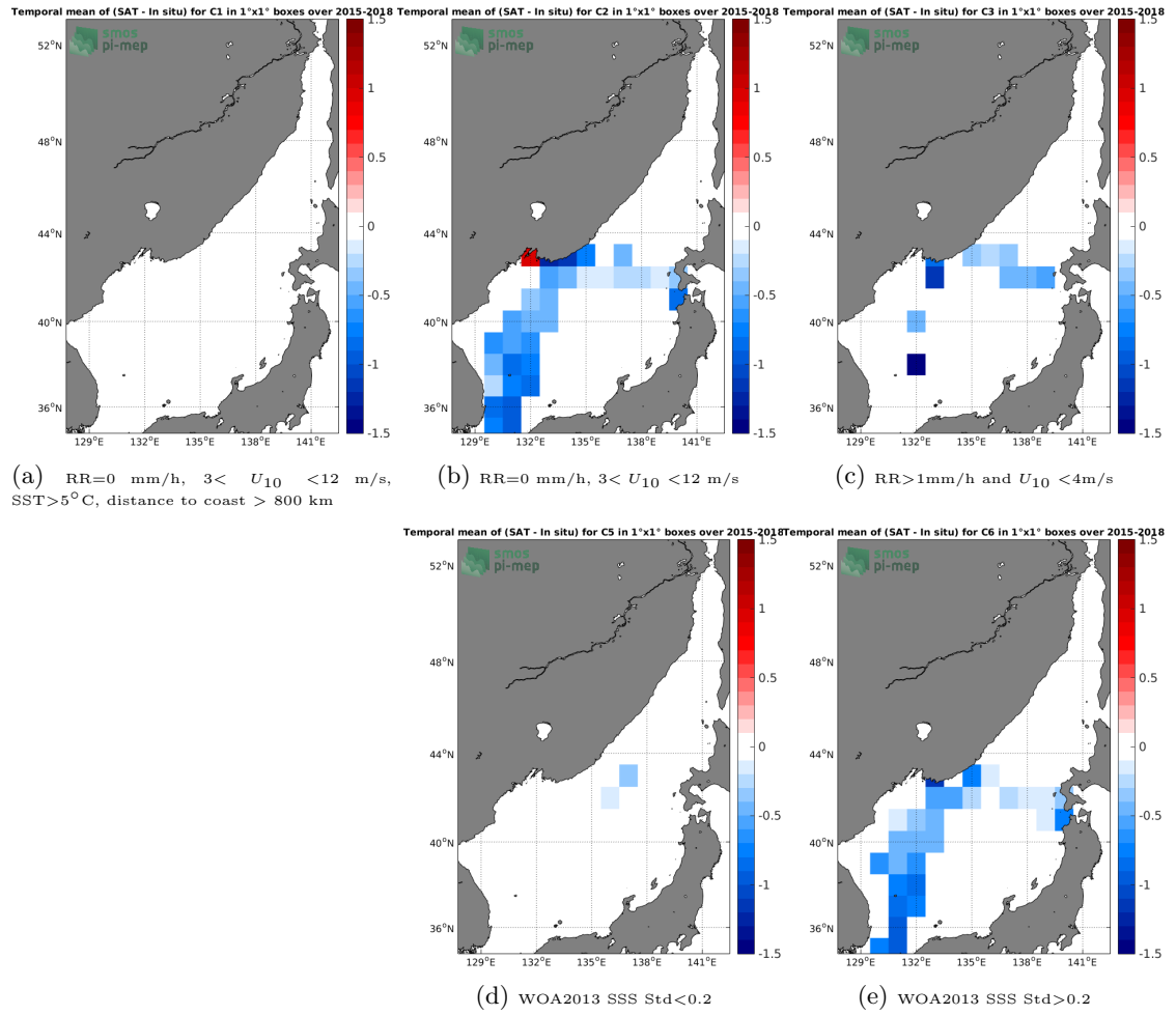
Figure 12: Temporal mean gridded over spatial boxes of size 1^\circ \times 1^\circ of \Delta SSS (SMAP-L3-RSS-V4-8DAY-RUNNING - TSG-LEGOS-DM) for 5 different subdatasets corresponding to: RR=0 mm/h, 3 < U_{10} < 12 m/s, SST>5°C, distance to coast > 800 km (a), RR=0 mm/h, 3 < U_{10} < 12 m/s (b), RR>1mm/h and U_{10} < 4 m/s (c), WOA2013 SSS Std<0.2 (d), WOA2013 SSS Std>0.2 (e).
