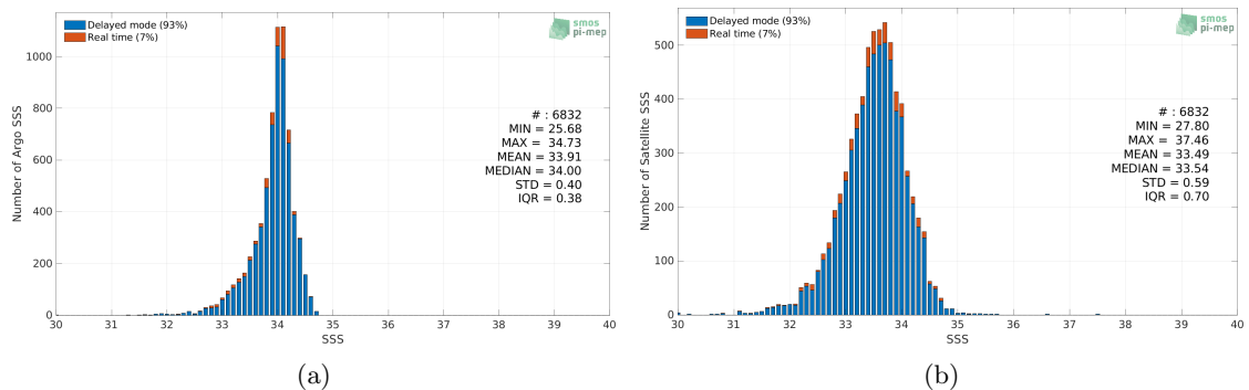
Figure 2: Histograms of SSS from Argo (a) and SMAP SSS L3 v4 - 8-Day running (RSS) (b) considering all match-up pairs per bins of 0.1 over the Sea of Japan Pi-MEP region and for the full satellite product period.
