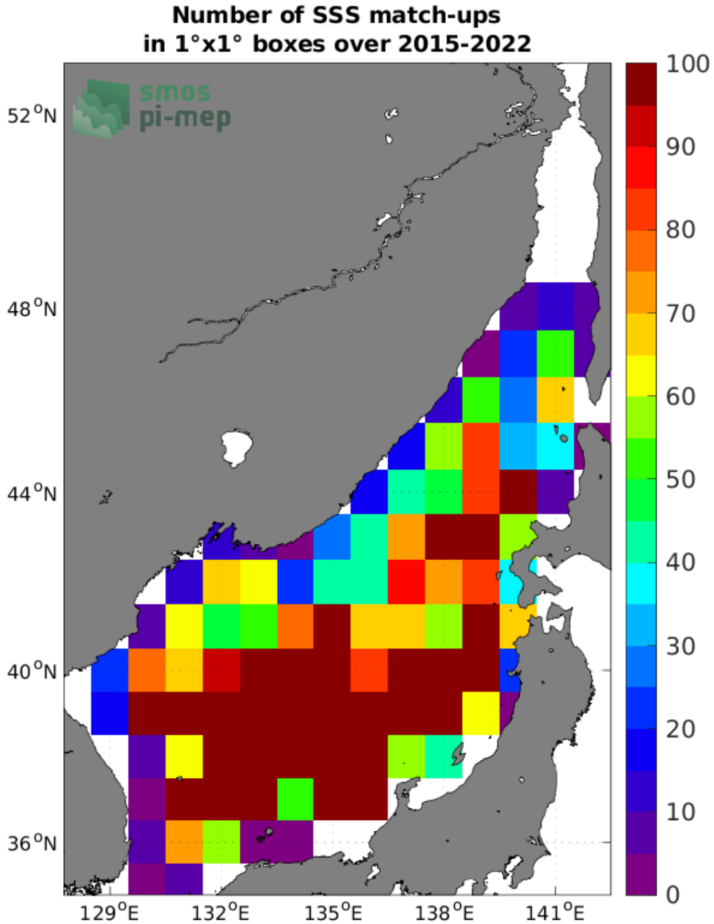
Figure 4: Number of SSS match-ups between Argo SSS and the SMAP SSS L3 v4 - 8-Day running (RSS) SSS product for the Sea of Japan Pi-MEP region over 1°x1° boxes and for the full satellite product period.
