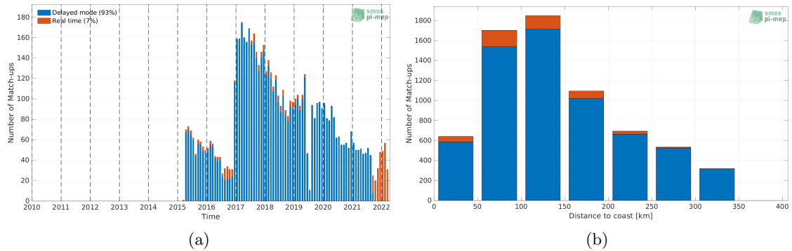
Figure 1: Number of match-ups between Argo and SMAP SSS L3 v4 - 8-Day running (RSS) SSS as a function of time (a) and as function of the distance to coast (b) over the Sea of Japan Pi-MEP region and for the full satellite product period.
