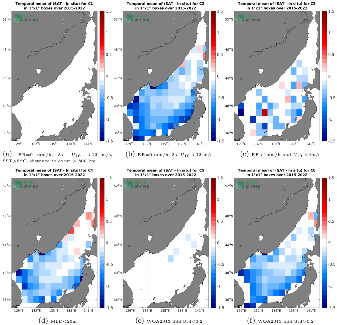
Figure 12: Temporal mean gridded over spatial boxes of size 1^\circ \times 1^\circ of \Delta SSS (SMAP SSS L3 v4 - 8-Day running (RSS) - Argo) for 6 different subdatasets corresponding to: RR=0 mm/h, 3 < U_{10} < 12 m/s, SST > 5^\circ C , distance to coast > 800 km (a), RR=0 mm/h, 3 < U_{10} < 12 m/s (b), RR > 1 mm/h and U_{10} < 4 m/s (c), MLD < 20 m (d), WOA2013 SSS Std < 0.2 (e), WOA2013 SSS Std > 0.2 (f).
