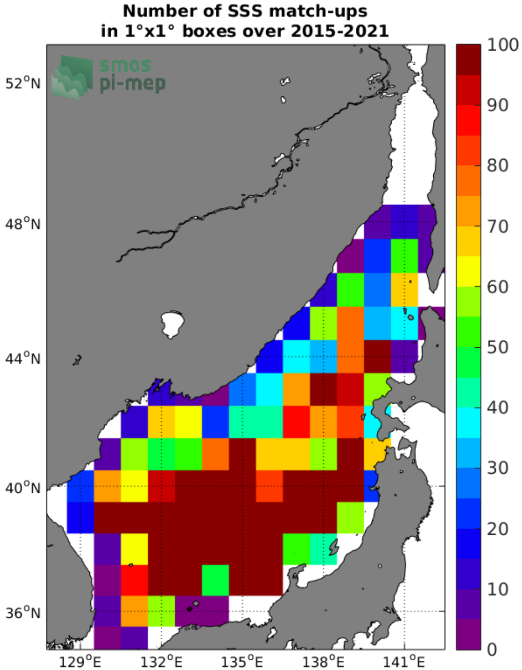
Figure 4: Number of SSS match-ups between Argo SSS and the SMAP SSS L3 v4 - 8-Day running (RSS) SSS product for the Sea of Japan Pi-MEP region over 1^\circ \times 1^\circ boxes and for the full satellite product period.
