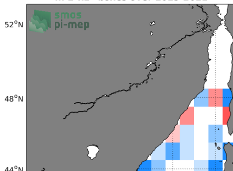
Temporal mean of (Sat - Argo) in 1°x1° boxes over 2015-2021
