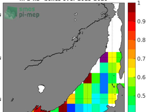
Temporal STD of (Sat - Argo) in 1°x1° boxes over 2015-2020
