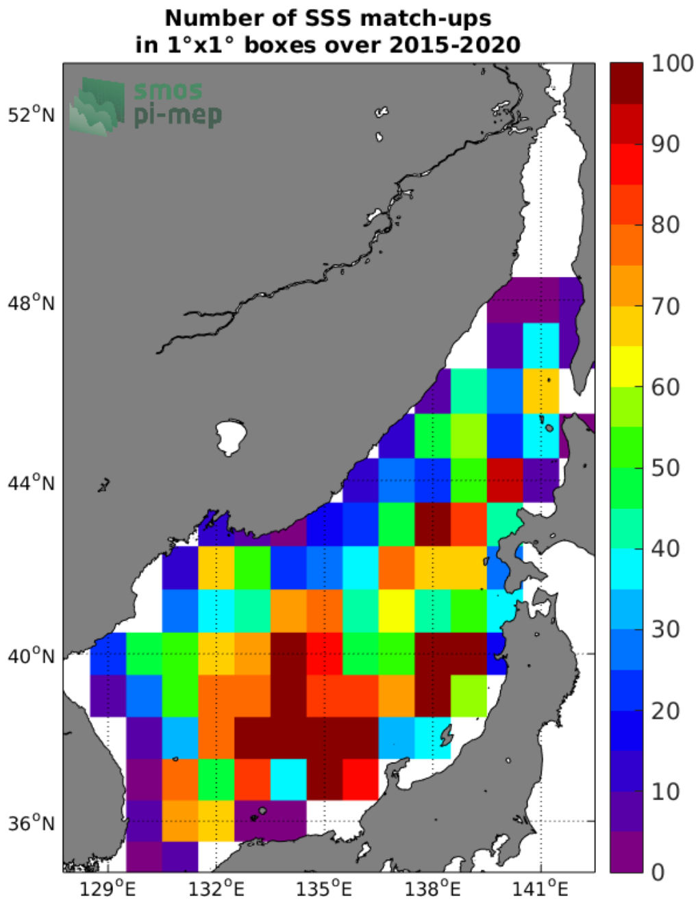
Figure 4: Number of SSS match-ups between Argo SSS and the SMAP-L3-RSS-V4-8DAY-RUNNING SSS product for the Sea of Japan Pi-MEP region over 1°x1° boxes and for the full satellite product period.
