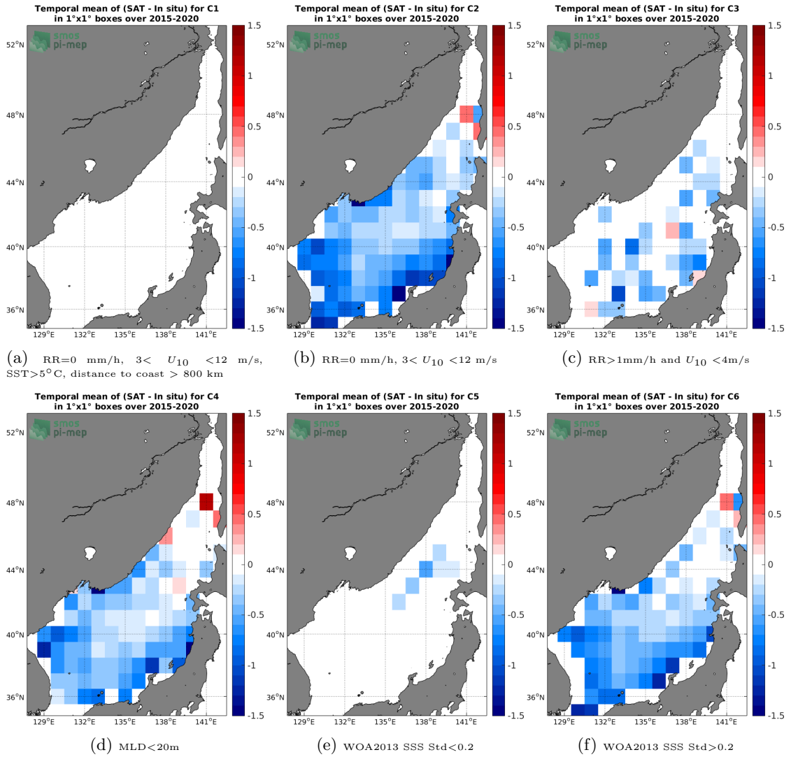
Figure 12: Temporal mean gridded over spatial boxes of size 1°x1° of \Delta SSS (SMAP-L3-RSS-V4-8DAY-RUNNING - Argo) for 6 different subdatasets corresponding to:RR=0 mm/h, 3 < U_{10} < 12 m/s, SST>5°C, distance to coast > 800 km (a), RR=0 mm/h, 3 < U_{10} < 12 m/s (b), RR>1mm/h and U_{10} < 4 m/s (c),MLD<20m (d),WOA2013 SSS Std<0.2 (e),WOA2013 SSS Std>0.2 (f).
