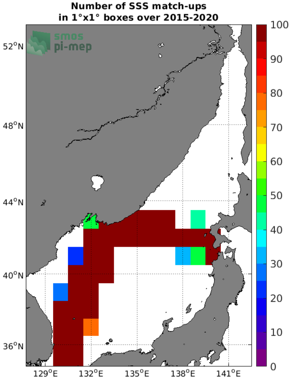
Figure 4: Number of SSS match-ups between TSG (LEGOS-DM) SSS and the SMAP SSS L3 v4 - Monthly (RSS) SSS product for the Sea of Japan Pi-MEP region over 1°x1° boxes and for the full satellite product period.
