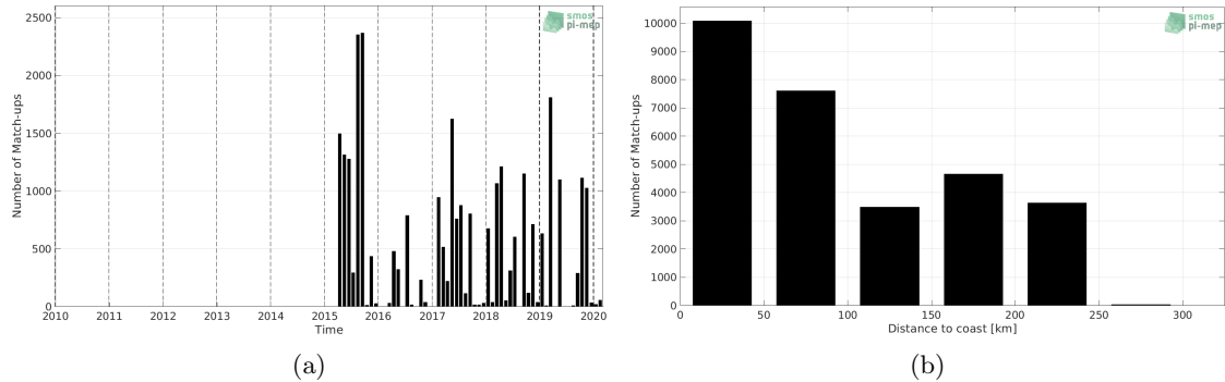
Figure 1: Number of match-ups between TSG (LEGOS-DM) and SMAP SSS L3 v4 - Monthly (RSS) SSS as a function of time (a) and as function of the distance to coast (b) over the Sea of Japan Pi-MEP region and for the full satellite product period.
