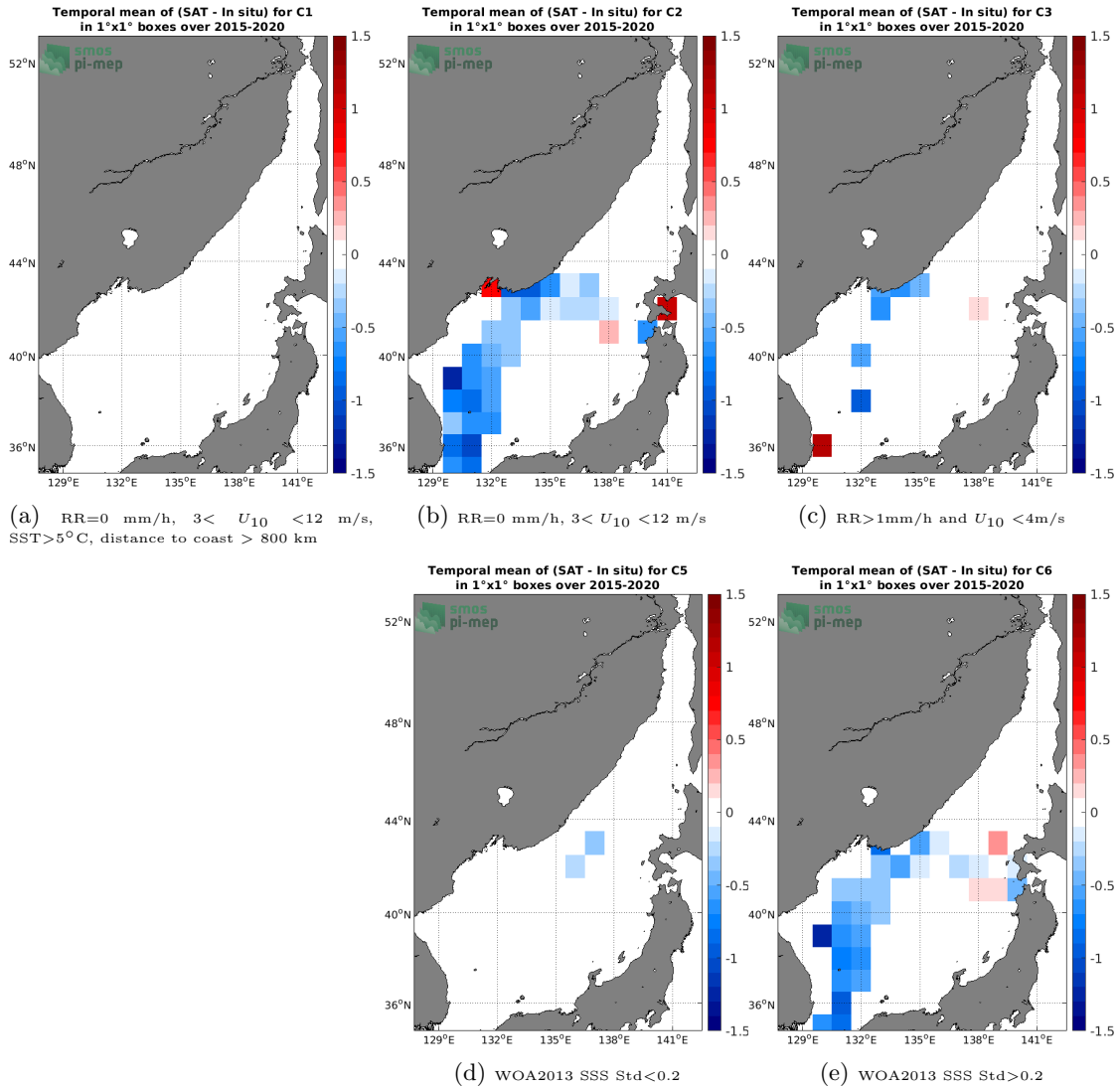
Figure 12: Temporal mean gridded over spatial boxes of size 1°x1° of \Delta SSS (SMAP SSS L3 v4 - Monthly (RSS) - TSG (LEGOS-DM)) for 5 different subdatasets corresponding to:RR=0 mm/h, 3 < U_{10} < 12 m/s, SST>5°C, distance to coast > 800 km (a), RR=0 mm/h, 3 < U_{10} < 12 m/s (b), RR>1mm/h and U_{10} < 4 m/s (c), WOA2013 SSS Std<0.2 (d), WOA2013 SSS Std>0.2 (e).
