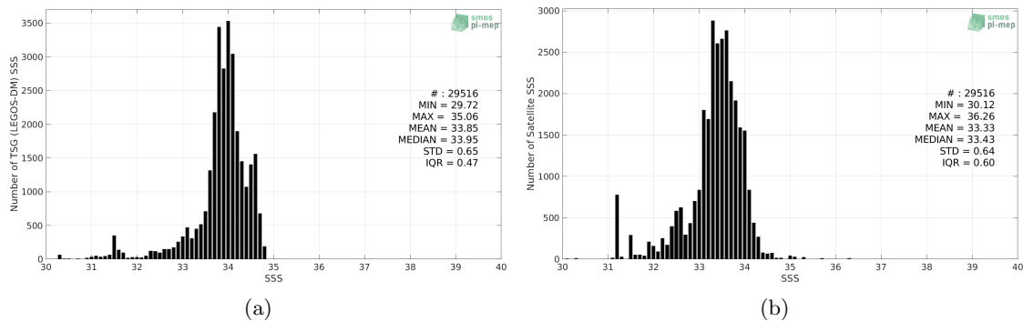
Figure 2: Histograms of SSS from TSG (LEGOS-DM) (a) and SMAP SSS L3 v4 - Monthly (RSS) (b) considering all match-up pairs per bins of 0.1 over the Sea of Japan Pi-MEP region and for the full satellite product period.
