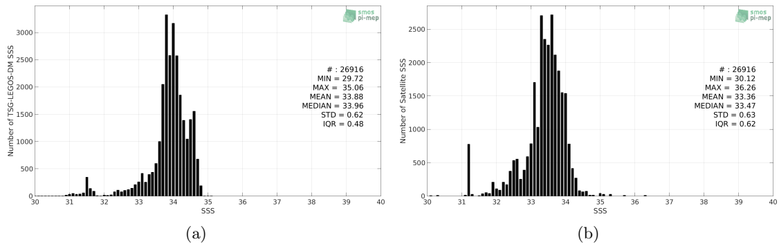
Figure 2: Histograms of SSS from TSG-LEGOS-DM (a) and SMAP-L3-RSS-V4-MONTHLY (b) considering all match-up pairs per bins of 0.1 over the Sea of Japan Pi-MEP region and for the full satellite product period.
