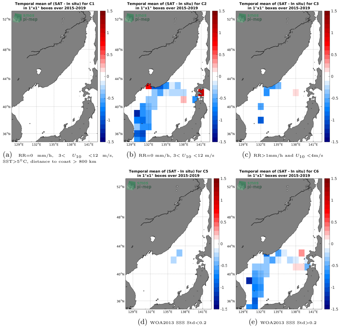
Figure 12: Temporal mean gridded over spatial boxes of size 1^\circ \times 1^\circ of \Delta\text{SSS} (SMAP-L3-RSS-V4-MONTHLY - TSG-LEGOS-DM) for 5 different subdatasets corresponding to: RR=0 mm/h, 3 < U_{10} < 12 m/s, SST > 5^\circ\text{C} , distance to coast > 800 km (a), RR=0 mm/h, 3 < U_{10} < 12 m/s (b), RR > 1 mm/h and U_{10} < 4 m/s (c), WOA2013 SSS Std < 0.2 (d), WOA2013 SSS Std > 0.2 (e).
