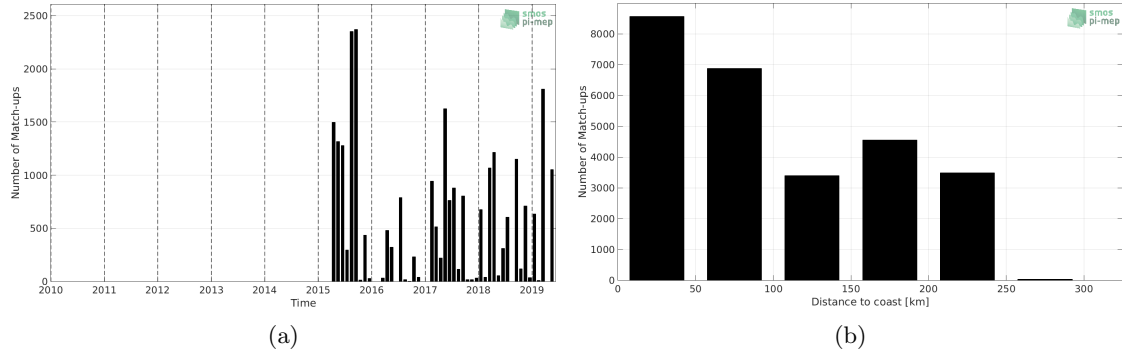
Figure 1: Number of match-ups between TSG-LEGOS-DM and SMAP-L3-RSS-V4-MONTHLY SSS as a function of time (a) and as function of the distance to coast (b) over the Sea of Japan Pi-MEP region and for the full satellite product period.
