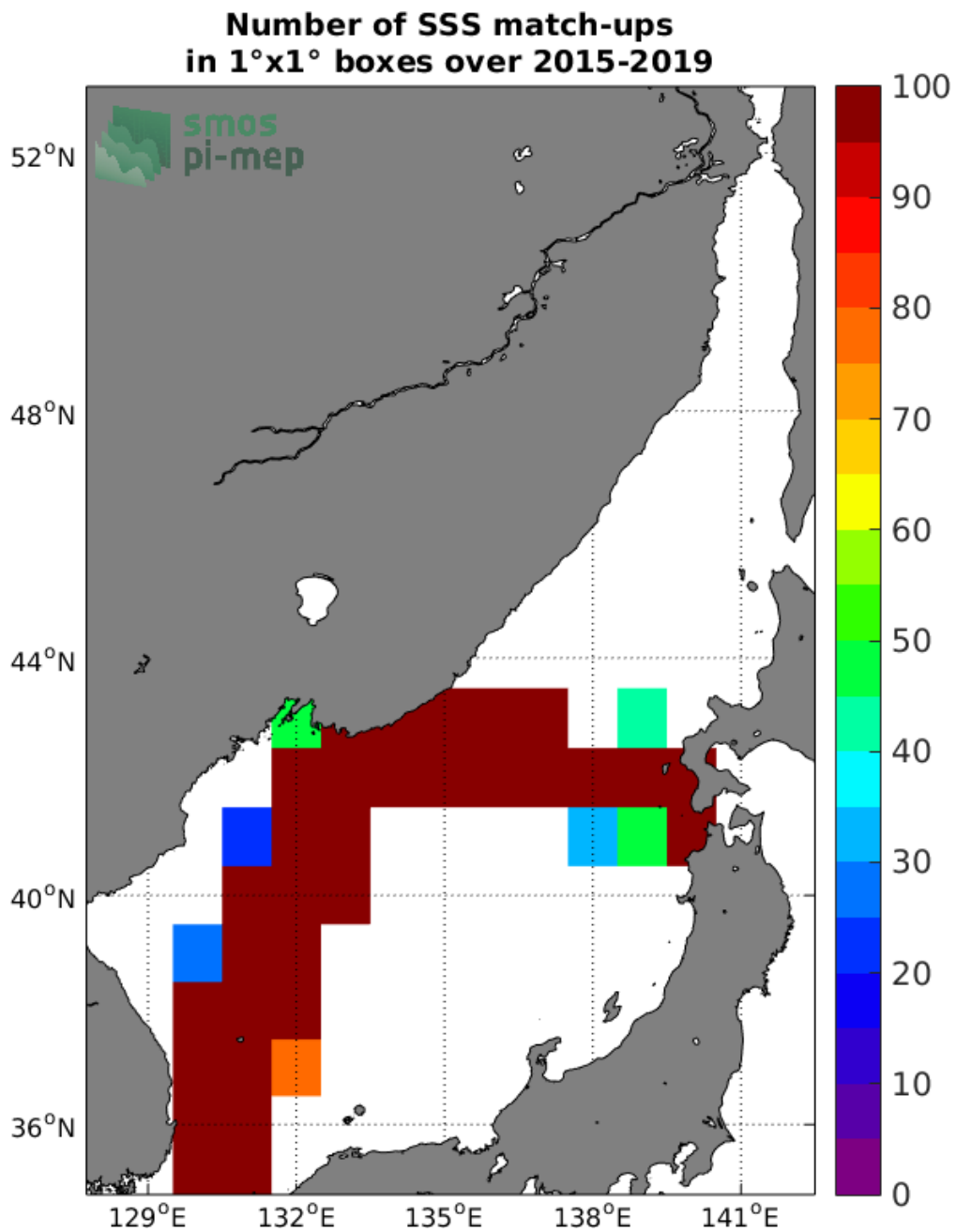
Figure 4: Number of SSS match-ups between TSG-LEGOS-DM SSS and the SMAP-L3-RSS-V4-MONTHLY SSS product for the Sea of Japan Pi-MEP region over 1°x1° boxes and for the full satellite product period.
