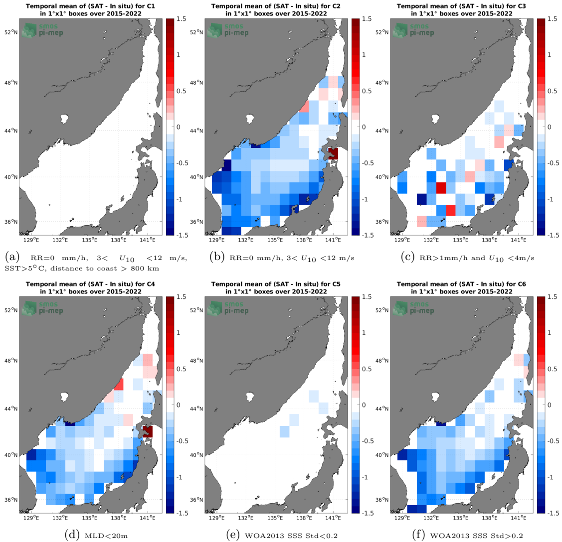
Figure 12: Temporal mean gridded over spatial boxes of size 1^\circ \times 1^\circ of \Delta SSS (SMAP SSS L3 v4 - Monthly (RSS) - Argo) for 6 different subdatasets corresponding to: RR=0 mm/h, 3 < U_{10} < 12 m/s, SST > 5^\circ\text{C} , distance to coast > 800 km (a), RR=0 mm/h, 3 < U_{10} < 12 m/s (b), RR > 1 mm/h and U_{10} < 4 m/s (c), MLD < 20 m (d), WOA2013 SSS Std < 0.2 (e), WOA2013 SSS Std > 0.2 (f).
