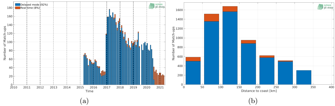
Figure 1: Number of match-ups between Argo and SMAP SSS L3 v4 - Monthly (RSS) SSS as a function of time (a) and as function of the distance to coast (b) over the Sea of Japan Pi-MEP region and for the full satellite product period.
