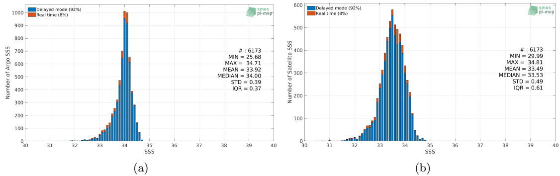
Figure 2: Histograms of SSS from Argo (a) and SMAP SSS L3 v4 - Monthly (RSS) (b) considering all match-up pairs per bins of 0.1 over the Sea of Japan Pi-MEP region and for the full satellite product period.
