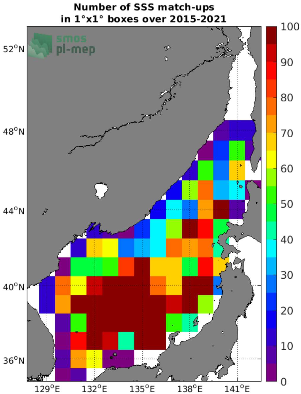
Figure 4: Number of SSS match-ups between Argo SSS and the SMAP SSS L3 v4 - Monthly (RSS) SSS product for the Sea of Japan Pi-MEP region over 1°x1° boxes and for the full satellite product period.
