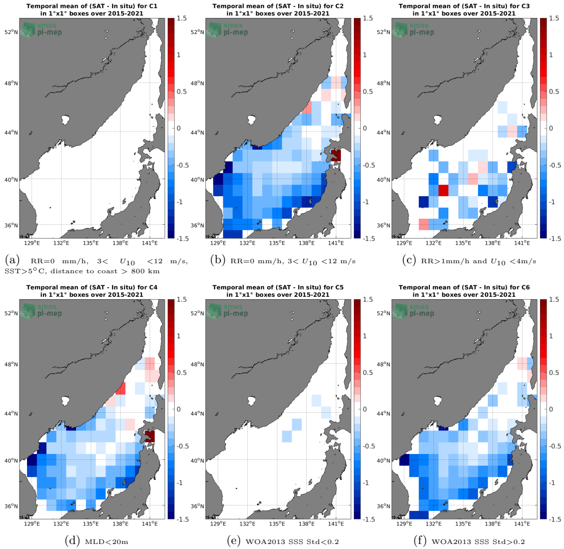
Figure 12: Temporal mean gridded over spatial boxes of size 1°x1° of \Delta SSS (SMAP SSS L3 v4 - Monthly (RSS) - Argo) for 6 different subdatasets corresponding to:RR=0 mm/h, 3 < U_{10} < 12 m/s, SST>5°C, distance to coast > 800 km (a), RR=0 mm/h, 3 < U_{10} < 12 m/s (b), RR>1mm/h and U_{10} < 4 m/s (c),MLD<20m (d),WOA2013 SSS Std<0.2 (e),WOA2013 SSS Std>0.2 (f).
