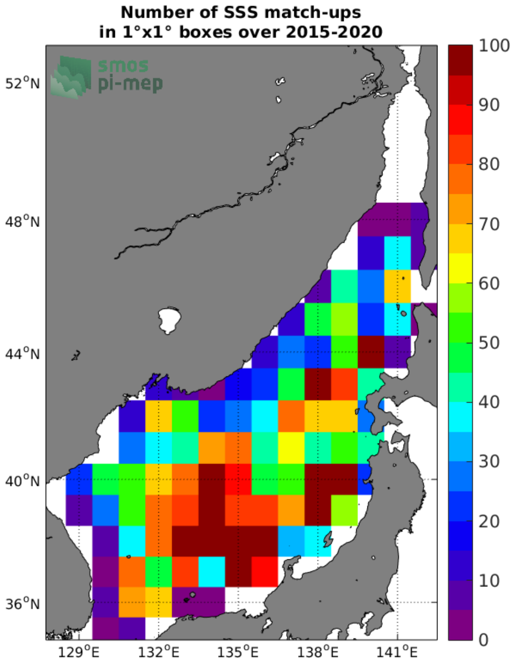
Figure 4: Number of SSS match-ups between Argo SSS and the SMAP-L3-RSS-V4-MONTHLY SSS product for the Sea of Japan Pi-MEP region over 1°x1° boxes and for the full satellite product period.
