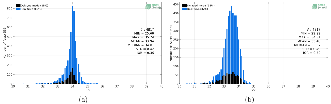
Figure 2: Histograms of SSS from Argo (a) and SMAP-L3-RSS-V4-MONTHLY (b) considering all match-up pairs per bins of 0.1 over the Sea of Japan Pi-MEP region and for the full satellite product period.
