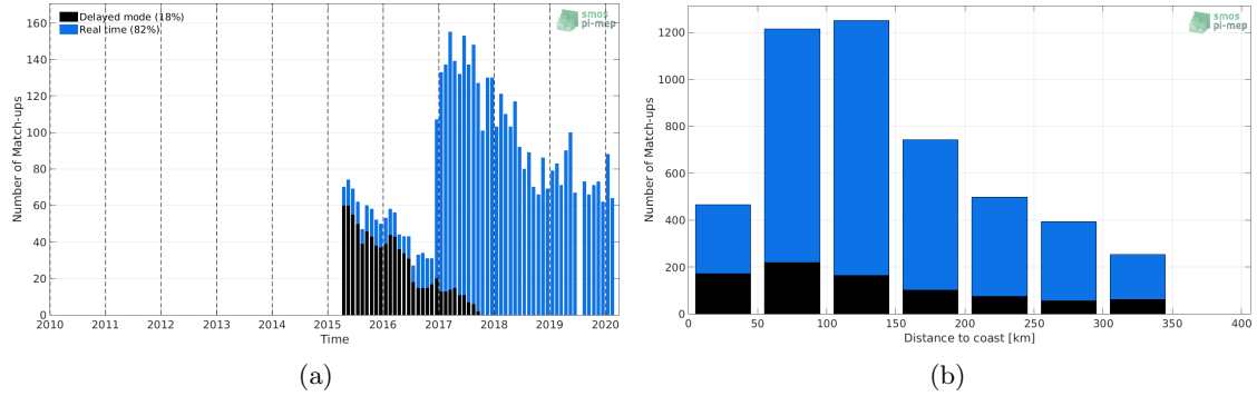
Figure 1: Number of match-ups between Argo and SMAP-L3-RSS-V4-MONTHLY SSS as a function of time (a) and as function of the distance to coast (b) over the Sea of Japan Pi-MEP region and for the full satellite product period.
