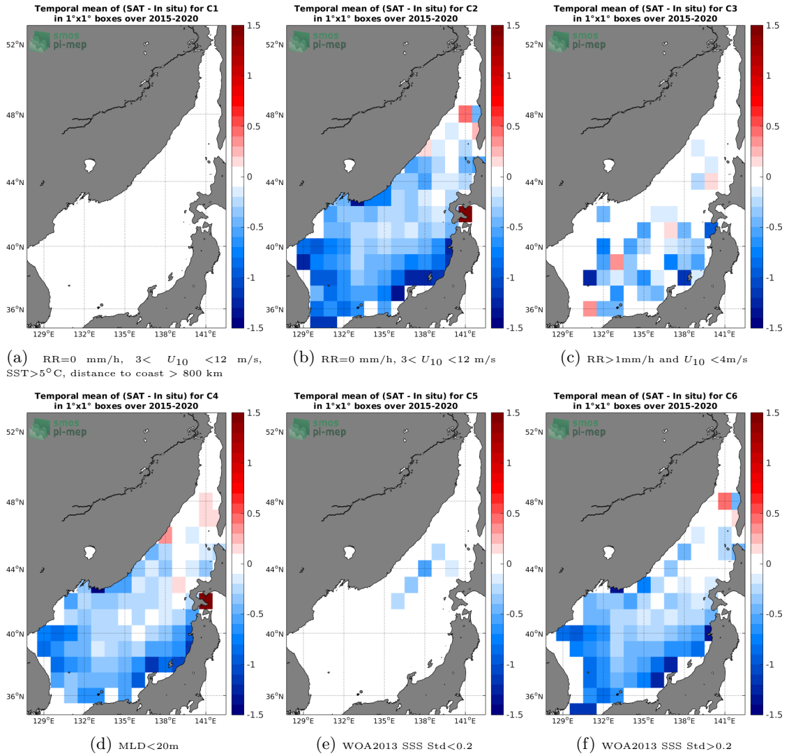
Figure 12: Temporal mean gridded over spatial boxes of size 1°x1° of \Delta SSS (SMAP-L3-RSS-V4-MONTHLY - Argo) for 6 different subdatasets corresponding to: RR=0 mm/h, 3 < U_{10} < 12 m/s, SST > 5^\circ\text{C} , distance to coast > 800 km (a), RR=0 mm/h, 3 < U_{10} < 12 m/s (b), RR > 1 mm/h and U_{10} < 4 m/s (c), MLD < 20 m (d), WOA2013 SSS Std < 0.2 (e), WOA2013 SSS Std > 0.2 (f).
