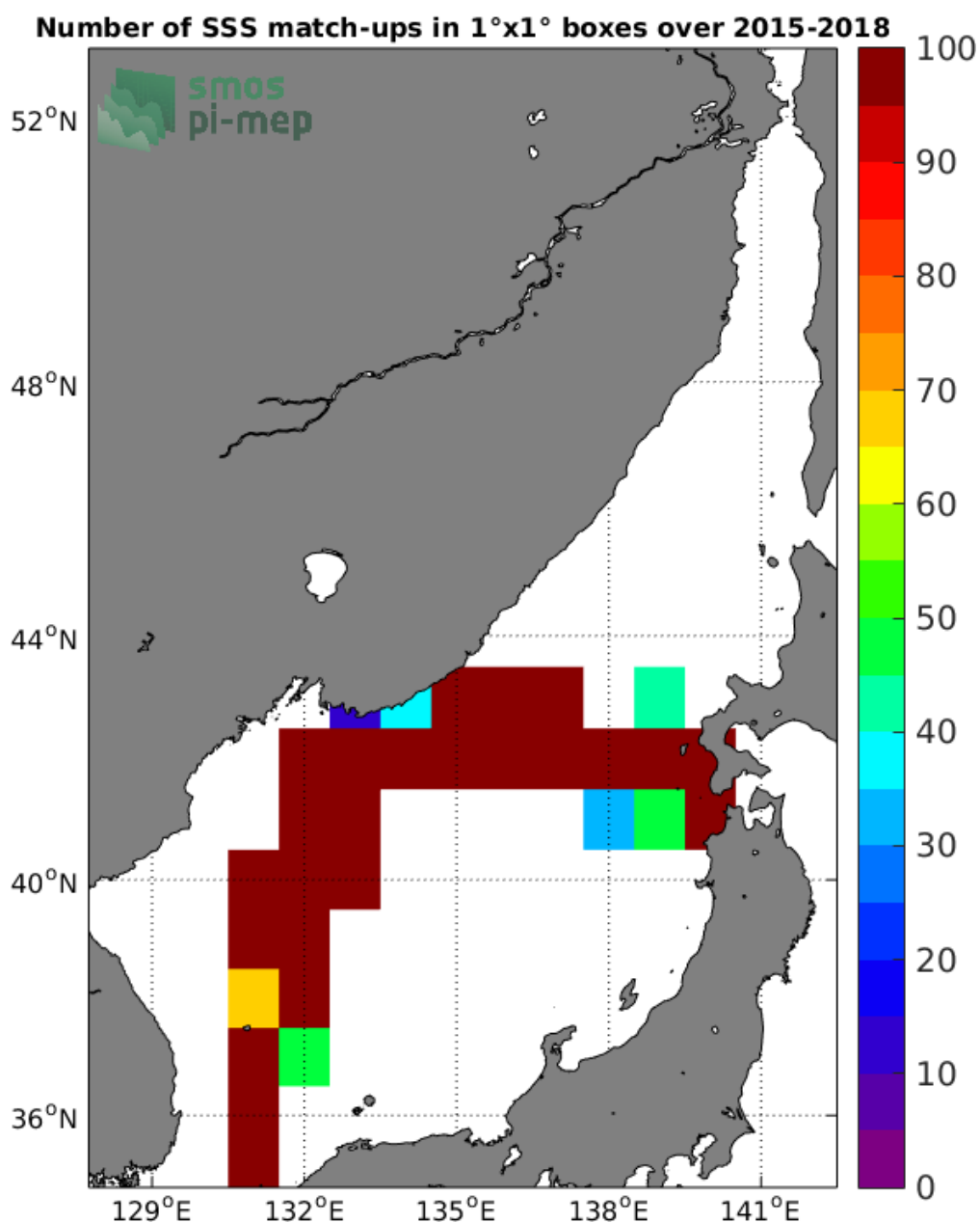
Figure 4: Number of SSS match-ups between TSG-LEGOS-DM SSS and the SMAP-L3-RSS-V3-8DAY-RUNNING-40KM SSS product for the Sea of Japan Pi-MEP region over 1°x1° boxes and for the full satellite product period.
