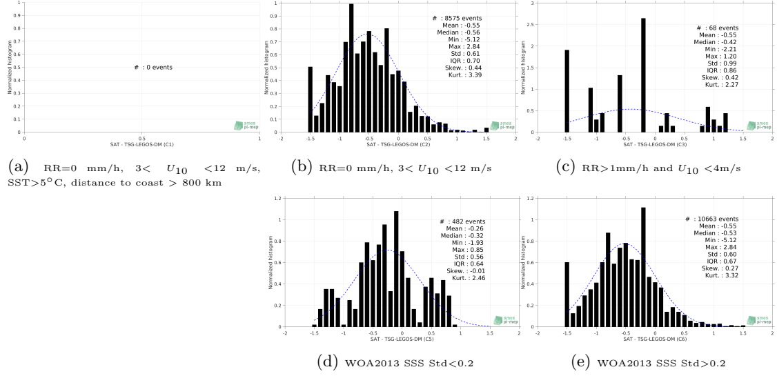
Figure 13: Normalized histogram of \Delta\text{SSS} (SMAP-L3-RSS-V3-8DAY-RUNNING-40KM - TSG-LEGOS-DM) for 5 different subdatasets corresponding to: RR=0 mm/h, 3 < U_{10} < 12 m/s, SST > 5^\circ\text{C} , distance to coast > 800 km (a), RR=0 mm/h, 3 < U_{10} < 12 m/s (b), RR > 1\text{mm/h} and U_{10} < 4\text{m/s} (c), WOA2013 SSS \text{Std} < 0.2 (d), WOA2013 SSS \text{Std} > 0.2 (e).
