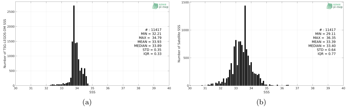
Figure 2: Histograms of SSS from TSG-LEGOS-DM (a) and SMAP-L3-RSS-V3-8DAY-RUNNING-40KM (b) considering all match-up pairs per bins of 0.1 over the Sea of Japan Pi-MEP region and for the full satellite product period.
