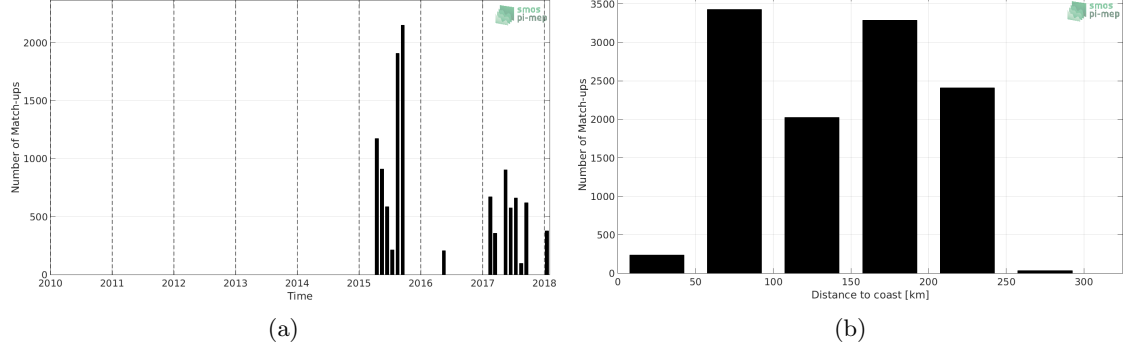
Figure 1: Number of match-ups between TSG-LEGOS-DM and SMAP-L3-RSS-V3-8DAY-RUNNING-40KM SSS as a function of time (a) and as function of the distance to coast (b) over the Sea of Japan Pi-MEP region and for the full satellite product period.
