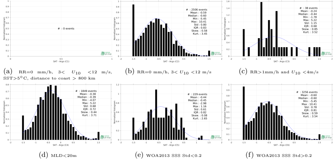
Figure 13: Normalized histogram of \Delta SSS (SMAP-L3-RSS-V3-8DAY-RUNNING-40KM - Argo) for 6 different subdatasets corresponding to: RR=0 mm/h, 3 < U_{10} < 12 m/s, SST > 5°C, distance to coast > 800 km (a), RR=0 mm/h, 3 < U_{10} < 12 m/s (b), RR > 1mm/h and U_{10} < 4 m/s (c), MLD < 20m (d), WOA2013 SSS Std < 0.2 (e), WOA2013 SSS Std > 0.2 (f).
