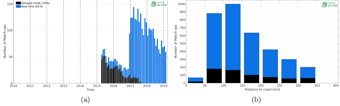
Figure 1: Number of match-ups between Argo and SMAP-L3-RSS-V3-8DAY-RUNNING-40KM SSS as a function of time (a) and as function of the distance to coast (b) over the Sea of Japan Pi-MEP region and for the full satellite product period.
