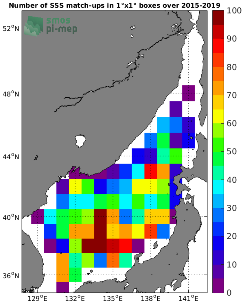
Figure 4: Number of SSS match-ups between Argo SSS and the SMAP-L3-RSS-V3-8DAY-RUNNING-40KM SSS product for the Sea of Japan Pi-MEP region over 1°x1° boxes and for the full satellite product period.
