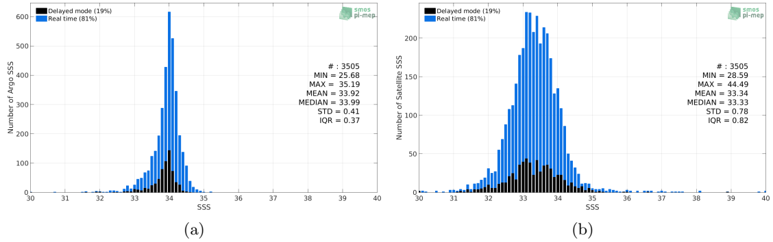
Figure 2: Histograms of SSS from Argo (a) and SMAP-L3-RSS-V3-8DAY-RUNNING-40KM (b) considering all match-up pairs per bins of 0.1 over the Sea of Japan Pi-MEP region and for the full satellite product period.
