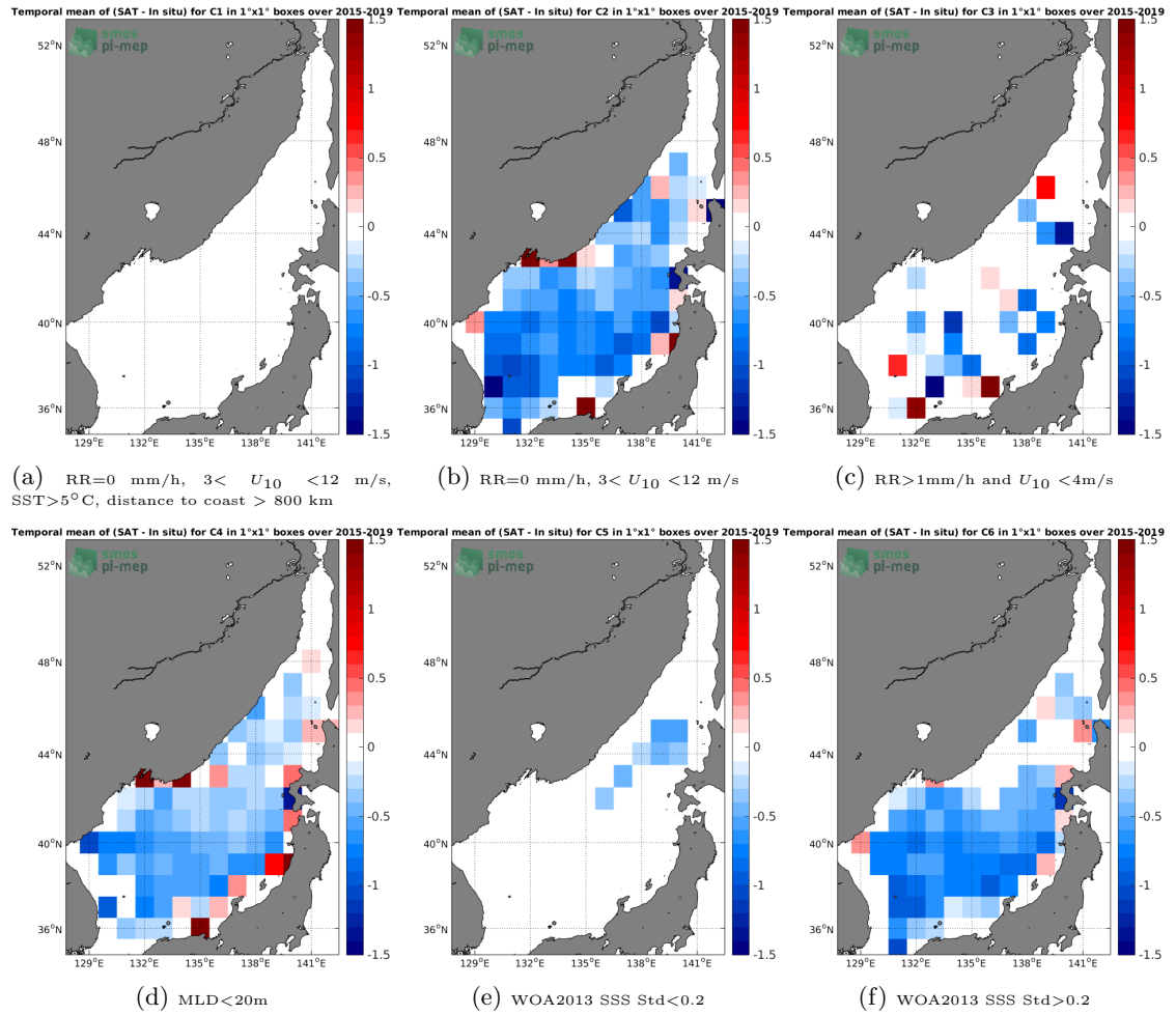
Figure 12: Temporal mean gridded over spatial boxes of size 1^\circ \times 1^\circ of \Delta SSS (SMAP-L3-RSS-V3-8DAY-RUNNING-40KM - Argo) for 6 different subdatasets corresponding to: RR=0 mm/h, 3 < U_{10} < 12 m/s, SST > 5^\circ\text{C} , distance to coast > 800 km (a), RR=0 mm/h, 3 < U_{10} < 12 m/s (b), RR > 1 mm/h and U_{10} < 4 m/s (c), MLD < 20 m (d), WOA2013 SSS Std < 0.2 (e), WOA2013 SSS Std > 0.2 (f).
