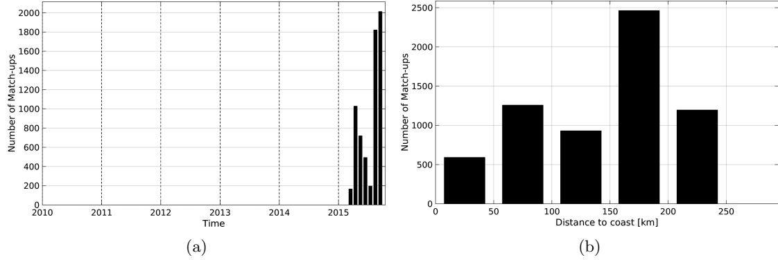
Figure 1: Number of match-ups between TSG-LEGOS-DM and SMAP-L3-RSS-V2-8DAY-RUNNING-70KM SSS as a function of time (a) and as function of the distance to coast (b) over the Sea of Japan Pi-MEP region and for the full satellite product period.
