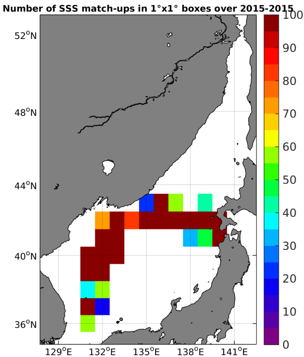
Figure 4: Number of SSS match-ups between TSG-LEGOS-DM SSS and the SMAP-L3-RSS-V2-8DAY-RUNNING-70KM SSS product for the Sea of Japan Pi-MEP region over 1°x1° boxes and for the full satellite product period.
