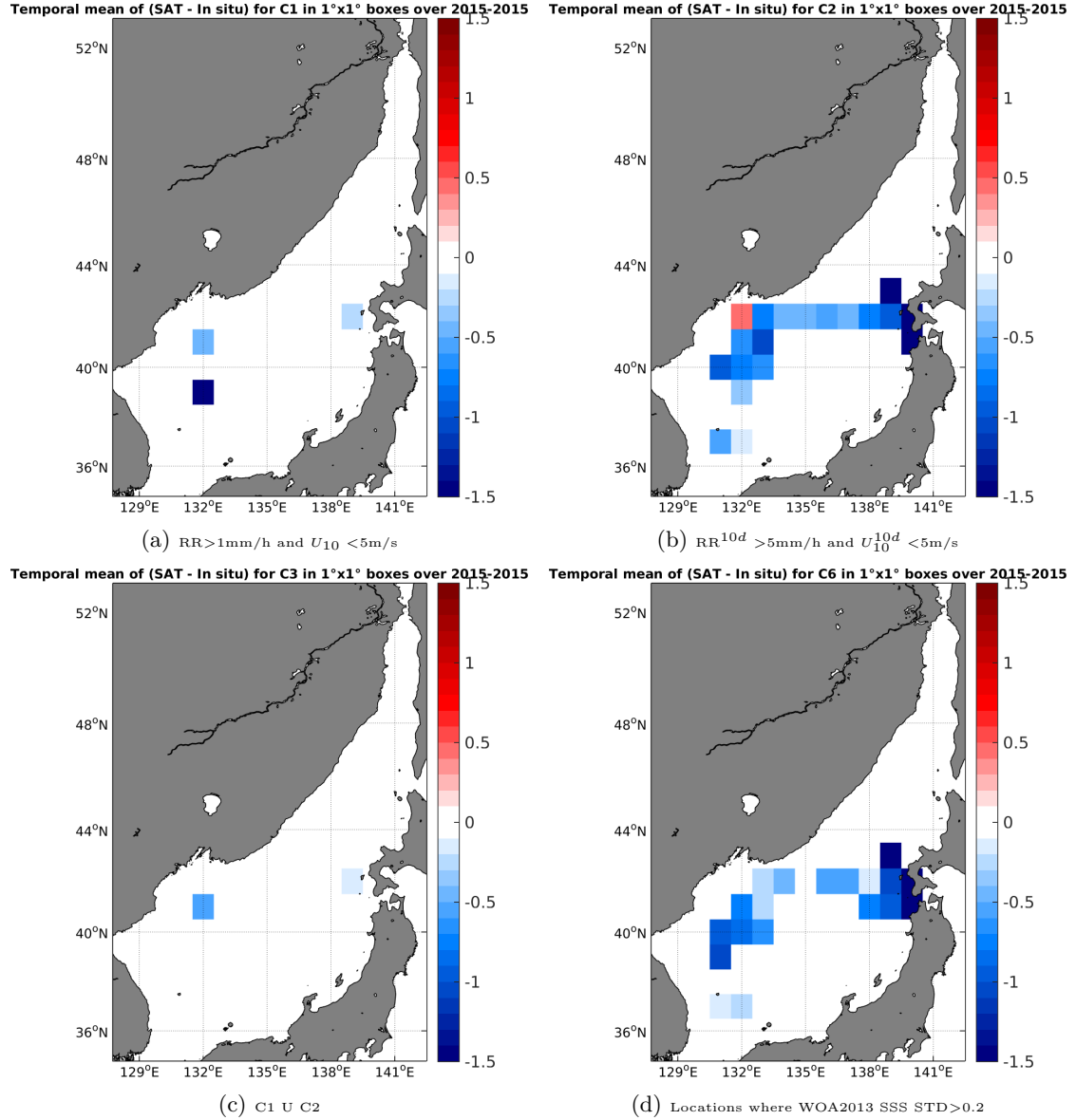
Figure 12: Temporal mean gridded over spatial boxes of size 1^\circ \times 1^\circ of \Delta SSS (SMAP-L3-RSS-V2-8DAY-RUNNING-70KM - TSG-LEGOS-DM) for 4 different subdatasets corresponding to: RR > 1 mm/h and U_{10} < 5 m/s (a), RR 10d > 5 mm/h and U_{10}^{10d} < 5 m/s (b), C1 U C2 (c), Locations where WOA2013 SSS STD > 0.2 (d).
