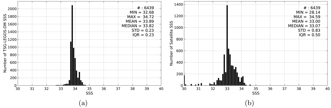
Figure 2: Histograms of SSS from TSG-LEGOS-DM (a) and SMAP-L3-RSS-V2-8DAY-RUNNING-70KM (b) considering all match-up pairs per bins of 0.1 over the Sea of Japan Pi-MEP region and for the full satellite product period.
