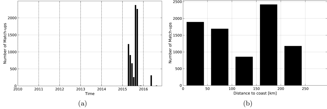
Figure 1: Number of match-ups between TSG-LEGOS-DM and SMAP-L3-RSS-V2-MONTHLY-0.25DEG-40KM SSS as a function of time (a) and as function of the distance to coast (b) over the Sea of Japan Pi-MEP region and for the full satellite product period.
