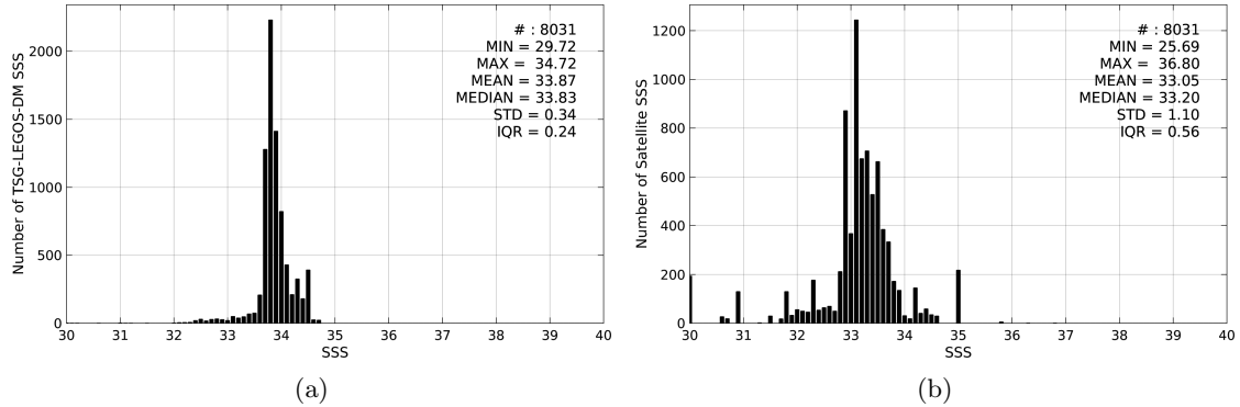
Figure 2: Histograms of SSS from TSG-LEGOS-DM (a) and SMAP-L3-RSS-V2-MONTHLY-0.25DEG-40KM (b) considering all match-up pairs per bins of 0.1 over the Sea of Japan Pi-MEP region and for the full satellite product period.
