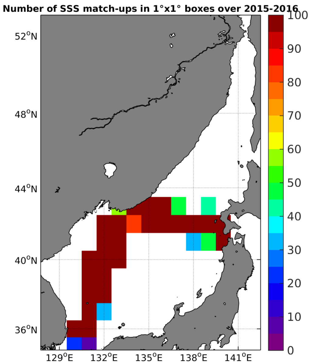
Figure 4: Number of SSS match-ups between TSG-LEGOS-DM SSS and the SMAP-L3-RSS-V2-MONTHLY-0.25DEG-40KM SSS product for the Sea of Japan Pi-MEP region over 1°x1° boxes and for the full satellite product period.
