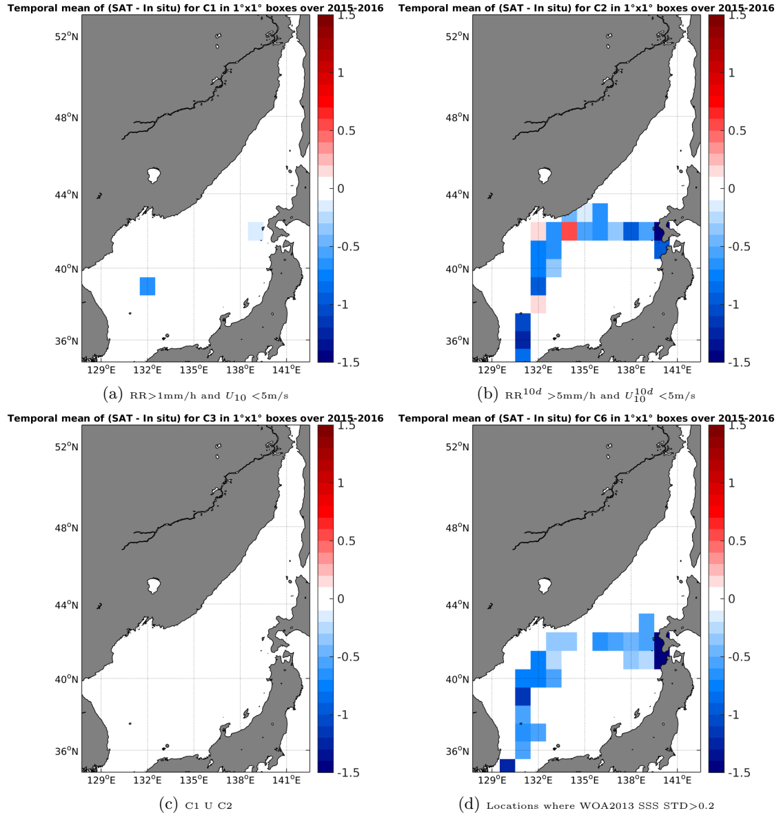
Figure 12: Temporal mean gridded over spatial boxes of size 1^\circ \times 1^\circ of \Delta SSS (SMAP-L3-RSS-V2-MONTHLY-0.25DEG-40KM - TSG-LEGOS-DM) for 4 different subdatasets corresponding to: RR>1mm/h and U_{10} < 5 m/s (a), RR^{10d} > 5 mm/h and U_{10}^{10d} < 5 m/s (b), C1 U C2 (c), Locations where WOA2013 SSS STD>0.2 (d).
