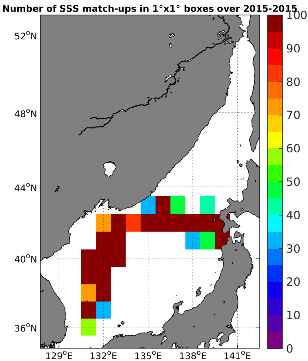
Figure 4: Number of SSS match-ups between TSG-LEGOS-DM SSS and the SMAP-L3-RSS-V2-MONTHLY-70KM SSS product for the Sea of Japan Pi-MEP region over 1°x1° boxes and for the full satellite product period.
