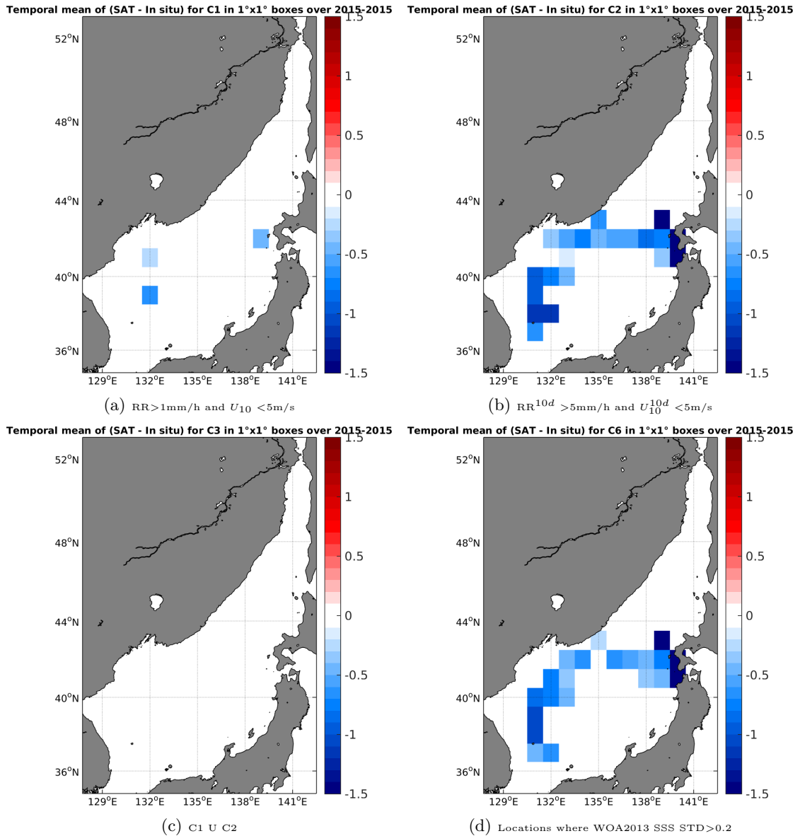
Figure 12: Temporal mean gridded over spatial boxes of size 1°x1° of \Delta SSS (SMAP-L3-RSS-V2-MONTHLY-70KM - TSG-LEGOS-DM) for 4 different subdatasets corresponding to: RR > 1\text{mm/h} and U_{10} < 5\text{m/s} (a), RR^{10d} > 5\text{mm/h} and U_{10}^{10d} < 5\text{m/s} (b), C1 U C2 (c), Locations where WOA2013 SSS STD > 0.2 (d).
