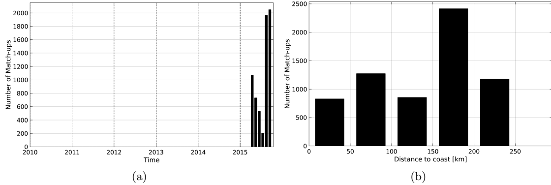
Figure 1: Number of match-ups between TSG-LEGOS-DM and SMAP-L3-RSS-V2-MONTHLY-70KM SSS as a function of time (a) and as function of the distance to coast (b) over the Sea of Japan Pi-MEP region and for the full satellite product period.
