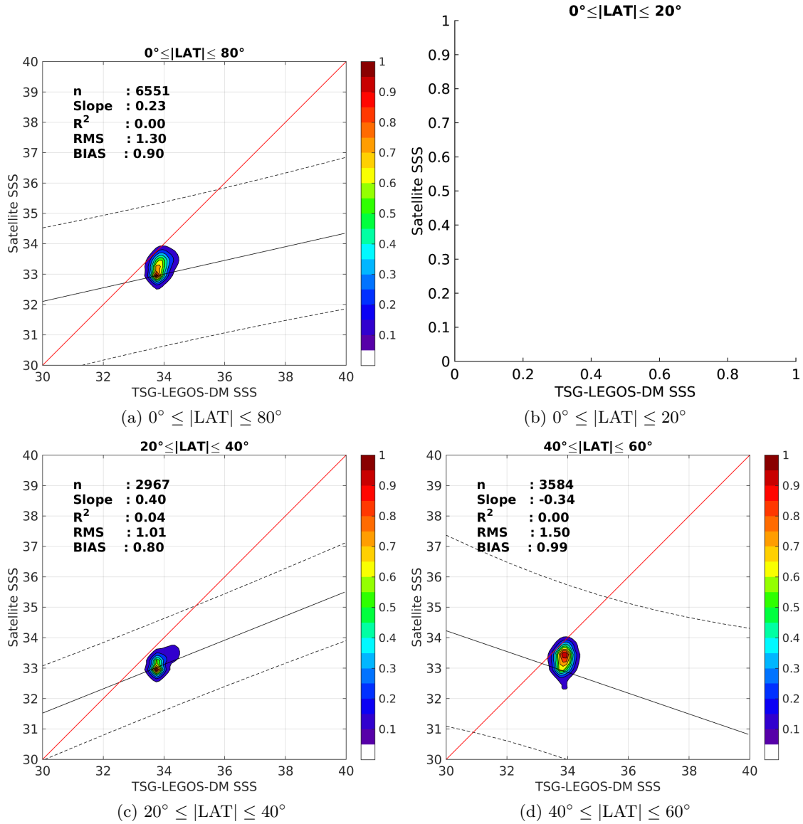
Figure 9: Contour maps of the concentration of SMAP-L3-RSS-V2-MONTHLY-70KM SSS (y-axis) versus TSG-LEGOS-DM SSS (x-axis) at match-up pairs for different latitude bands. For each plot, the red line shows x=y . The black thin and dashed lines indicate a linear fit through the data cloud and the \pm 95\% confidence levels, respectively. The number match-up pairs n , the slope and R^2 coefficient of the linear fit, the root mean square (RMS) and the mean bias between satellite and in situ data are indicated for each latitude band in each plots.
