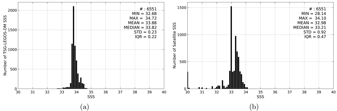
Figure 2: Histograms of SSS from TSG-LEGOS-DM (a) and SMAP-L3-RSS-V2-MONTHLY-70KM (b) considering all match-up pairs per bins of 0.1 over the Sea of Japan Pi-MEP region and for the full satellite product period.
