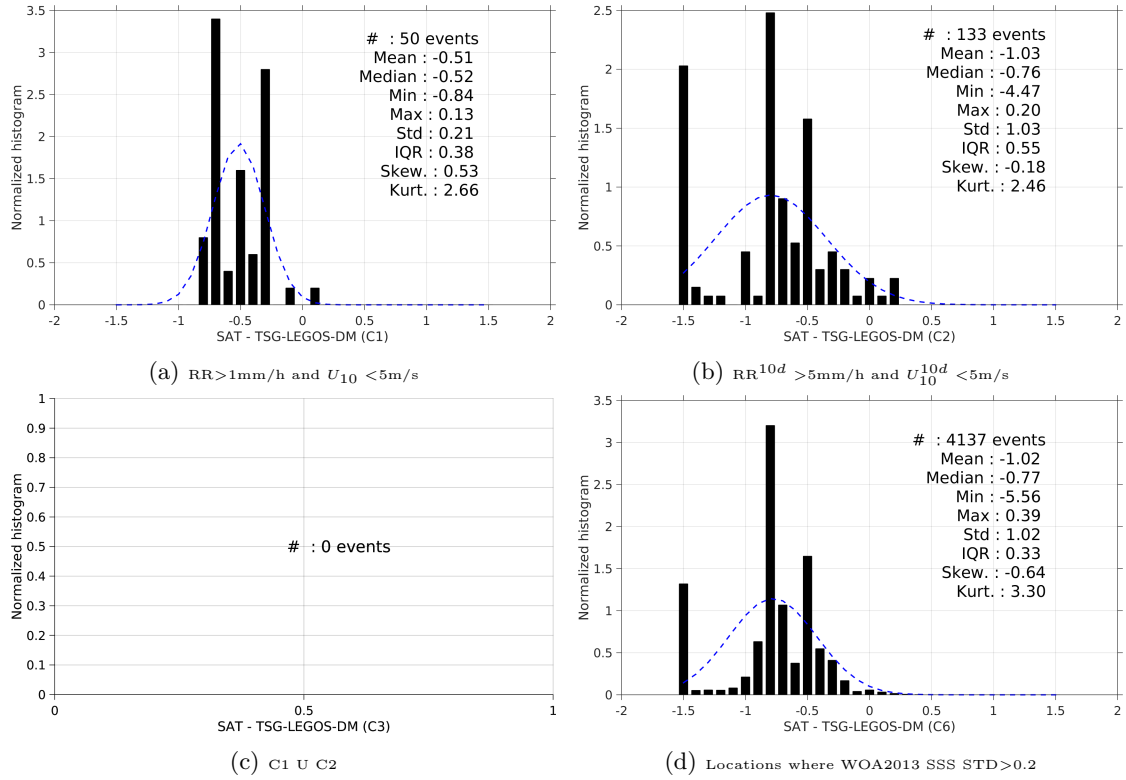
Figure 13: Normalized histogram of \Delta\text{SSS} (SMAP-L3-RSS-V2-MONTHLY-70KM - TSG-LEGOS-DM) for 6 different subdatasets corresponding to: RR > 1mm/h and U_{10} < 5\text{m/s} (a), RR^{10d} > 5\text{mm/h} and U_{10}^{10d} < 5\text{m/s} (b), C1 U C2 (c), Locations where WOA2013 SSS STD > 0.2 (d).
