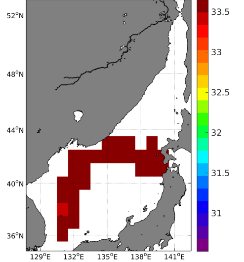
(c) MEAN(TSG-LEGOS-DM SSS)
