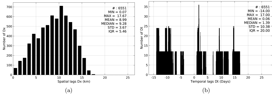
Figure 5: Histograms of the spatial (a) and temporal (b) lags between the time of the TSG-LEGOS-DM measurements and the date of the corresponding SMAP-L3-RSS-V2-MONTHLY-70KM SSS product.
