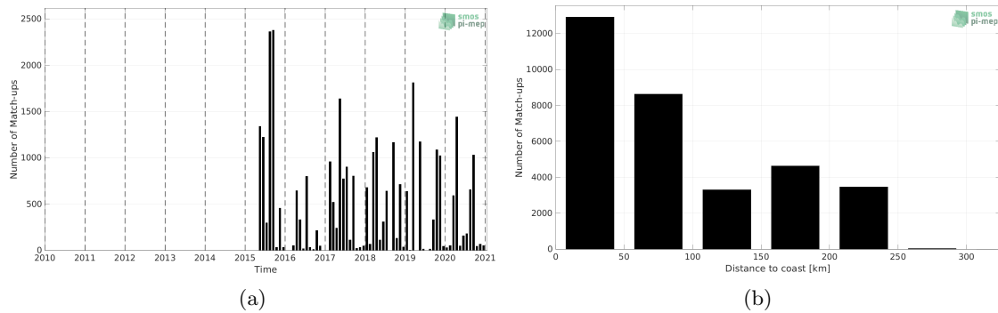
Figure 1: Number of match-ups between TSG (LEGOS-DM) and SMAP SSS L3 v5.0 - 8-Day running (JPL) SSS as a function of time (a) and as function of the distance to coast (b) over the Sea of Japan Pi-MEP region and for the full satellite product period.
