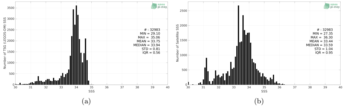
Figure 2: Histograms of SSS from TSG (LEGOS-DM) (a) and SMAP SSS L3 v5.0 - 8-Day running (JPL) (b) considering all match-up pairs per bins of 0.1 over the Sea of Japan Pi-MEP region and for the full satellite product period.
