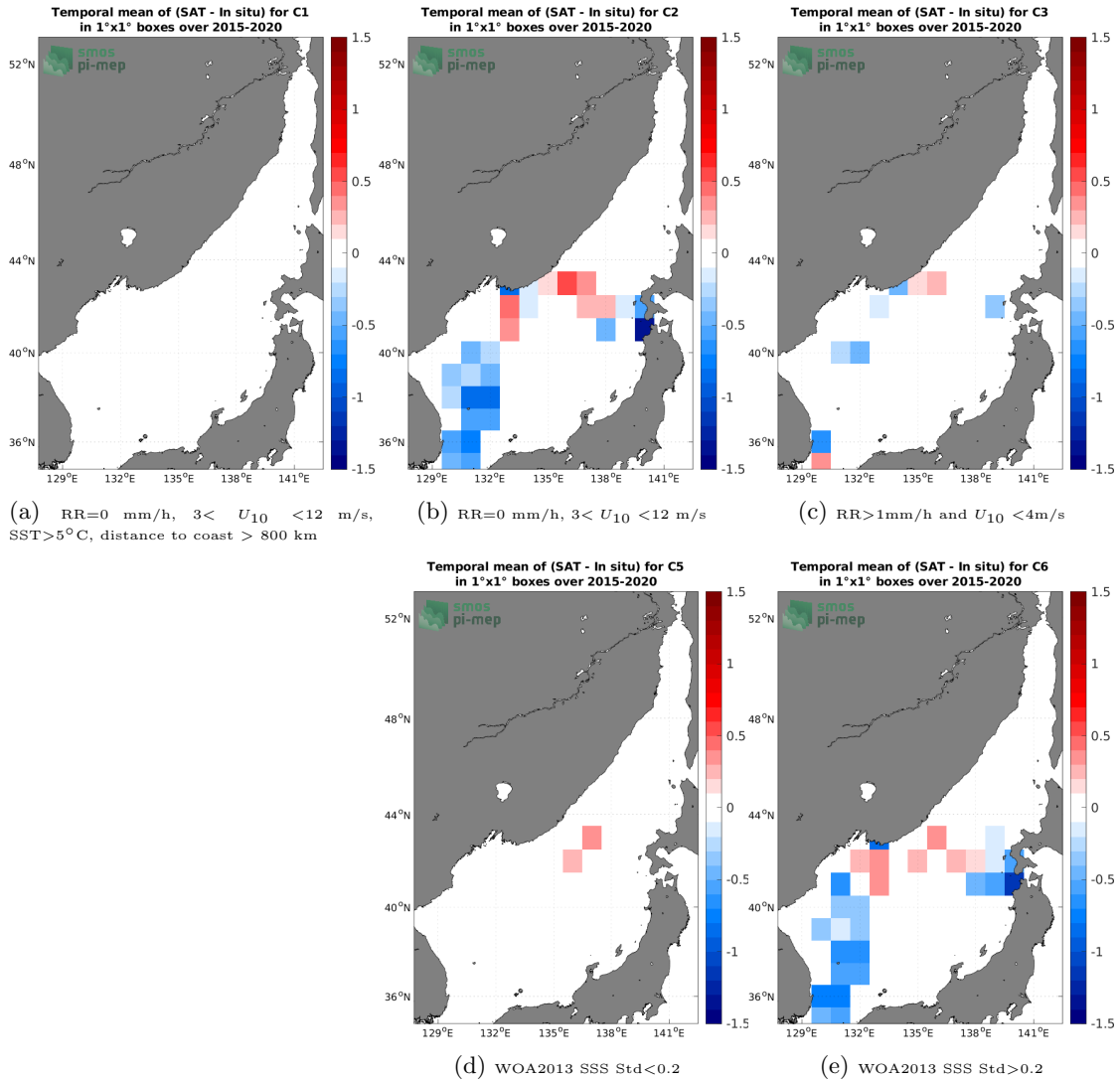
Figure 12: Temporal mean gridded over spatial boxes of size 1^\circ \times 1^\circ of \Delta\text{SSS} (SMAP SSS L3 v5.0 - 8-Day running (JPL) - TSG (LEGOS-DM)) for 5 different subdatasets corresponding to: RR=0 mm/h, 3 < U_{10} < 12 m/s, SST > 5^\circ\text{C} , distance to coast > 800 km (a), RR=0 mm/h, 3 < U_{10} < 12 m/s (b), RR > 1 mm/h and U_{10} < 4 m/s (c), WOA2013 SSS Std < 0.2 (d), WOA2013 SSS Std > 0.2 (e).
