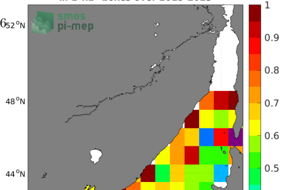
Temporal STD of (Sat - Argo) in 1°x1° boxes over 2015-2023
