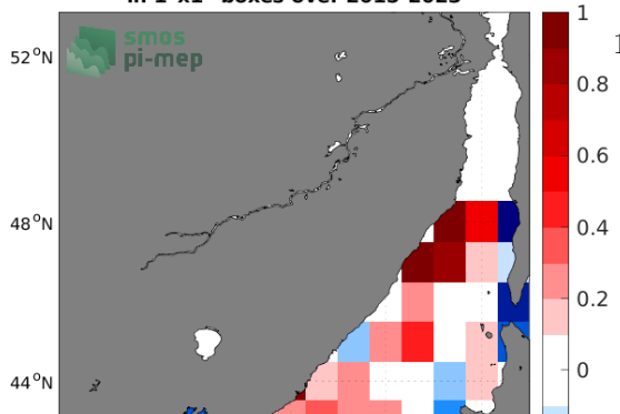
Temporal mean of (Sat - Argo) in 1°x1° boxes over 2015-2023
