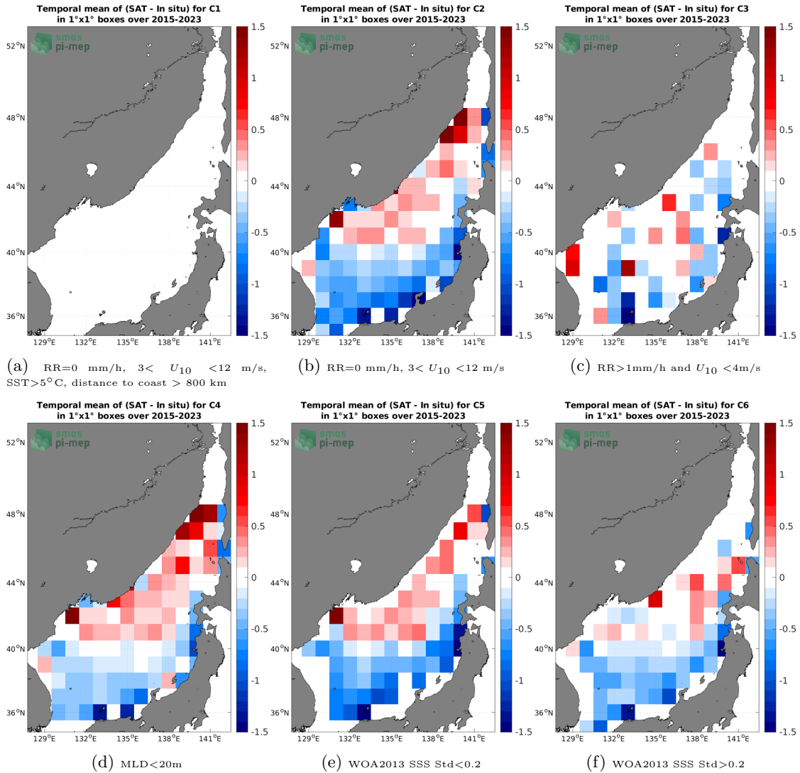
Figure 12: Temporal mean gridded over spatial boxes of size 1^\circ \times 1^\circ of \Delta SSS (SMAP SSS L3 v5.0 - 8-Day running (JPL) - Argo) for 6 different subdatasets corresponding to: RR=0 mm/h, 3 < U_{10} < 12 m/s, SST > 5^\circ C , distance to coast > 800 km (a), RR=0 mm/h, 3 < U_{10} < 12 m/s (b), RR > 1 mm/h and U_{10} < 4 m/s (c), MLD < 20 m (d), WOA2013 SSS Std < 0.2 (e), WOA2013 SSS Std > 0.2 (f).
