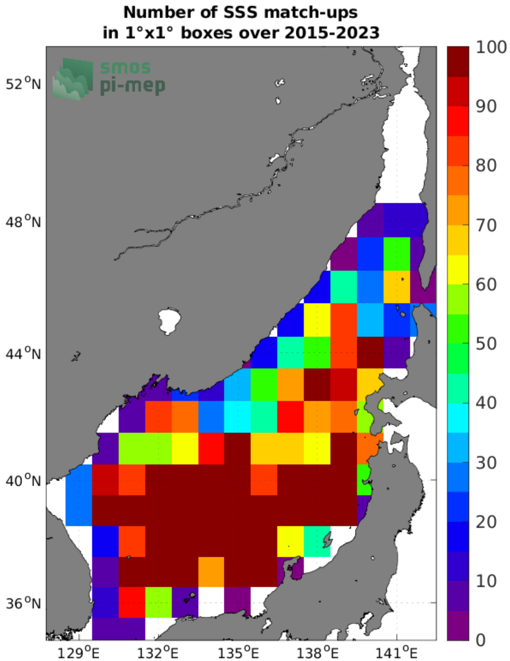
Figure 4: Number of SSS match-ups between Argo SSS and the SMAP SSS L3 v5.0 - 8-Day running (JPL) SSS product for the Sea of Japan Pi-MEP region over 1°x1° boxes and for the full satellite product period.
