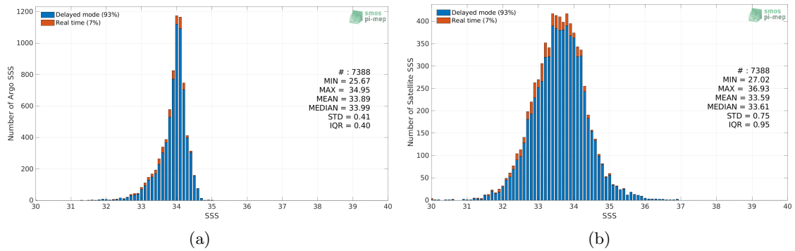
Figure 2: Histograms of SSS from Argo (a) and SMAP SSS L3 v5.0 - 8-Day running (JPL) (b) considering all match-up pairs per bins of 0.1 over the Sea of Japan Pi-MEP region and for the full satellite product period.
