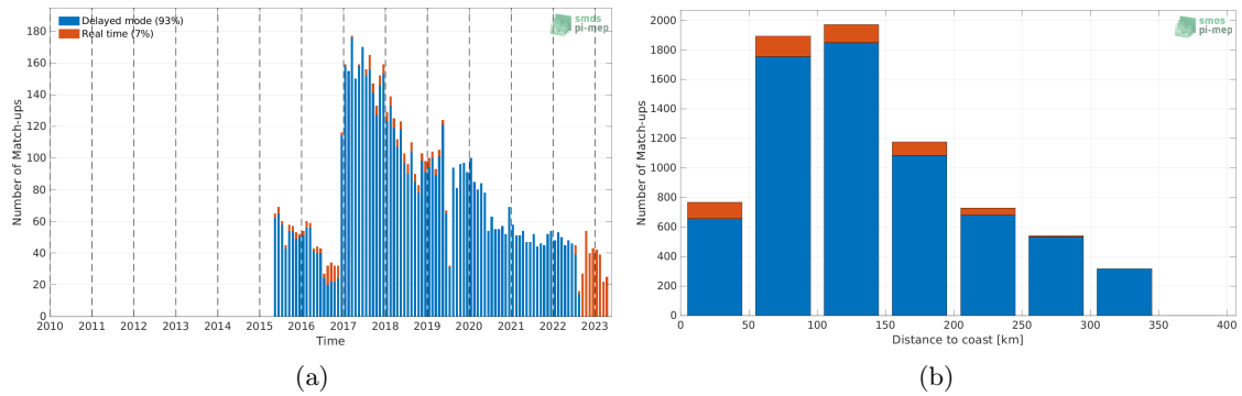
Figure 1: Number of match-ups between Argo and SMAP SSS L3 v5.0 - 8-Day running (JPL) SSS as a function of time (a) and as function of the distance to coast (b) over the Sea of Japan Pi-MEP region and for the full satellite product period.
