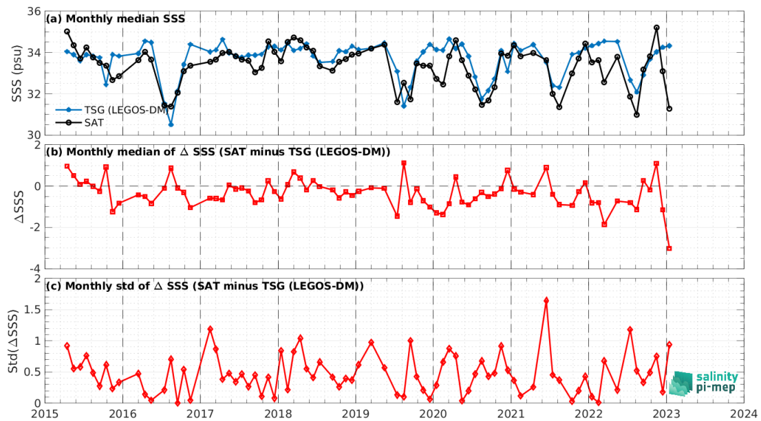
Figure 8: Time series of the monthly median SSS (top), median of \Delta SSS (Satellite - TSG (LEGOS-DM)) and Std of \Delta SSS (Satellite - TSG (LEGOS-DM)) over the Sea of Japan Pi-MEP region considering all match-ups collected by the Pi-MEP.
