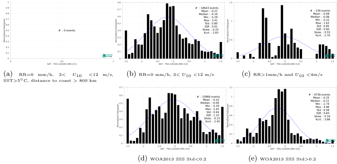
Figure 15: Normalized histogram of \Delta SSS (SMAP SSS L3 v5.0 - Monthly (JPL) - TSG (LEGOS-DM)) for 5 different subdatasets corresponding to: RR=0 mm/h, 3 < U_{10} < 12 m/s, SST > 5°C, distance to coast > 800 km (a), RR=0 mm/h, 3 < U_{10} < 12 m/s (b), RR > 1mm/h and U_{10} < 4 m/s (c), WOA2013 SSS Std < 0.2 (d), WOA2013 SSS Std > 0.2 (e).
