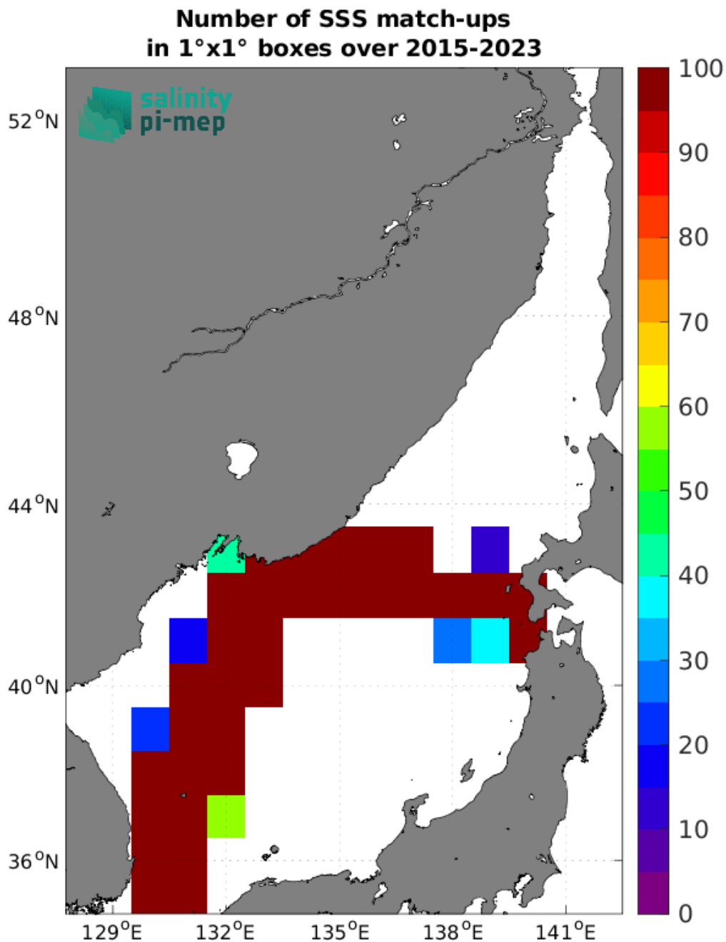
Figure 5: Number of SSS match-ups between TSG (LEGOS-DM) SSS and the SMAP SSS L3 v5.0 - Monthly (JPL) SSS product for the Sea of Japan Pi-MEP region over 1°x1° boxes and for the full satellite product period.
