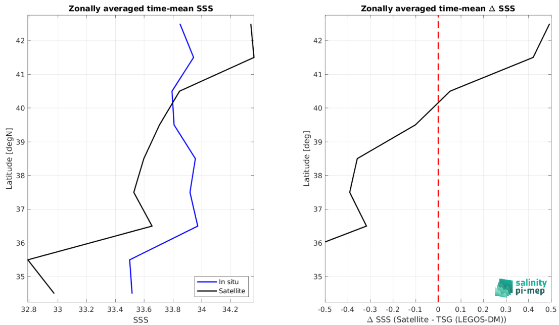
Figure 9: Left panel: Zonal mean SSS from SMAP SSS L3 v5.0 - Monthly (JPL) satellite product (black) and from TSG (LEGOS-DM) (blue). Right panel: Zonal mean of \Delta SSS (Satellite - TSG (LEGOS-DM)) for all the collected Pi-MEP match-up pairs estimated over the full satellite product period.
