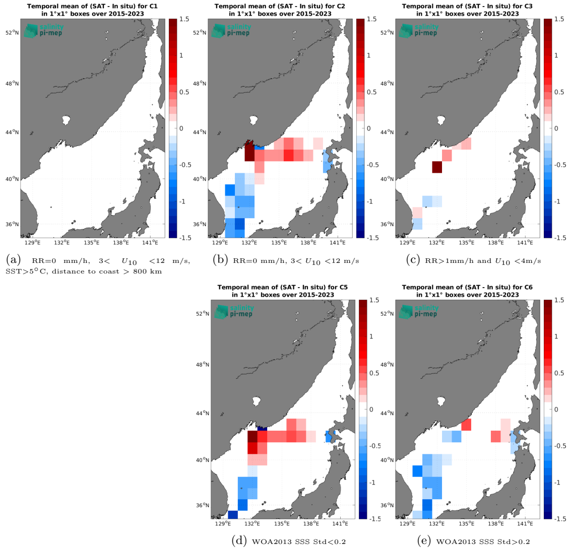
Figure 14: Temporal mean gridded over spatial boxes of size 1^\circ \times 1^\circ of \Delta SSS (SMAP SSS L3 v5.0 - Monthly (JPL) - TSG (LEGOS-DM)) for 5 different subdatasets corresponding to:RR=0 mm/h, 3 < U_{10} < 12 m/s, SST>5°C, distance to coast > 800 km (a), RR=0 mm/h, 3 < U_{10} < 12 m/s (b), RR>1mm/h and U_{10} < 4 m/s (c), WOA2013 SSS Std<0.2 (d), WOA2013 SSS Std>0.2 (e).
