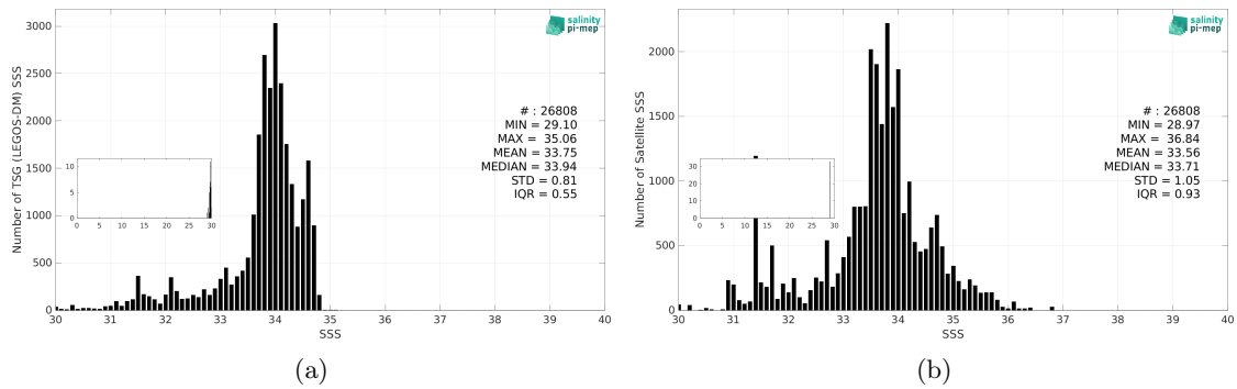
Figure 3: Histograms of SSS from TSG (LEGOS-DM) (a) and SMAP SSS L3 v5.0 - Monthly (JPL) (b) considering all match-up pairs per bins of 0.1 over the Sea of Japan Pi-MEP region and for the full satellite product period.
