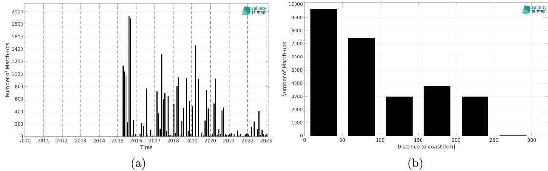
Figure 2: Number of match-ups between TSG (LEGOS-DM) and SMAP SSS L3 v5.0 - Monthly (JPL) SSS as a function of time (a) and as function of the distance to coast (b) over the Sea of Japan Pi-MEP region and for the full satellite product period.
