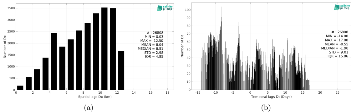
Figure 6: Histograms of the spatial (a) and temporal (b) lags between the location/time of the TSG (LEGOS-DM) measurement and the date of the corresponding SMAP SSS L3 v5.0 - Monthly (JPL) SSS pixel.
