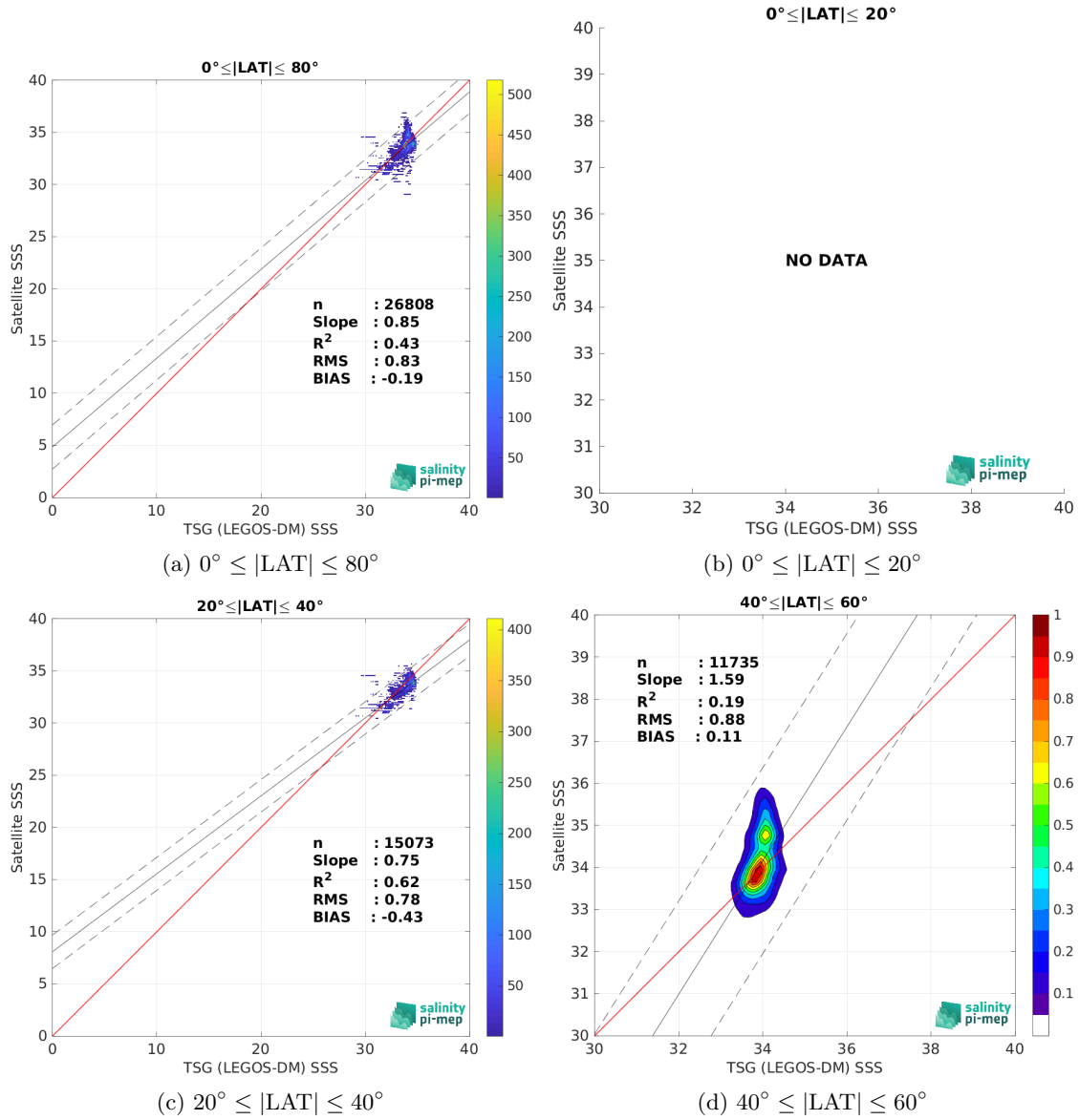
Figure 10: Contour maps of the concentration of SMAP SSS L3 v5.0 - Monthly (JPL) SSS (y-axis) versus TSG (LEGOS-DM) SSS (x-axis) at match-up pairs for different latitude bands. For each plot, the red line shows x=y . The black thin and dashed lines indicate a linear fit through the data cloud and the \pm 95\% confidence levels, respectively. The number match-up pairs n , the slope and R^2 coefficient of the linear fit, the root mean square (RMS) and the mean bias between satellite and in situ data are indicated for each latitude band in each plots.
