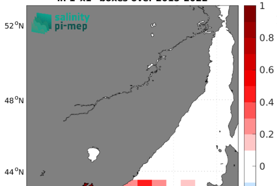
Temporal mean of (Sat - TSG (LEGOS-DM)) in 1°x1° boxes over 2015-2022
