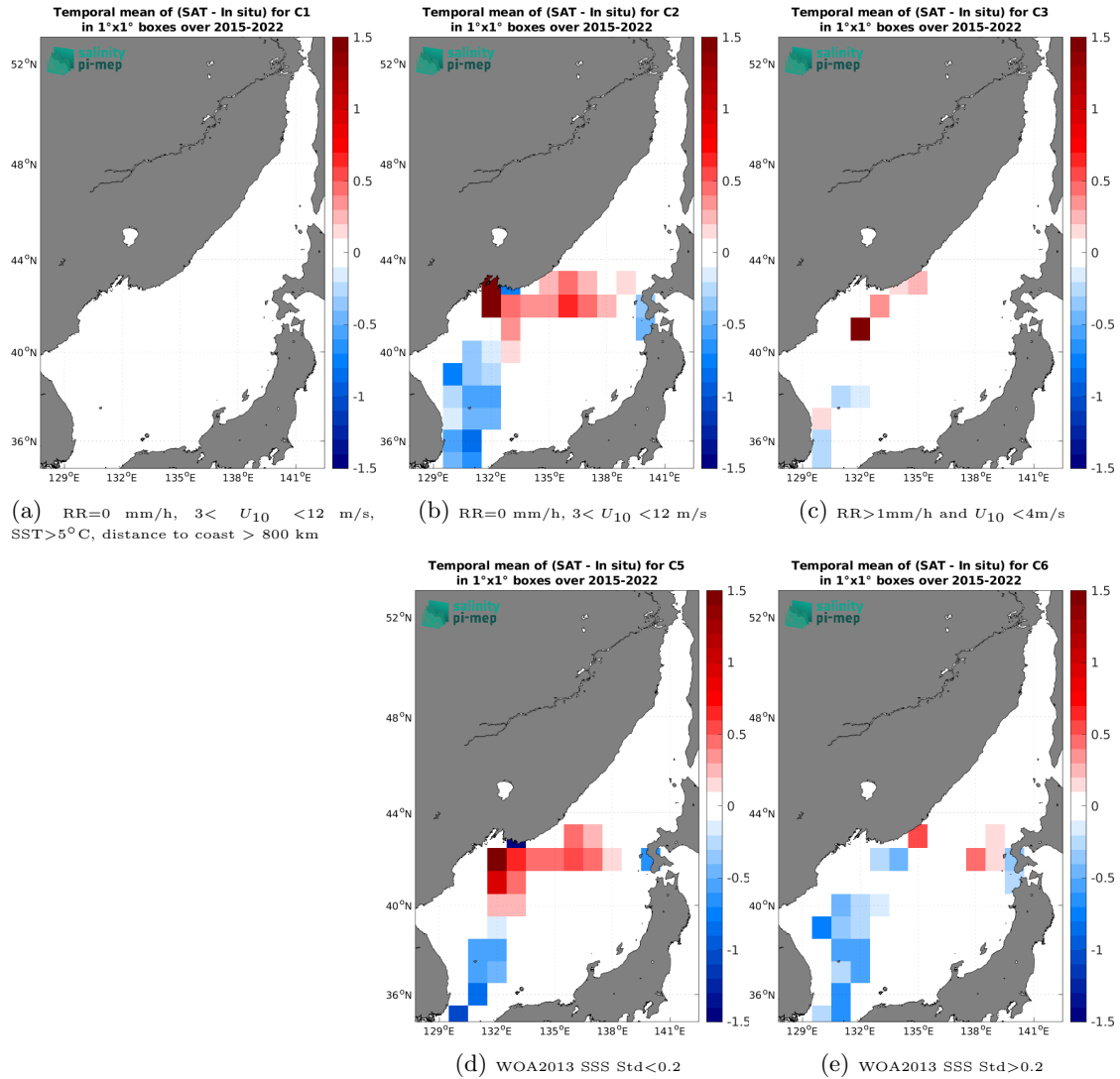
Figure 14: Temporal mean gridded over spatial boxes of size 1^\circ \times 1^\circ of \Delta\text{SSS} (SMAP SSS L3 v5.0 - Monthly (JPL) - TSG (LEGOS-DM)) for 5 different subdatasets corresponding to: RR=0 mm/h, 3 < U_{10} < 12 m/s, SST > 5^\circ\text{C} , distance to coast > 800 km (a), RR=0 mm/h, 3 < U_{10} < 12 m/s (b), RR > 1 mm/h and U_{10} < 4 m/s (c), WOA2013 SSS Std < 0.2 (d), WOA2013 SSS Std > 0.2 (e).
