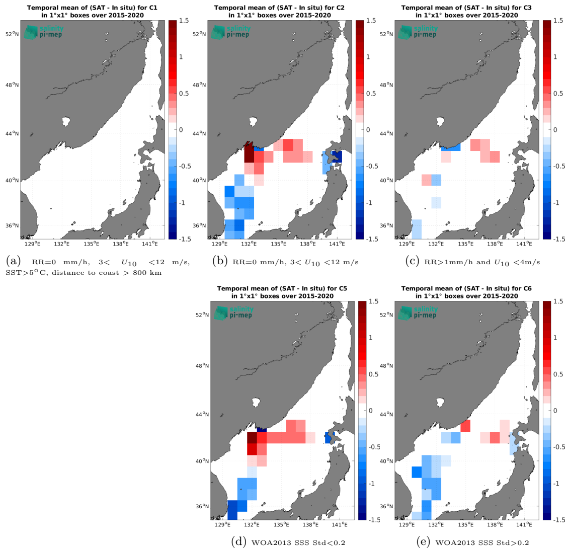
Figure 12: Temporal mean gridded over spatial boxes of size 1^\circ \times 1^\circ of \Delta\text{SSS} (SMAP SSS L3 v5.0 - Monthly (JPL) - TSG (LEGOS-DM)) for 5 different subdatasets corresponding to: RR=0 mm/h, 3 < U_{10} < 12 m/s, SST > 5^\circ\text{C} , distance to coast > 800 km (a), RR=0 mm/h, 3 < U_{10} < 12 m/s (b), RR > 1 mm/h and U_{10} < 4 m/s (c), WOA2013 SSS Std < 0.2 (d), WOA2013 SSS Std > 0.2 (e).
