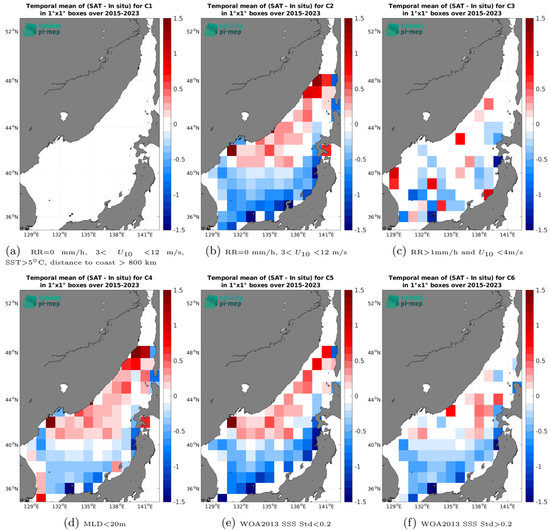
Figure 12: Temporal mean gridded over spatial boxes of size 1^\circ \times 1^\circ of \Delta SSS (SMAP SSS L3 v5.0 - Monthly (JPL) - Argo) for 6 different subdatasets corresponding to: RR=0 mm/h, 3 < U_{10} < 12 m/s, SST > 5°C, distance to coast > 800 km (a), RR=0 mm/h, 3 < U_{10} < 12 m/s (b), RR > 1mm/h and U_{10} < 4 m/s (c), MLD < 20m (d), WOA2013 SSS Std < 0.2 (e), WOA2013 SSS Std > 0.2 (f).
