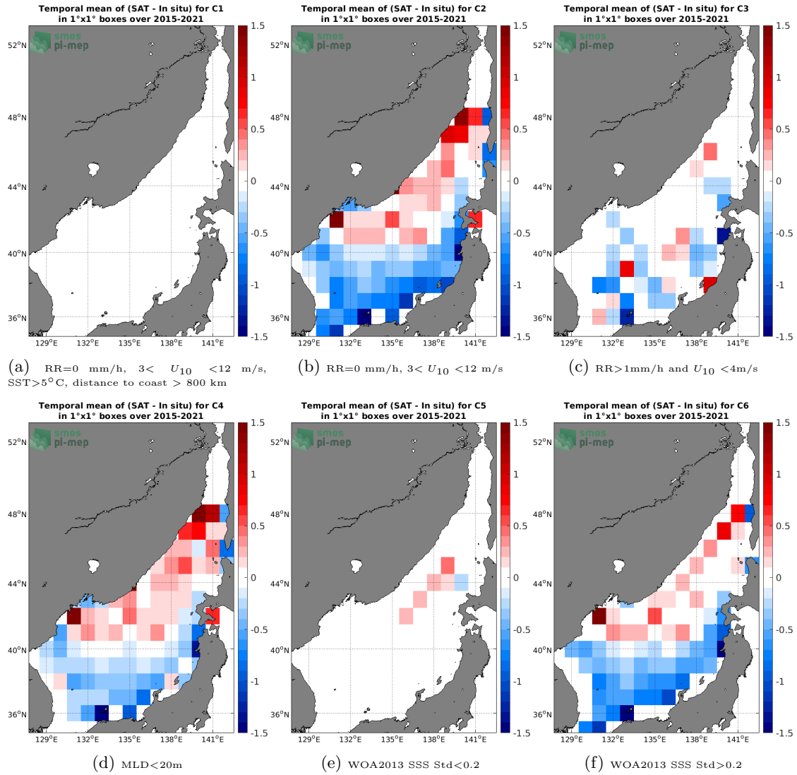
Figure 12: Temporal mean gridded over spatial boxes of size 1°x1° of \Delta SSS (SMAP SSS L3 v5.0 - Monthly (JPL) - Argo) for 6 different subdatasets corresponding to:RR=0 mm/h, 3 < U_{10} < 12 m/s, SST>5°C, distance to coast > 800 km (a), RR=0 mm/h, 3 < U_{10} < 12 m/s (b), RR>1mm/h and U_{10} < 4 m/s (c),MLD<20m (d),WOA2013 SSS Std<0.2 (e),WOA2013 SSS Std>0.2 (f).
