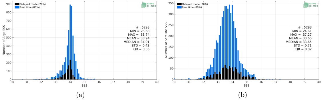
Figure 2: Histograms of SSS from Argo (a) and SMAP SSS L3 v5.0 - Monthly (JPL) (b) considering all match-up pairs per bins of 0.1 over the Sea of Japan Pi-MEP region and for the full satellite product period.
