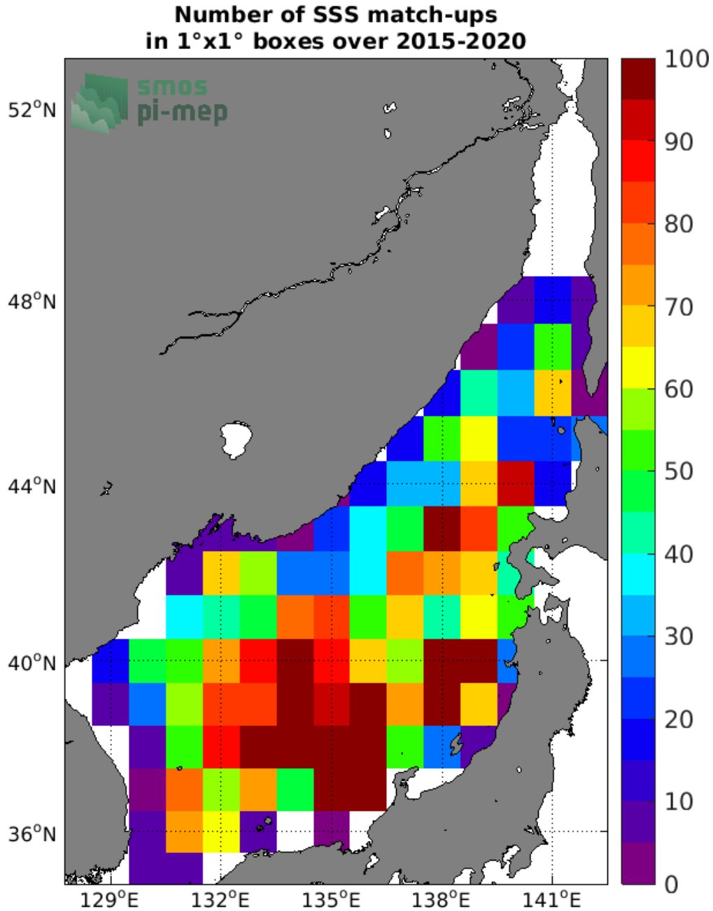
Figure 4: Number of SSS match-ups between Argo SSS and the SMAP SSS L3 v5.0 - Monthly (JPL) SSS product for the Sea of Japan Pi-MEP region over 1°x1° boxes and for the full satellite product period.
