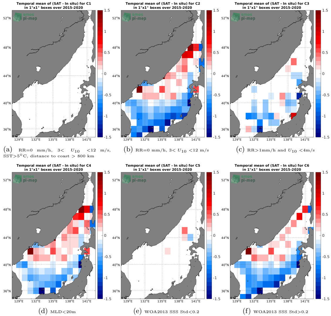
Figure 12: Temporal mean gridded over spatial boxes of size 1°x1° of \Delta SSS (SMAP SSS L3 v5.0 - Monthly (JPL) - Argo) for 6 different subdatasets corresponding to: RR=0 mm/h, 3 < U_{10} < 12 m/s, SST > 5^\circ\text{C} , distance to coast > 800 km (a), RR=0 mm/h, 3 < U_{10} < 12 m/s (b), RR > 1 mm/h and U_{10} < 4 m/s (c), MLD < 20 m (d), WOA2013 SSS Std < 0.2 (e), WOA2013 SSS Std > 0.2 (f).
