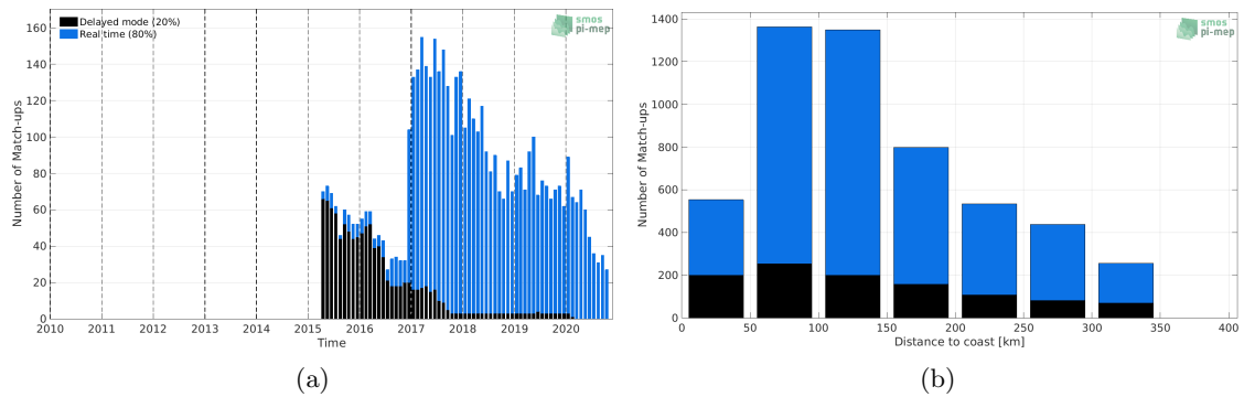
Figure 1: Number of match-ups between Argo and SMAP SSS L3 v5.0 - Monthly (JPL) SSS as a function of time (a) and as function of the distance to coast (b) over the Sea of Japan Pi-MEP region and for the full satellite product period.
